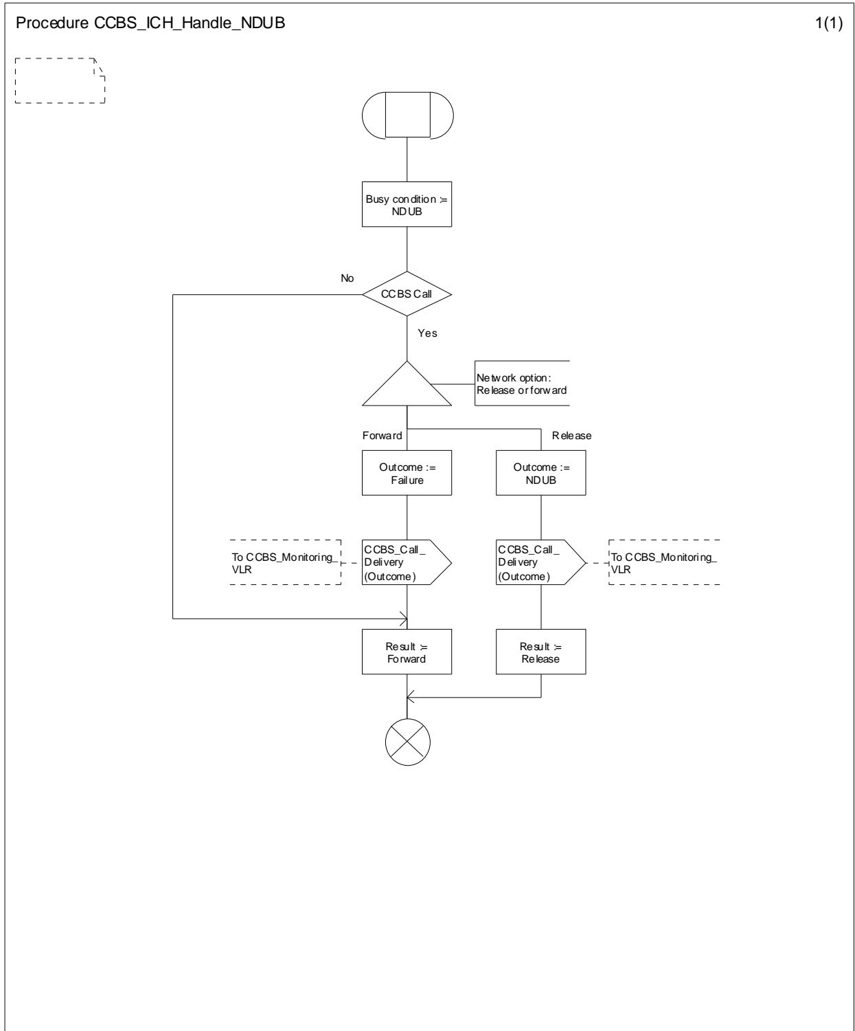
Figure 11.2.3.7: Procedure CCBS_ICH_Handle_NDUB
