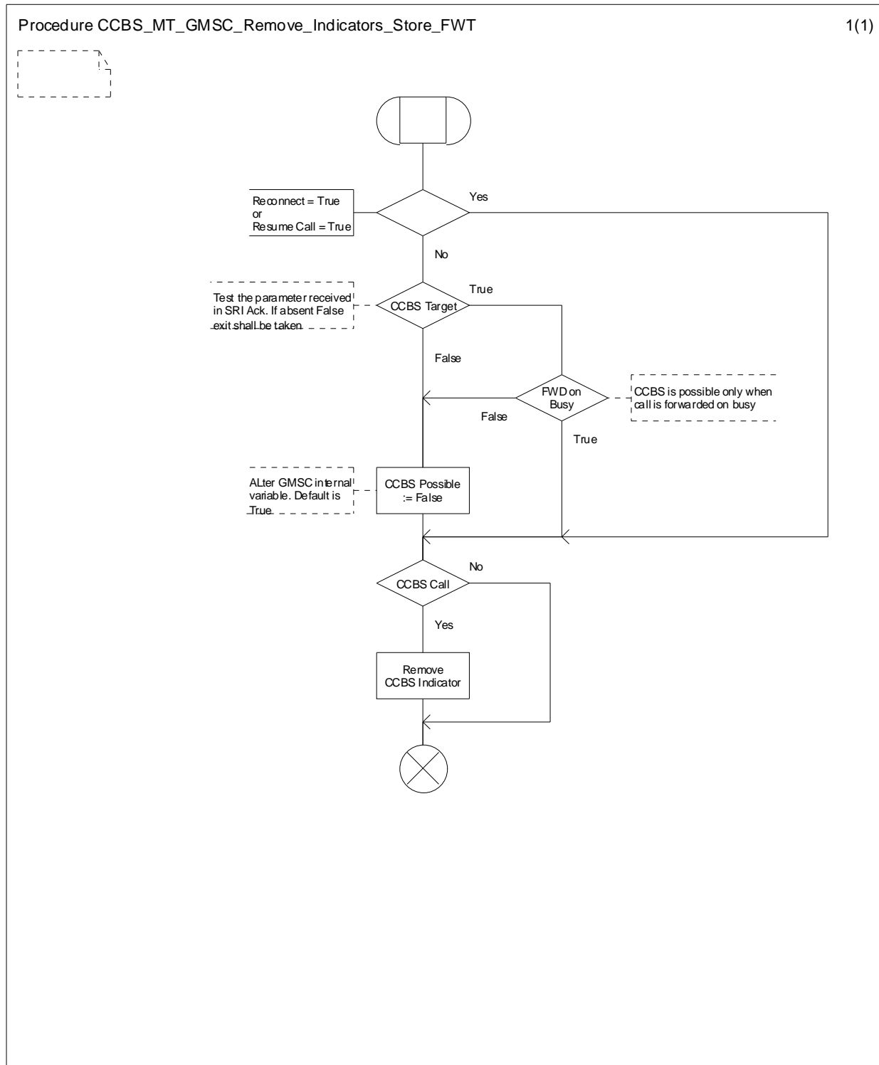
Figure 11.2.1.3: Procedure CCBS_MT_GMSC_Remove_Indicators_Store_FWT
