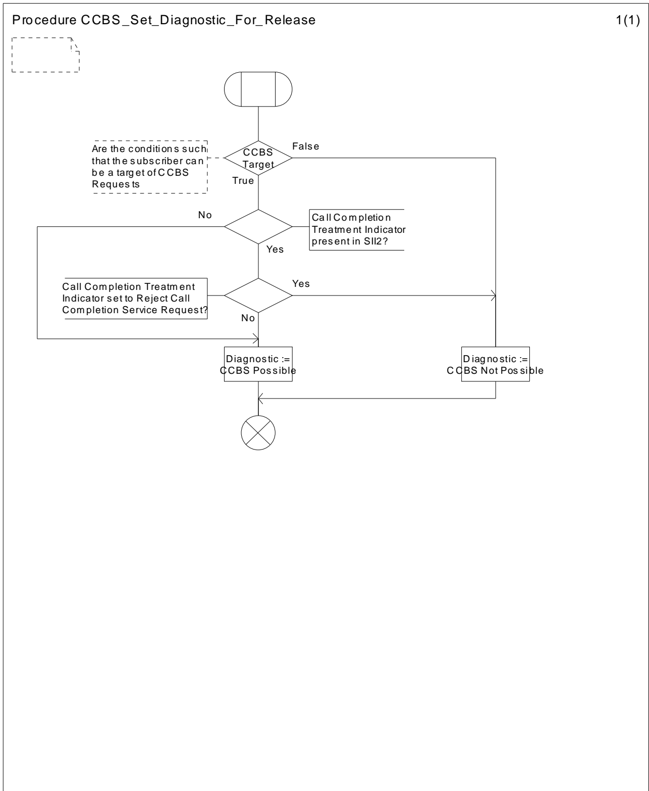
Figure 11.3.4: Procedure CCBS_Set_Diagnostic_For_Release
