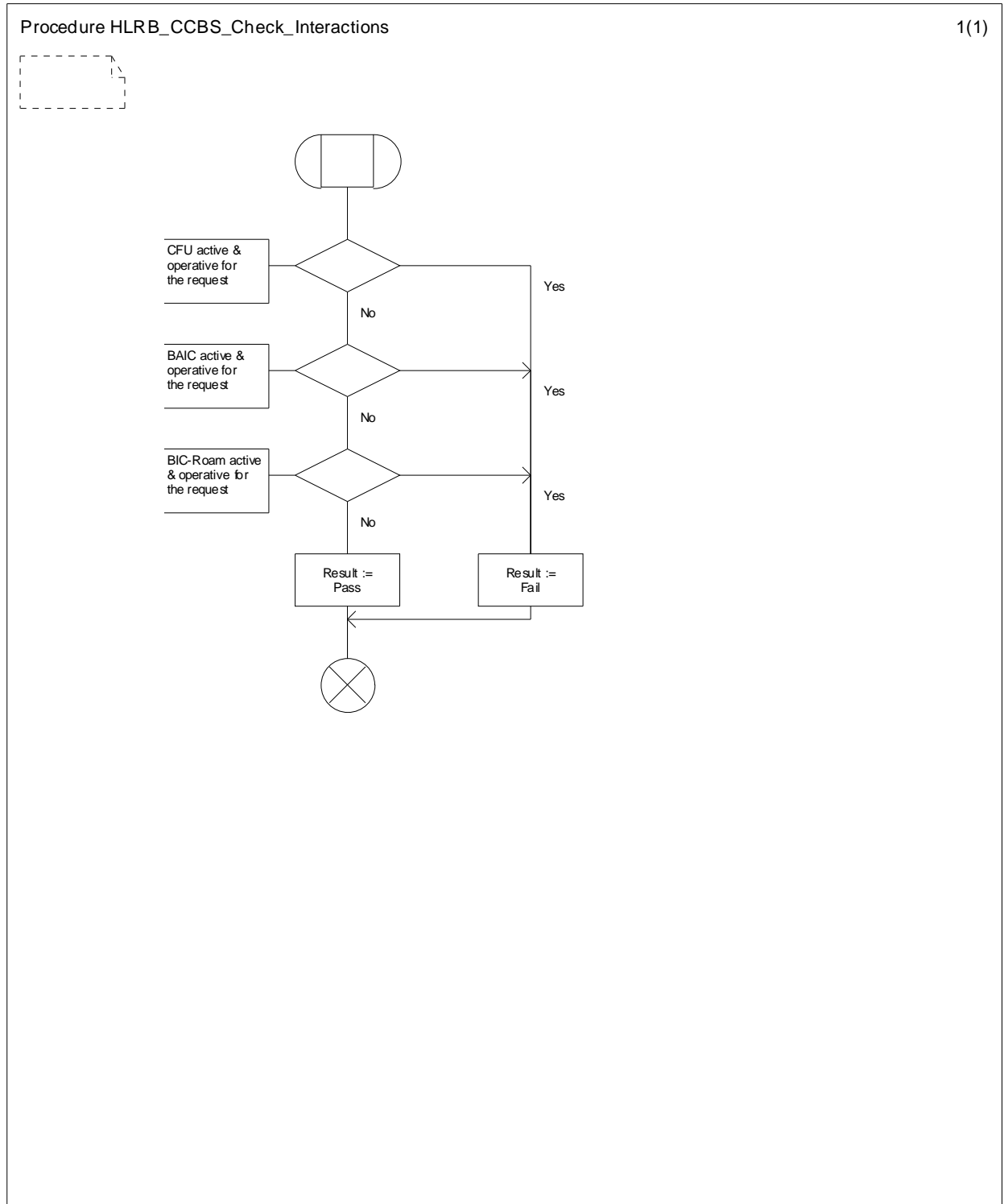
Figure 11.2.2.7: Procedure HLRB_Check_Interactions
