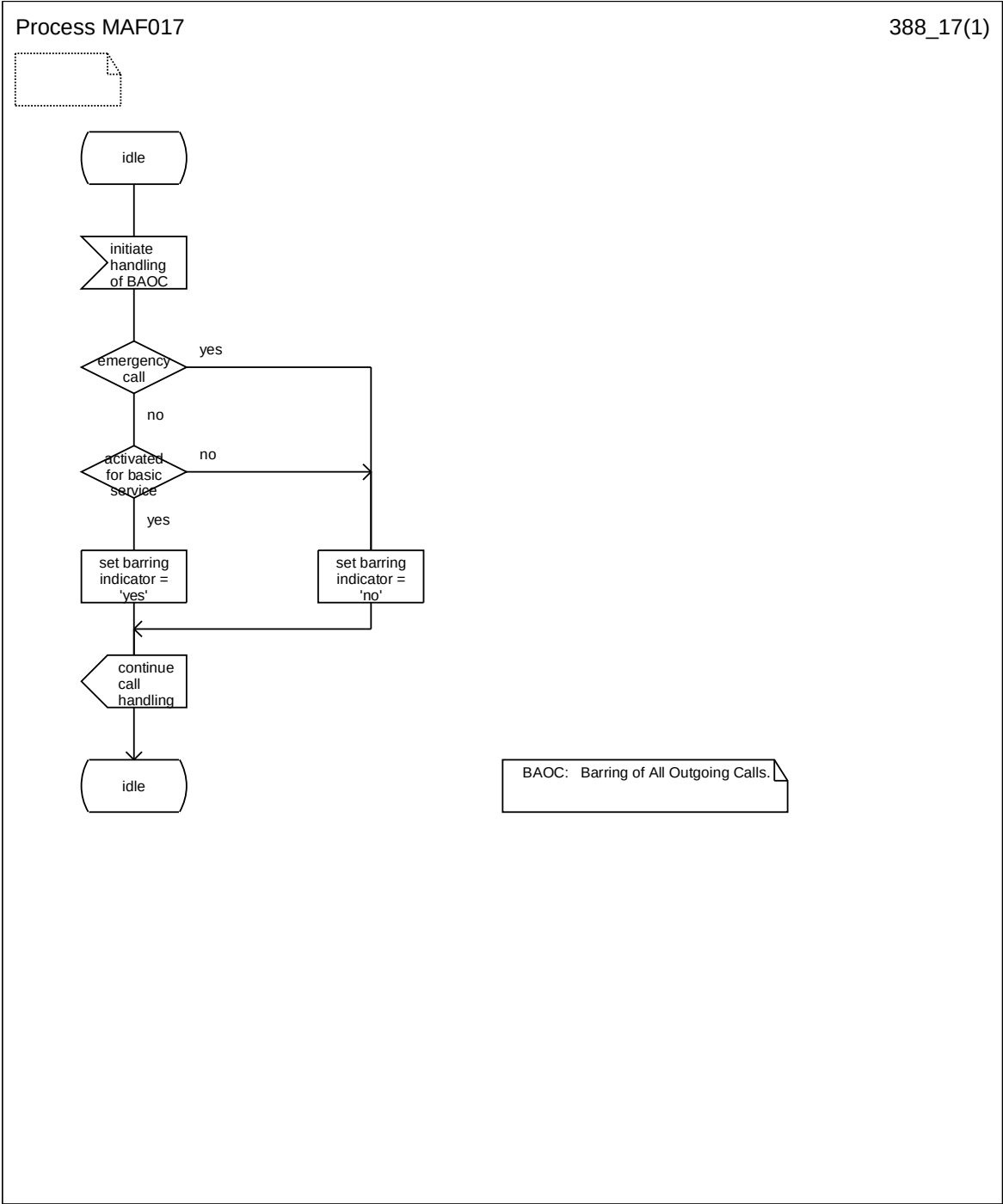
NOTE: Emergency call check is applied only at VLR. Figure 6.7: MAF017 Barring of all outgoing calls related authorisations examination (VLR/SGSN/MME)
