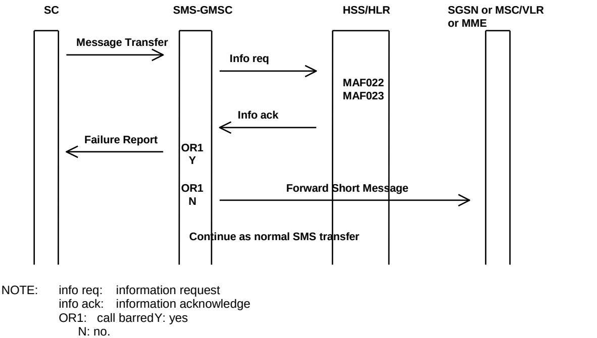
Figure 7.8B: Information flow for barring of MT SMS
