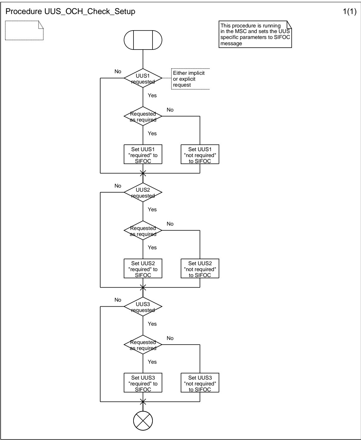
Figure 9.1.1.1: Procedure UUS_OCH_Check_Setup
