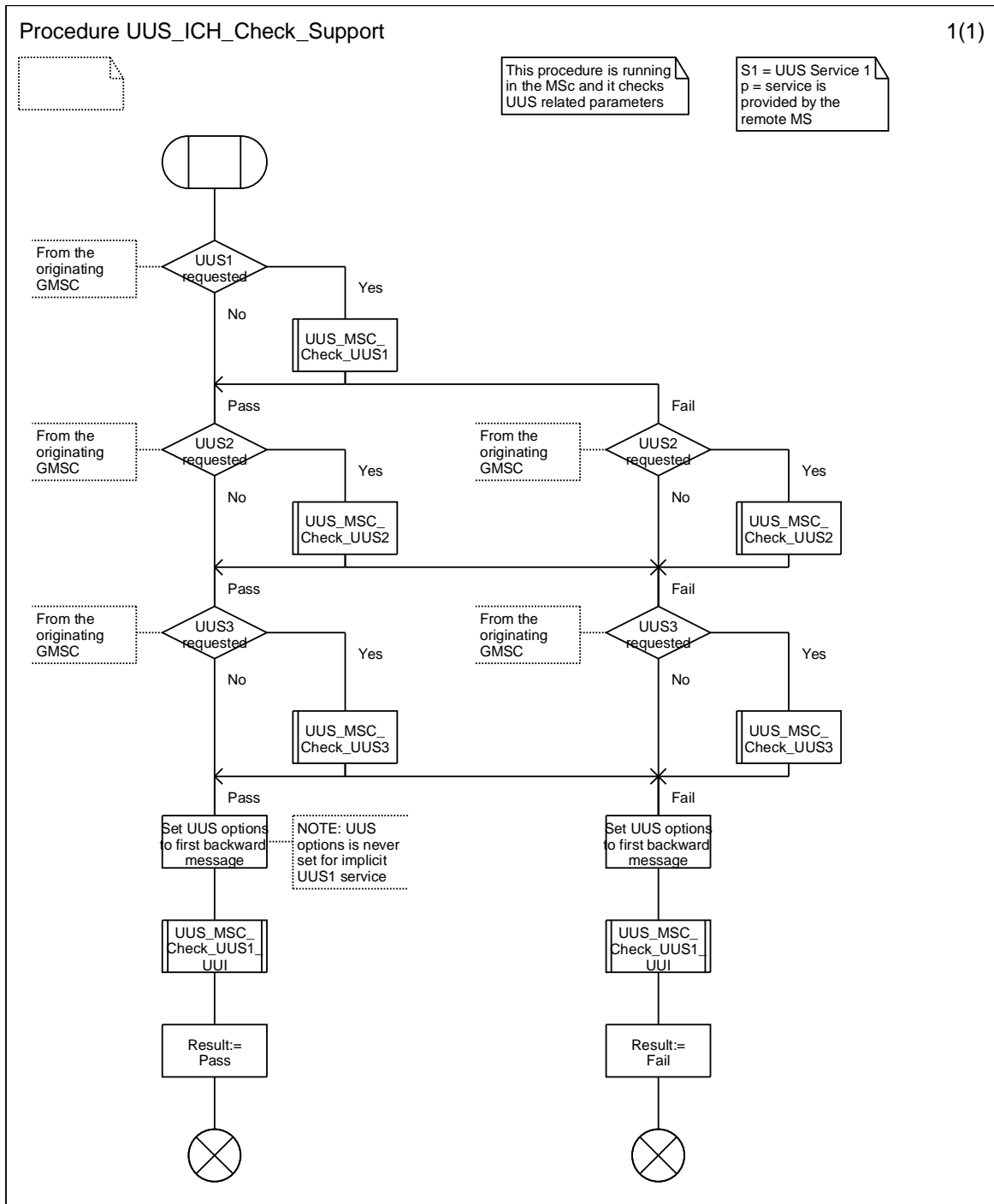
Figure 9.2.2.1: Procedure UUS_ICH_Check_Support
