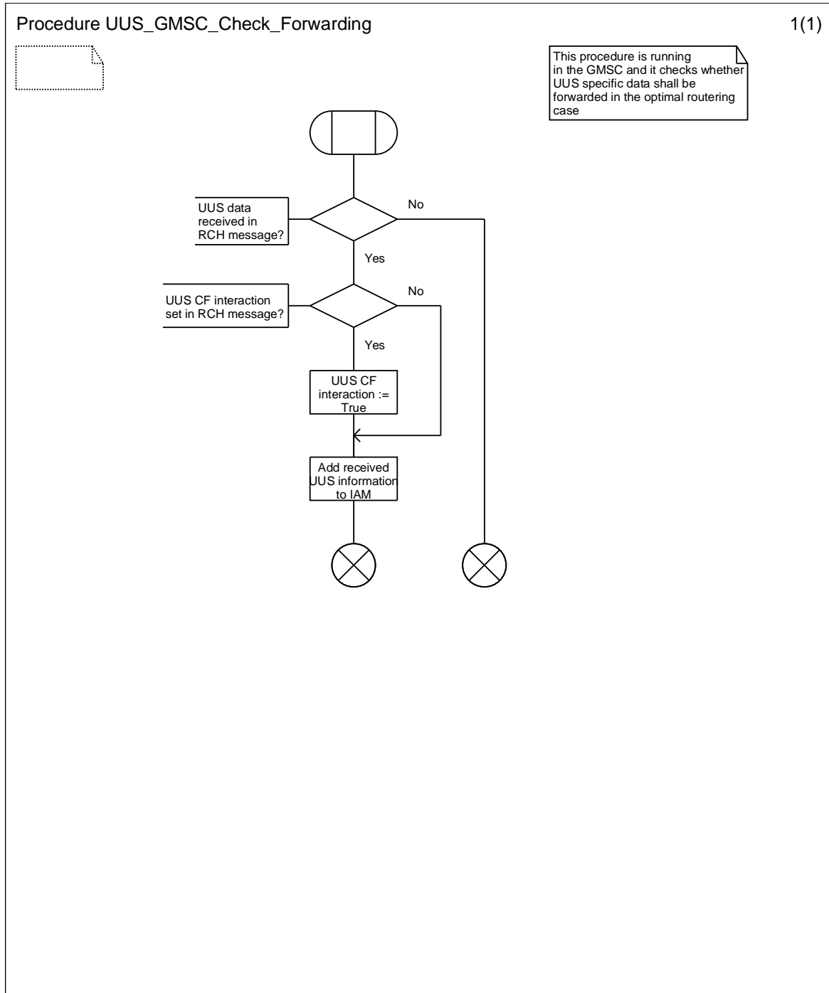
Figure 9.2.1.1: Procedure UUS_GMSC_Check_Forwarding
