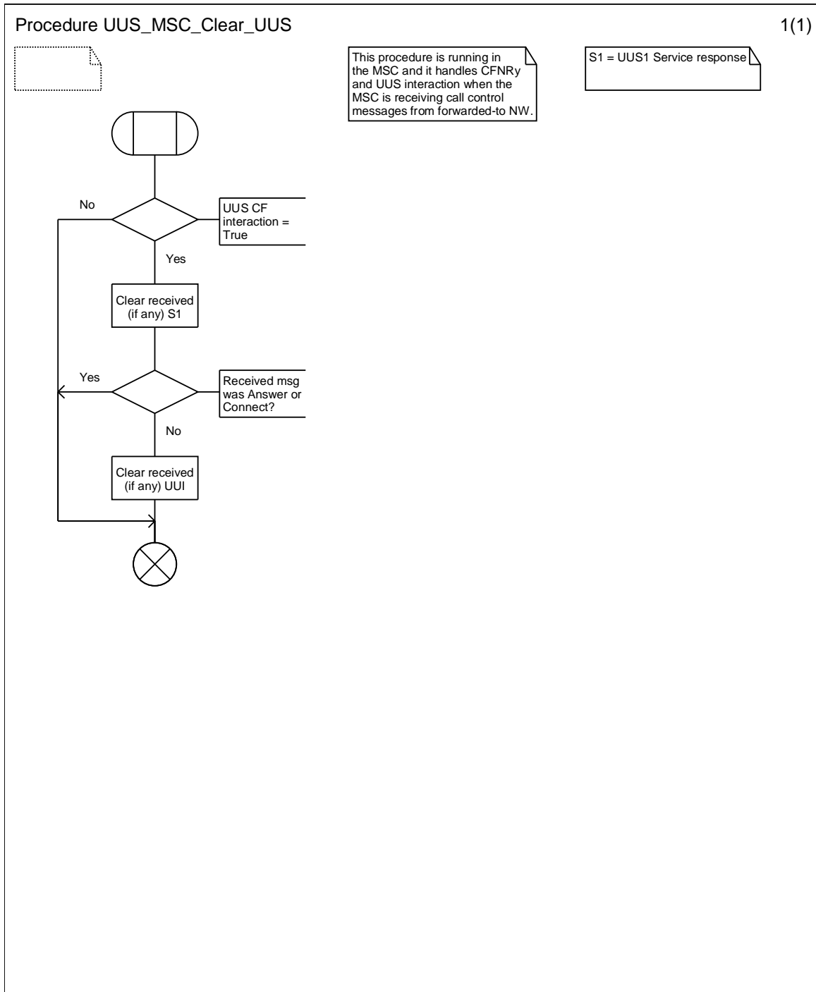
Figure 9.3.6: Procedure UUS_MSC_Clear_UUS
