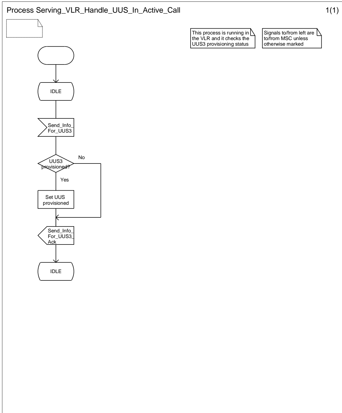
Figure 9.4.2.1: Process Serving_VLR_Handle_UUS_In_Active_Call
