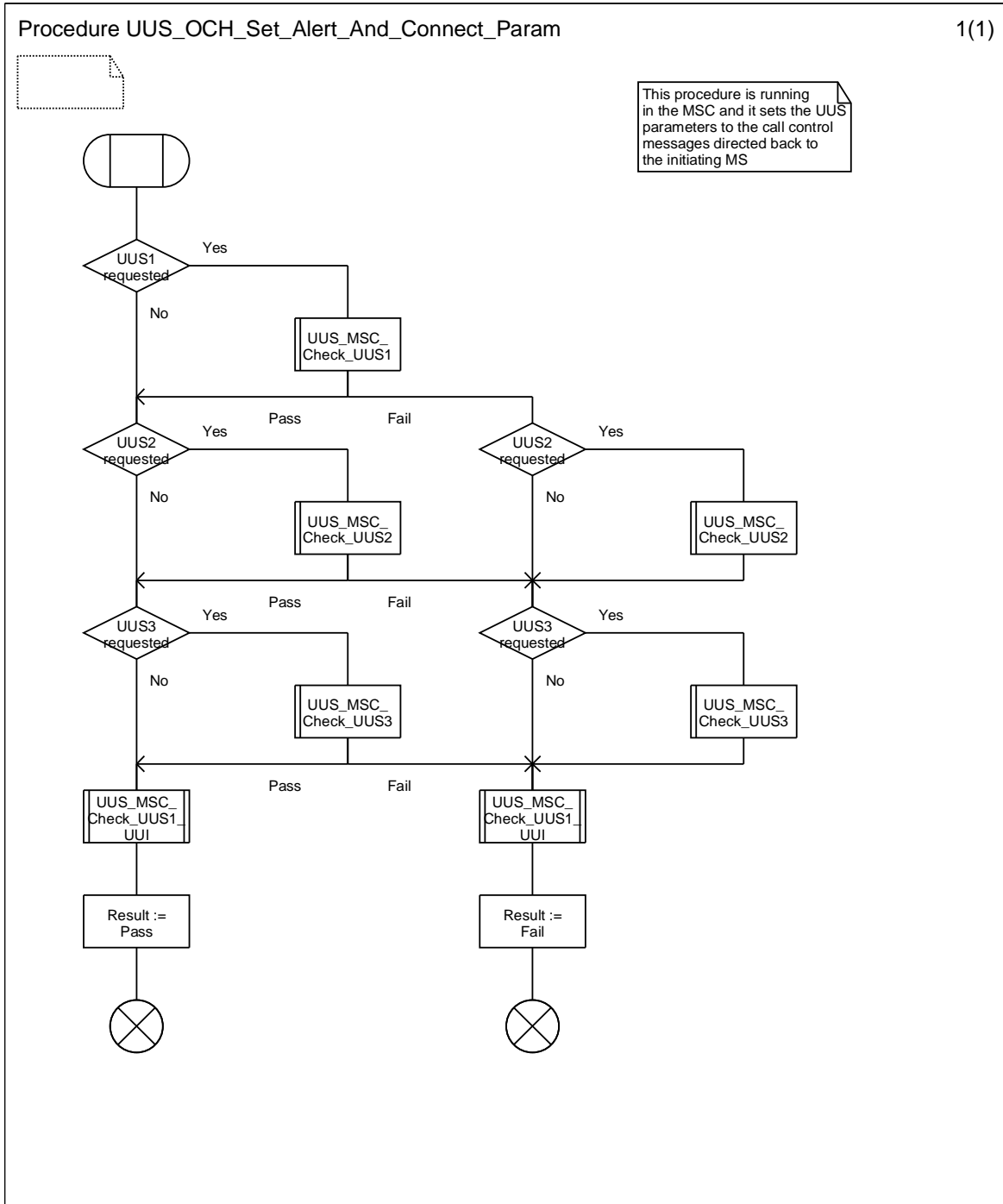
Figure 9.1.1.3: Procedure UUS_OCH_Set_Alert_And_Connect_Param
