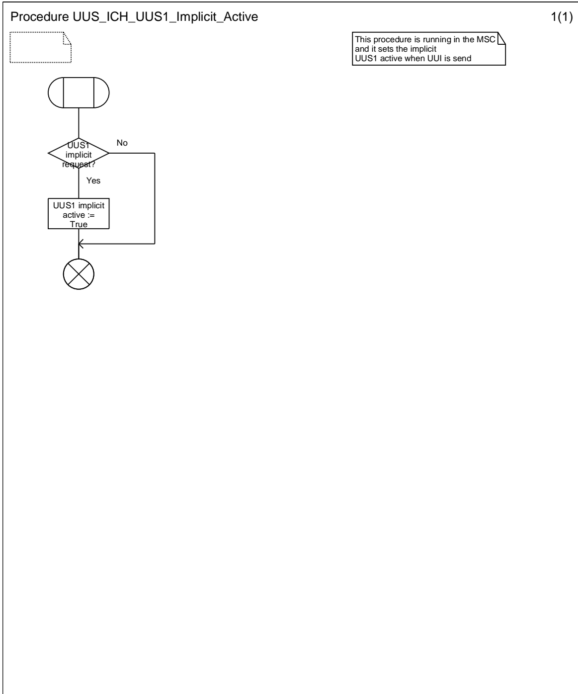
Figure 9.2.2.5: Procedure UUS_ICH_UUS1_Implicit_Active
