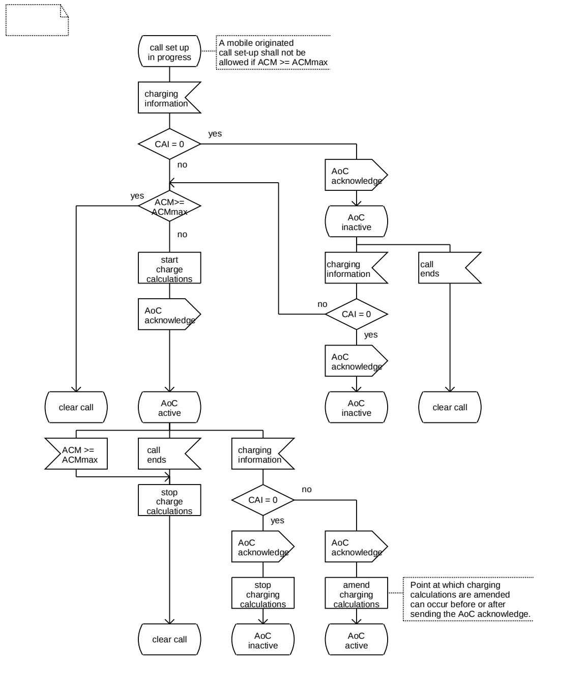
Figure 2.2: SDL diagram of advice of charge (charging) in the mobile equipment
