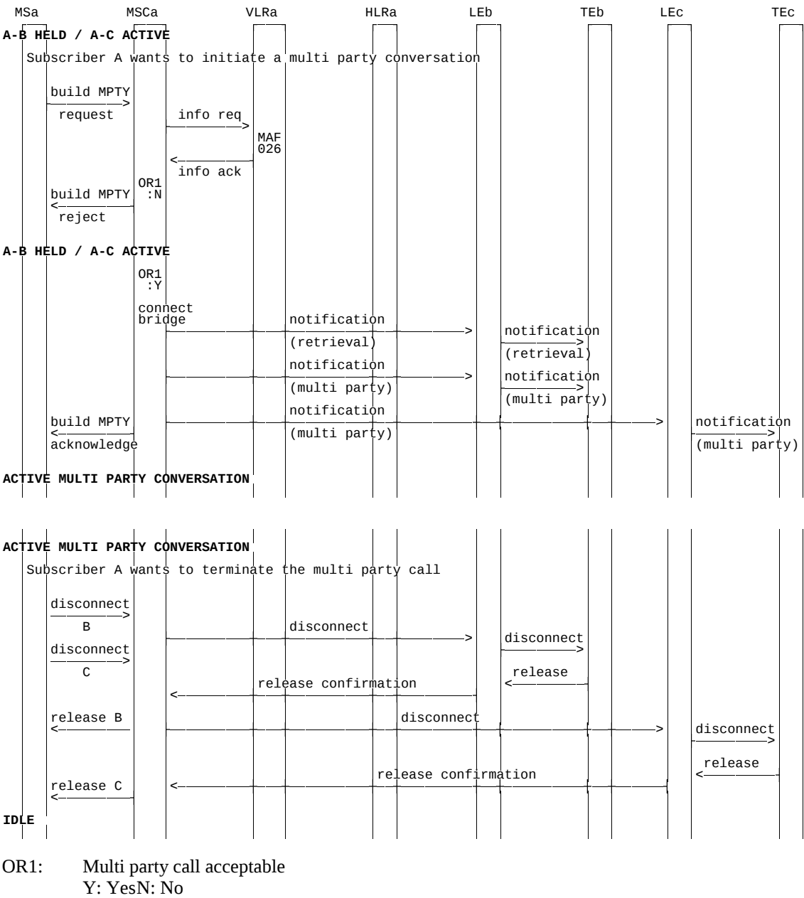
Figure 1.5 (sheet 1 of 7): Information flow for Multi Party service
