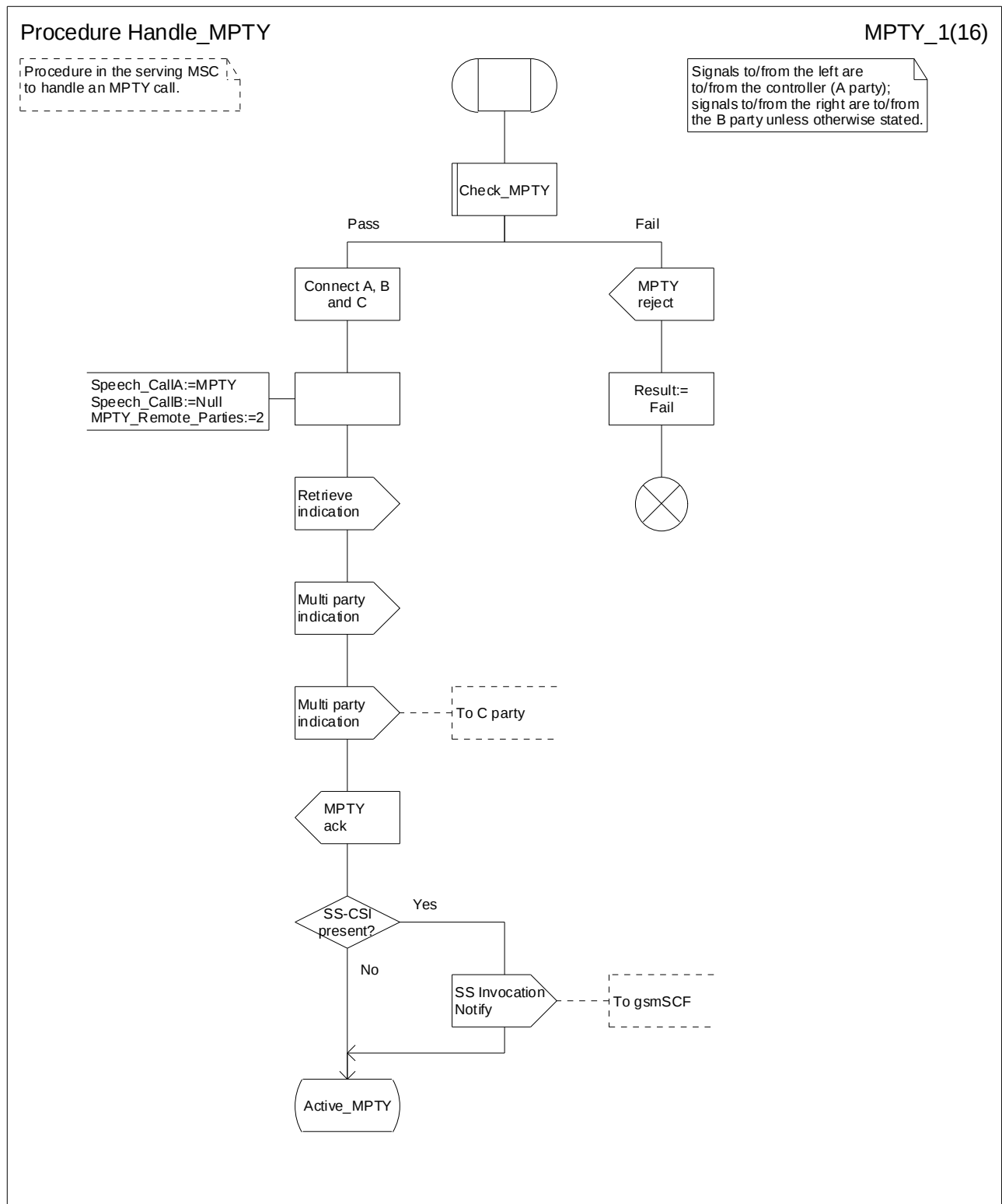
Figure 1.2 (sheet 1 of 16): Procedure Handle_MPTY
