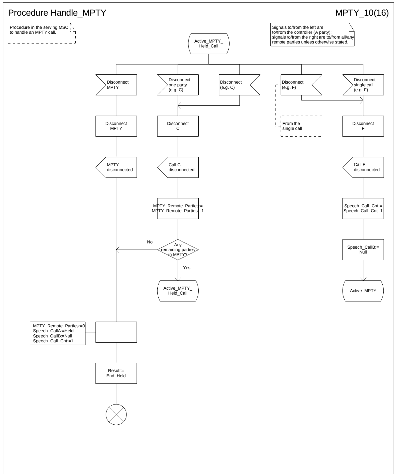
Figure 1.2 (sheet 10 of 16): Procedure Handle_MPTY
