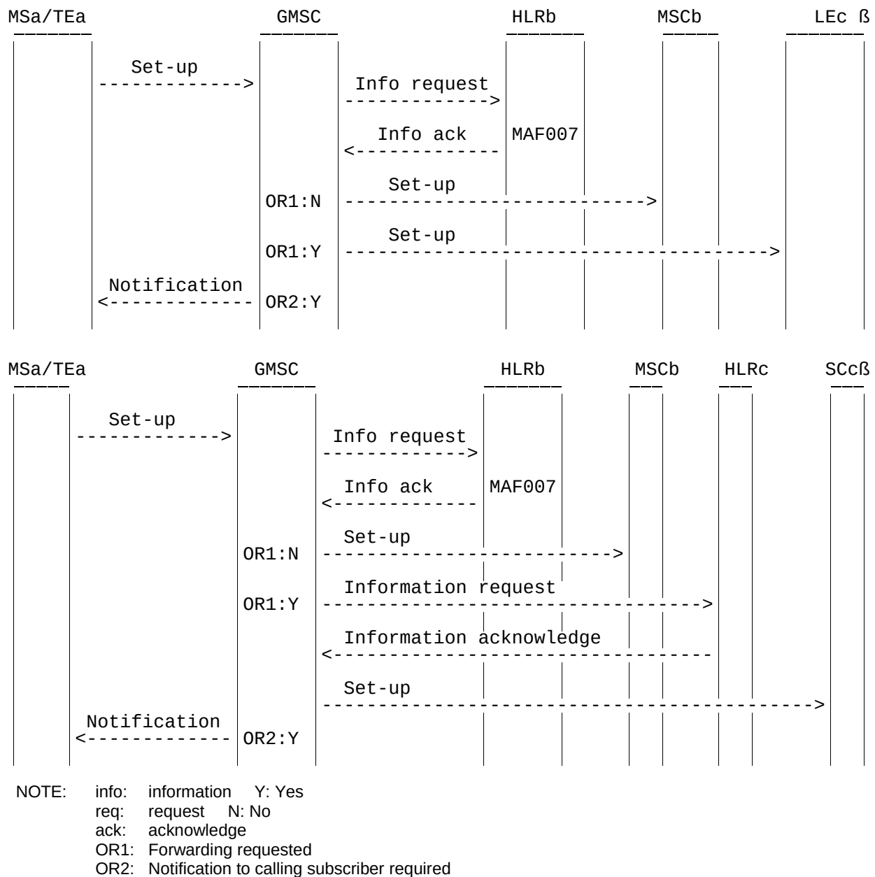
Figure 1.11: Information flow for call forwarding unconditional
