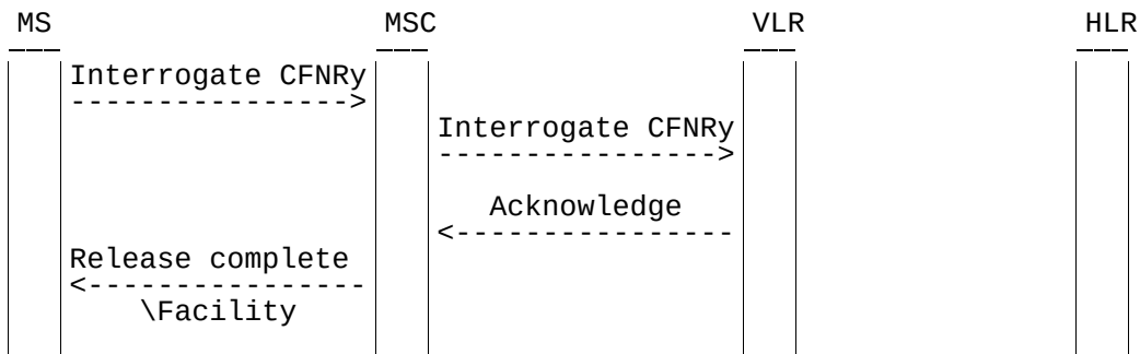
Figure 3.9: Interrogation of call forwarding on no reply
