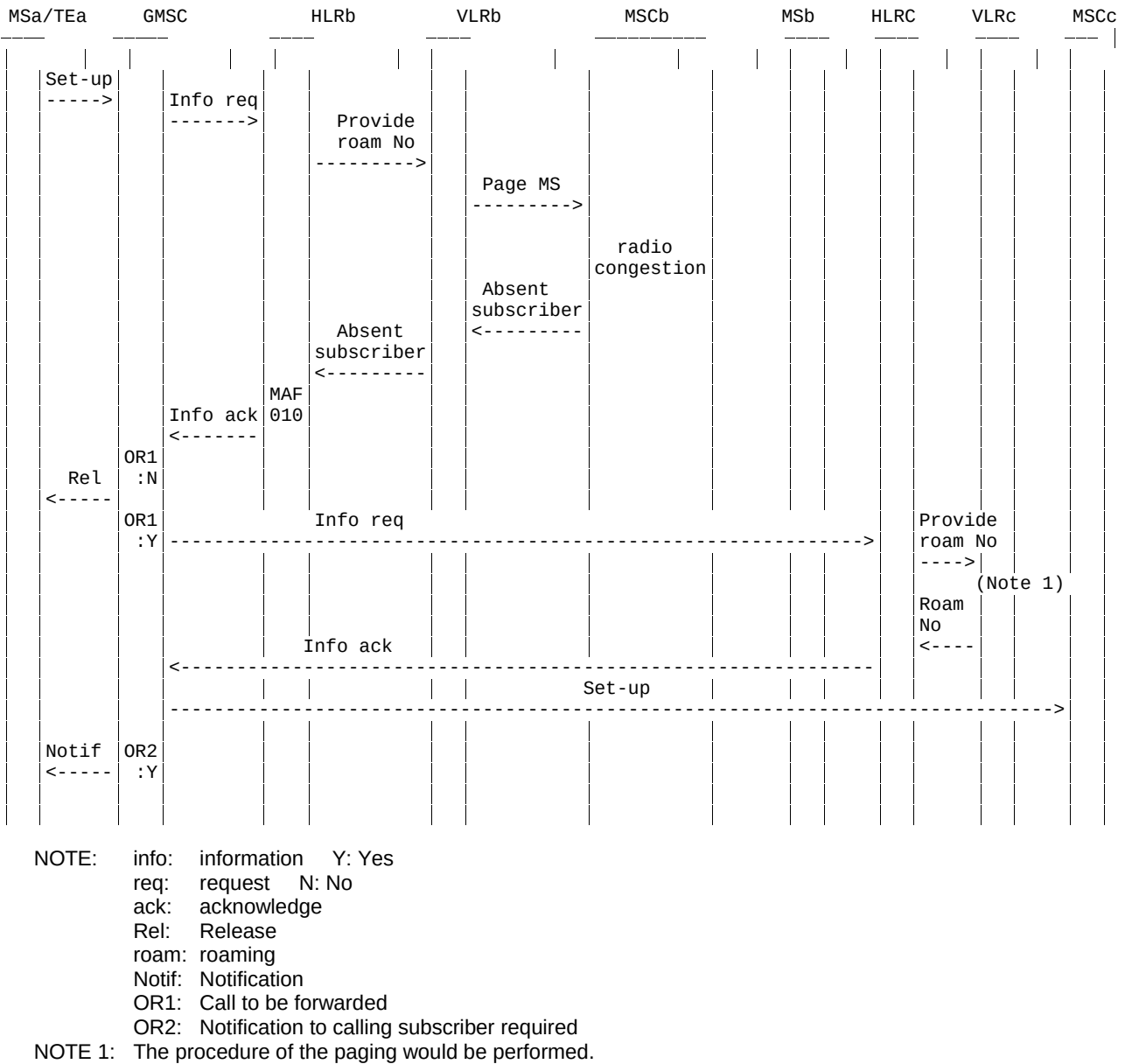
Figure 4.24: Information flow for call forwarding on mobile subscriber not reachable in case of radio congestion (to mobile station) (re-routing by HLR)
