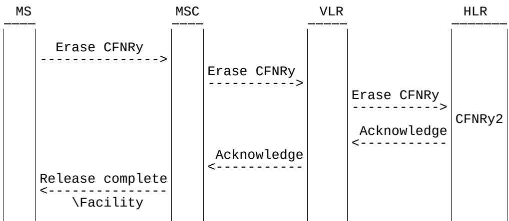
Figure 3.3: Erasure of call forwarding on no reply
