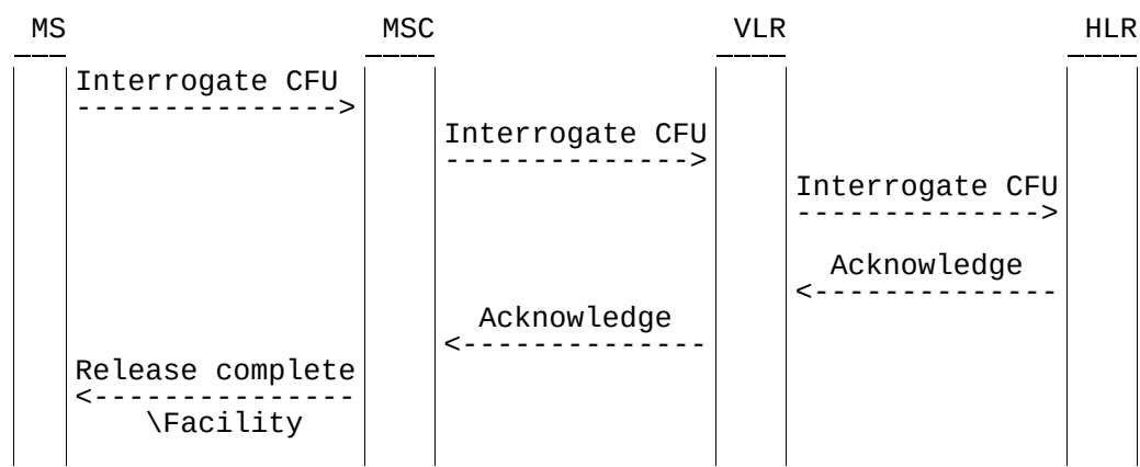
Figure 1.9: Interrogation of call forwarding unconditional
