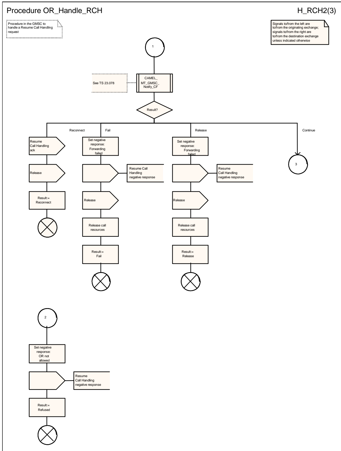
Figure 7b: Procedure OR_Handle_RCH (sheet 2)
