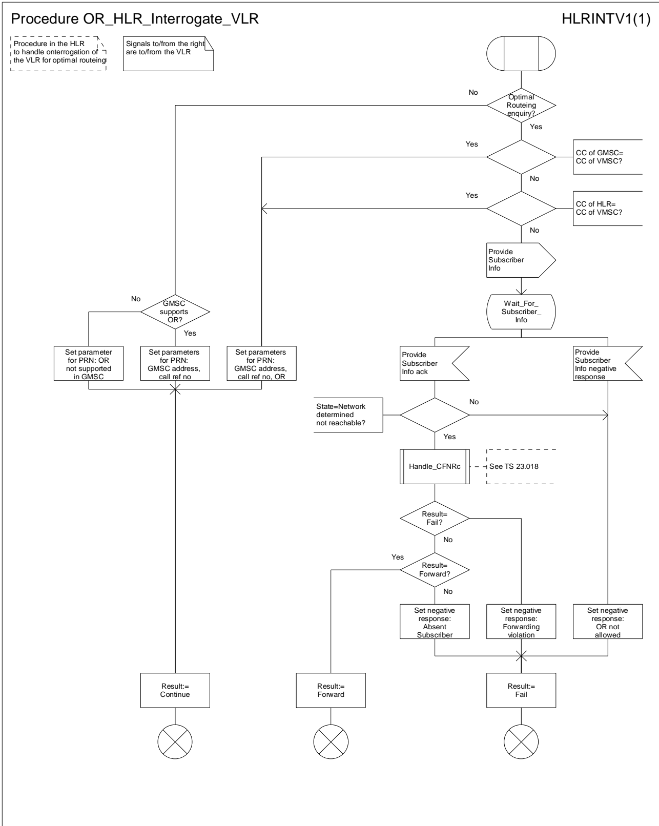
Figure 11: Procedure OR_HLR_Interrogate_VLR
