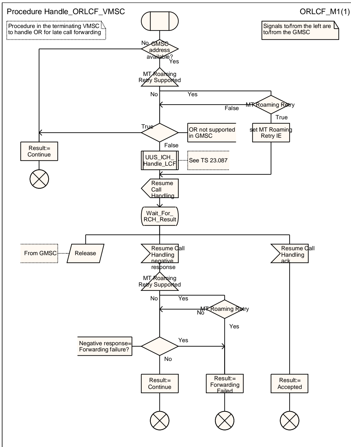
Figure 12: Procedure Handle_ORLCF_VMSC
