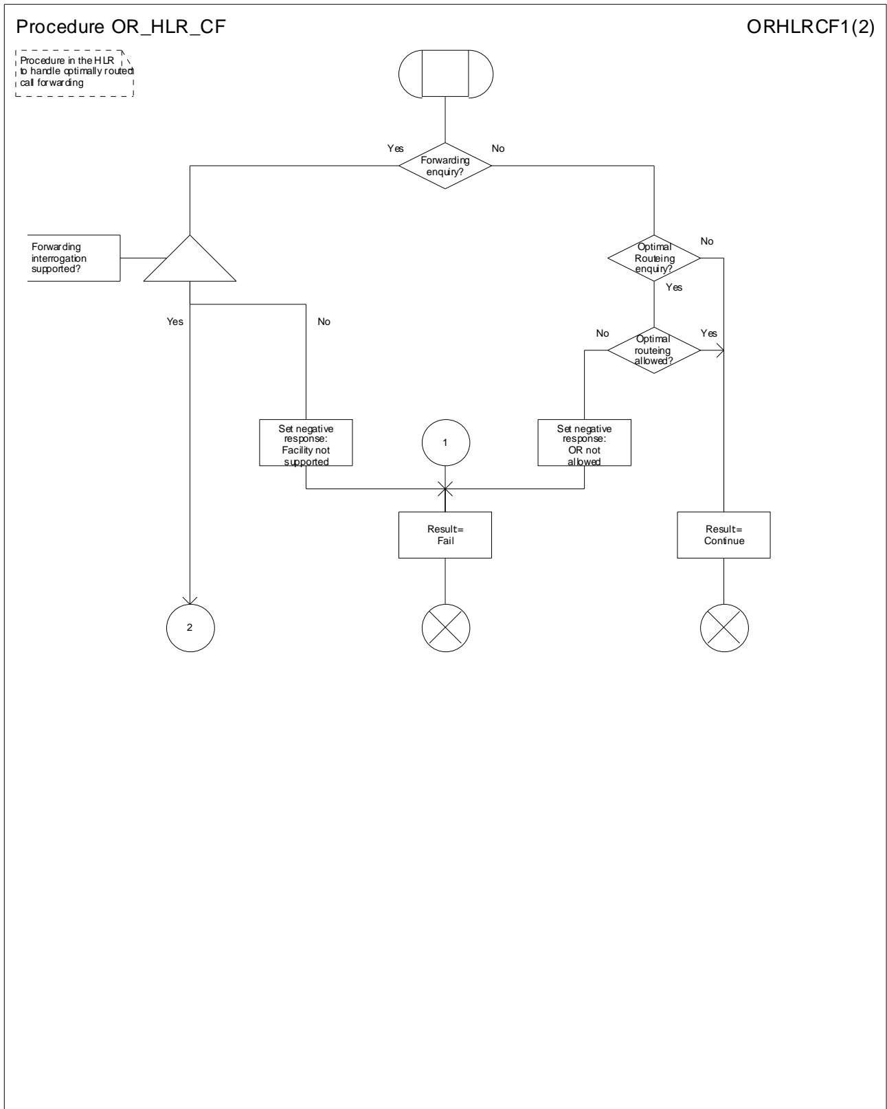
Figure 10a: Procedure OR_HLR_CF (sheet 1)
