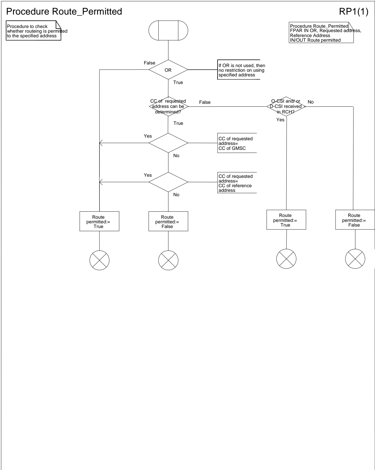
Figure 8: Procedure Route_Permitted
