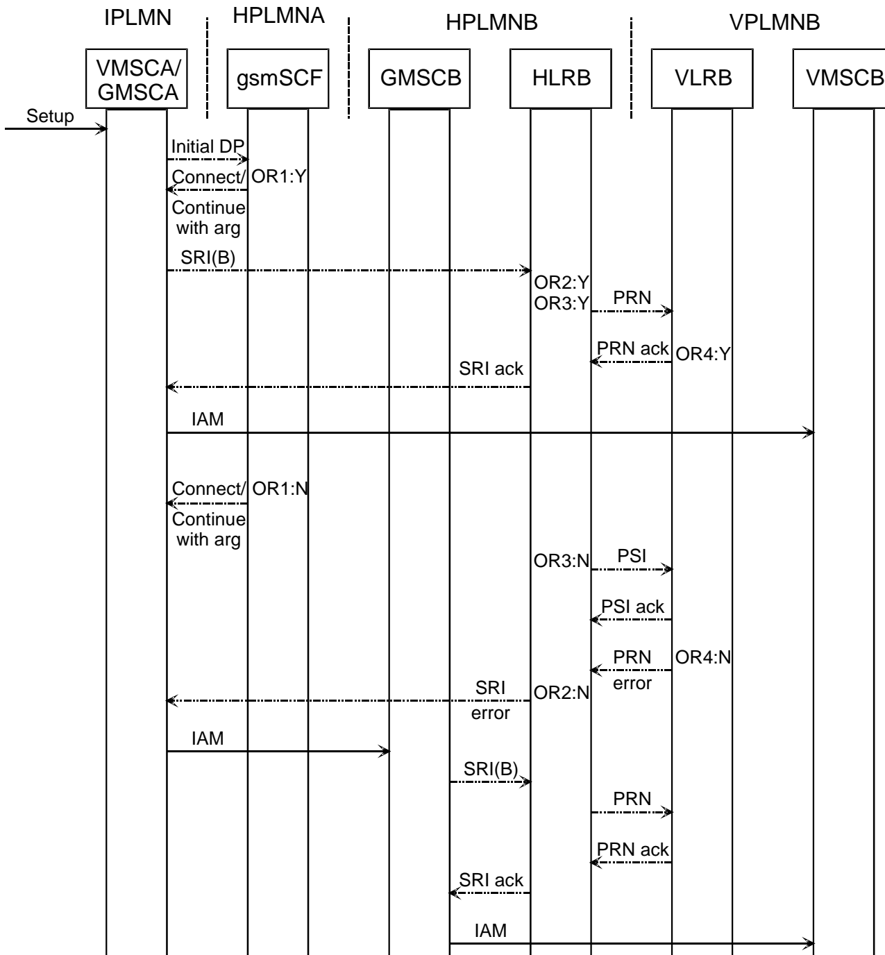
Figure 3: Message flow for optimal routeing of basic mobile-to-mobile call
