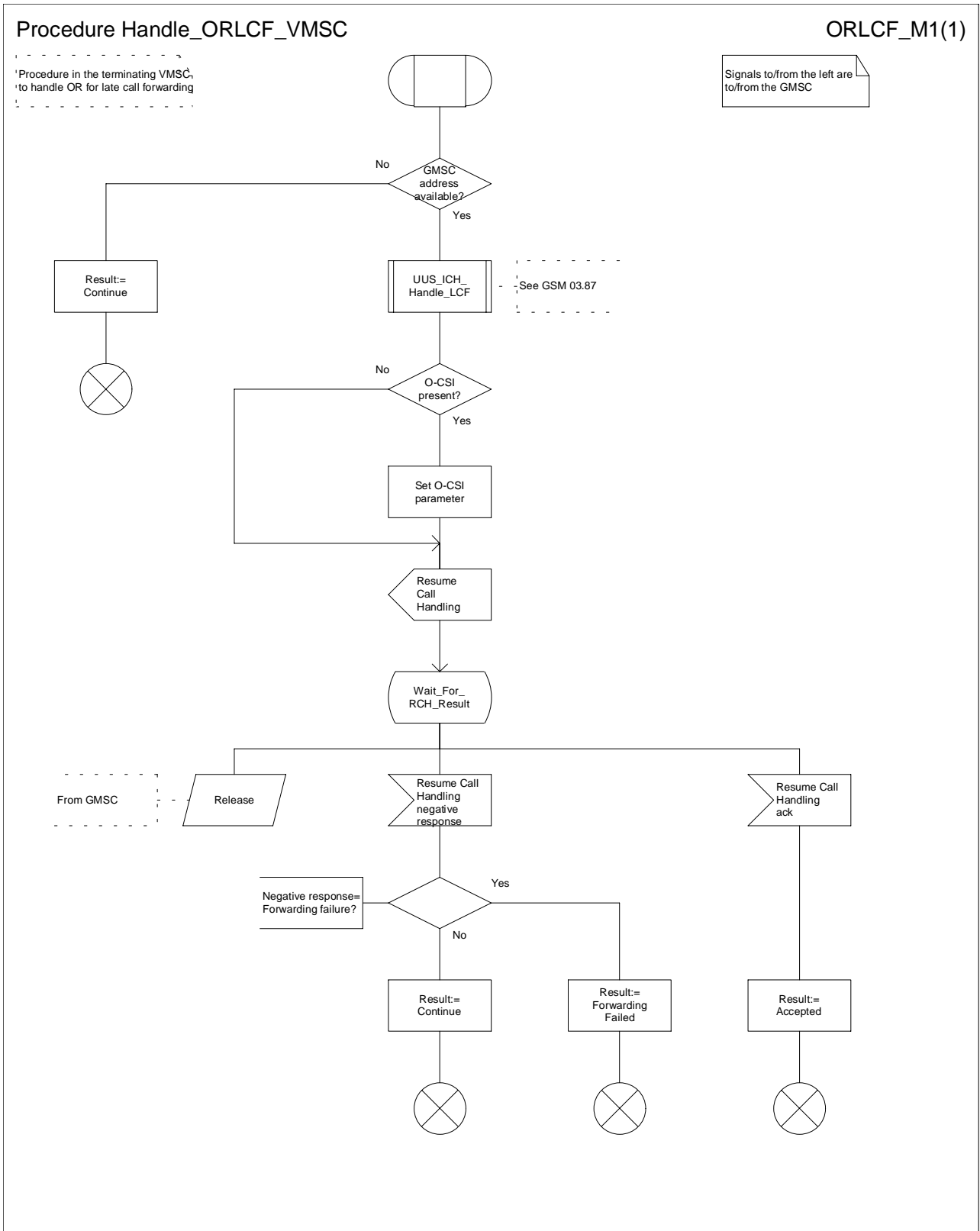
Figure 12: Procedure Handle_ORLCF_VMSC
