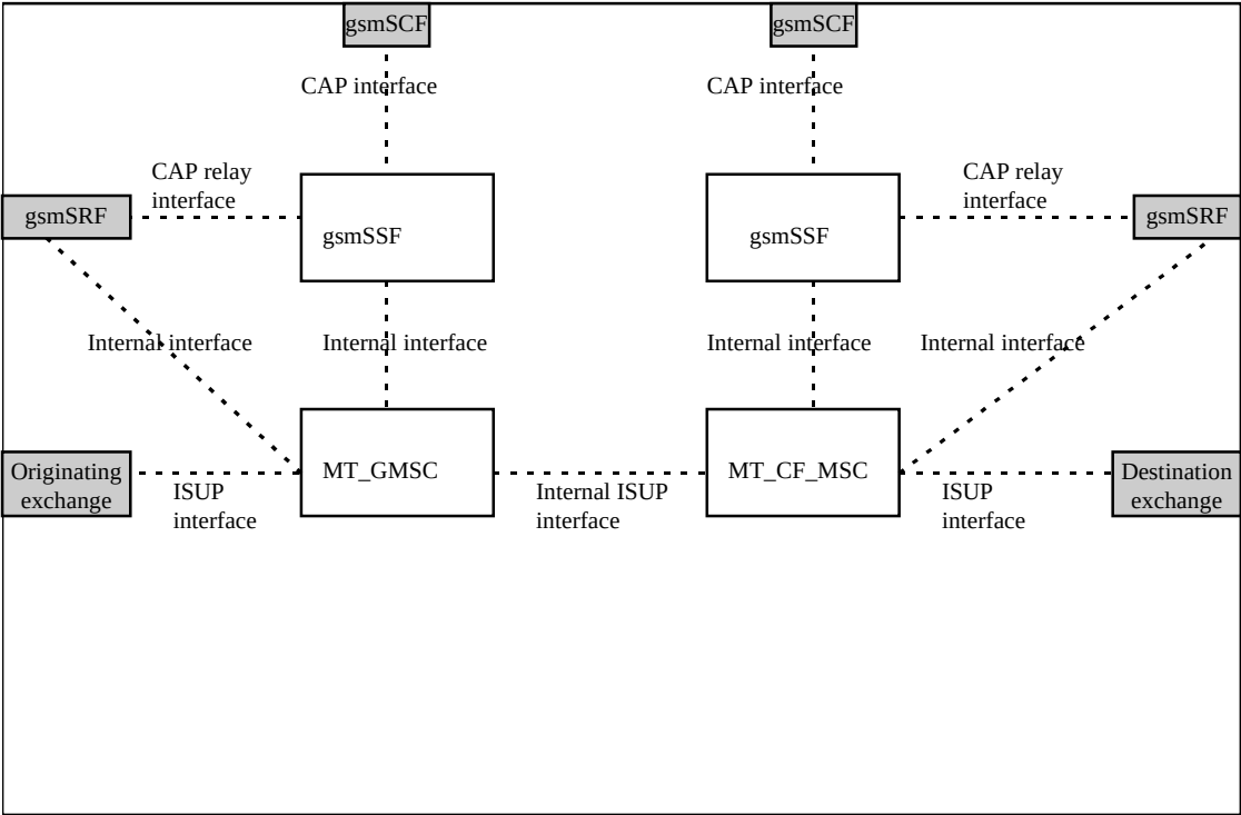
Figure 4.8c: Terminating GMSC case (gsmSSF relay)
