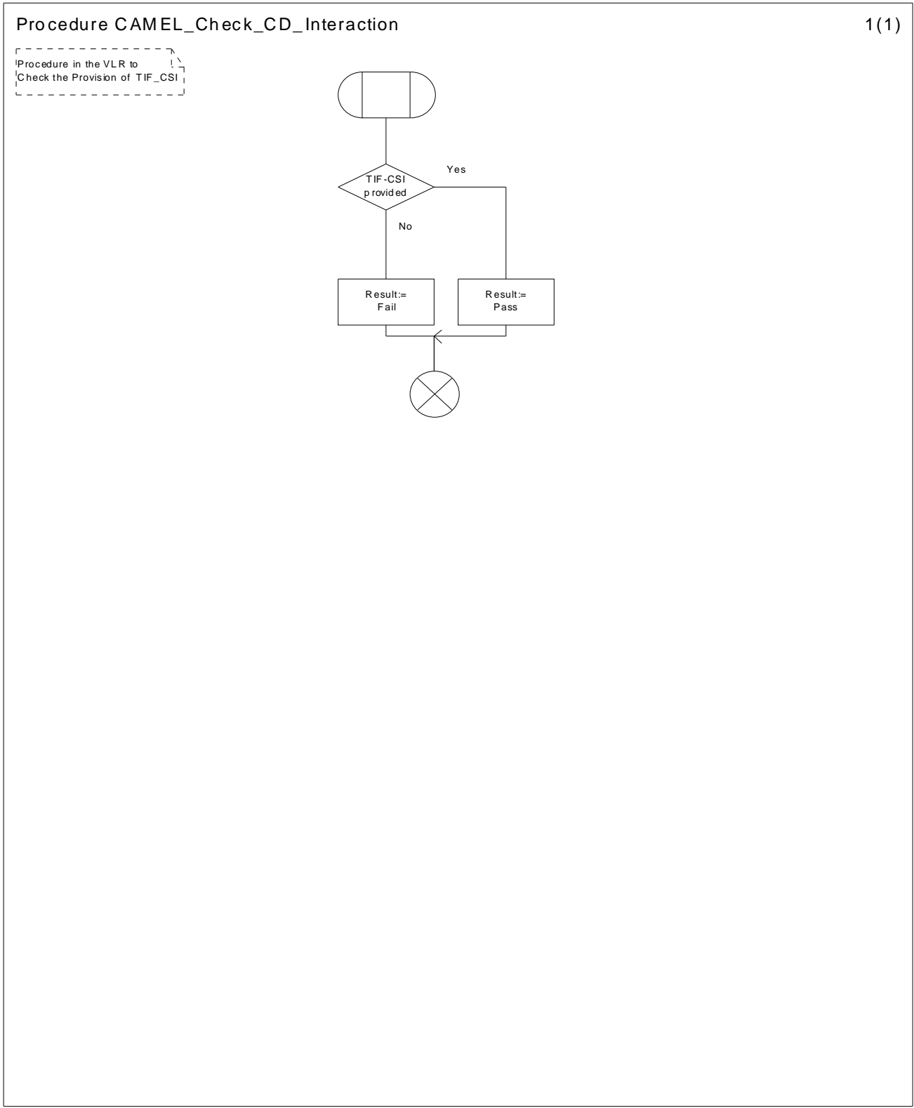
Figure 7.2: Procedure CAMEL_Check_CD_Interaction
