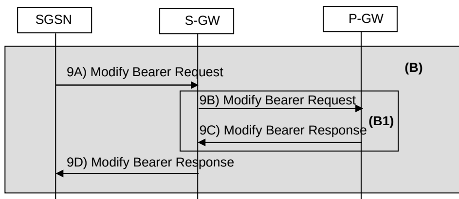
Figure 36b: Step 9 for Iu Mode Routeing Area Update Procedure using S4
