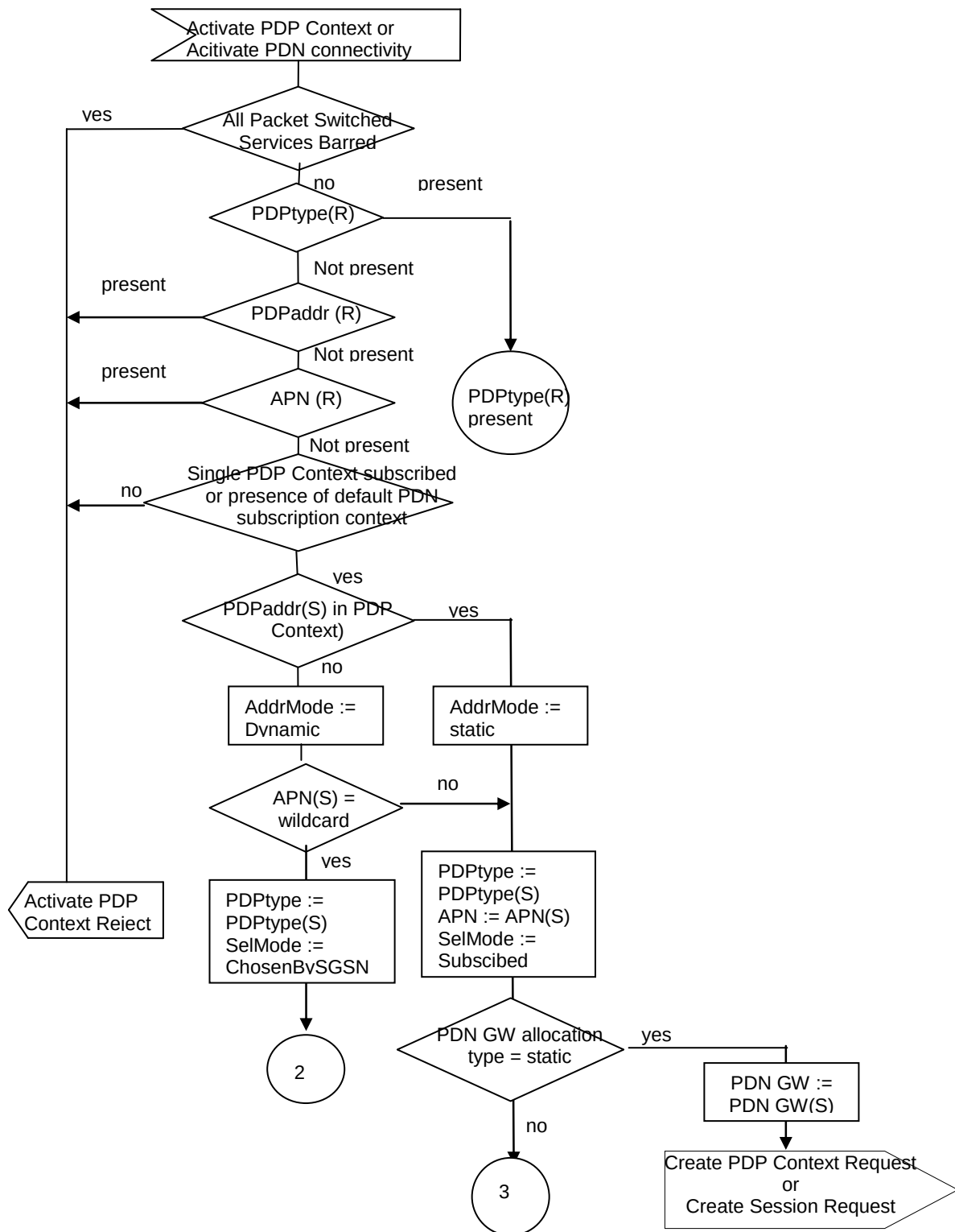
Figure A.1: APN selection-Null Parameter present
