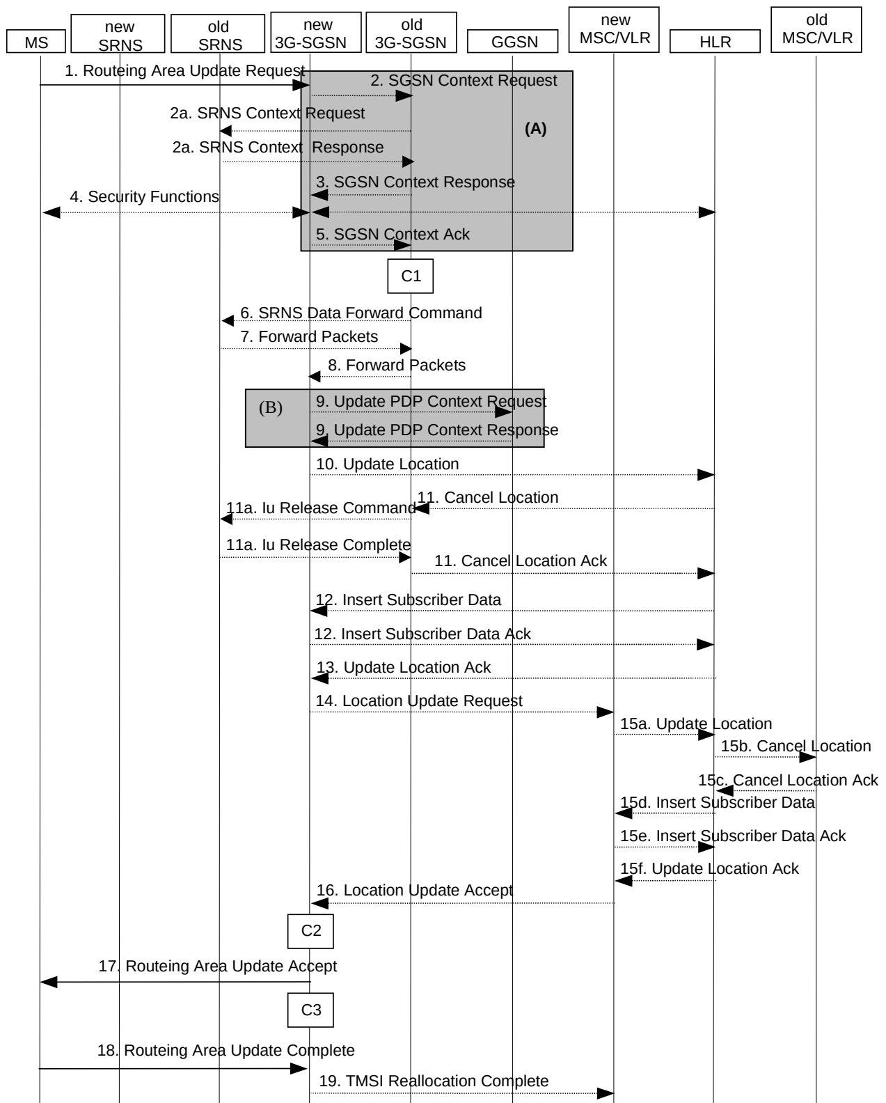
Figure 36: Iu mode RA Update Procedure
