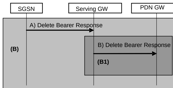
Figure 77b: PDN GW initiated Bearer Deactivation Procedure using S4, part 2
