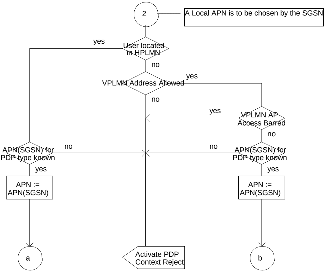
Figure A.5: SDL Diagram 5
