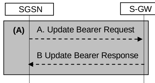
Figure 88b: RAB Release Procedure Using S4
