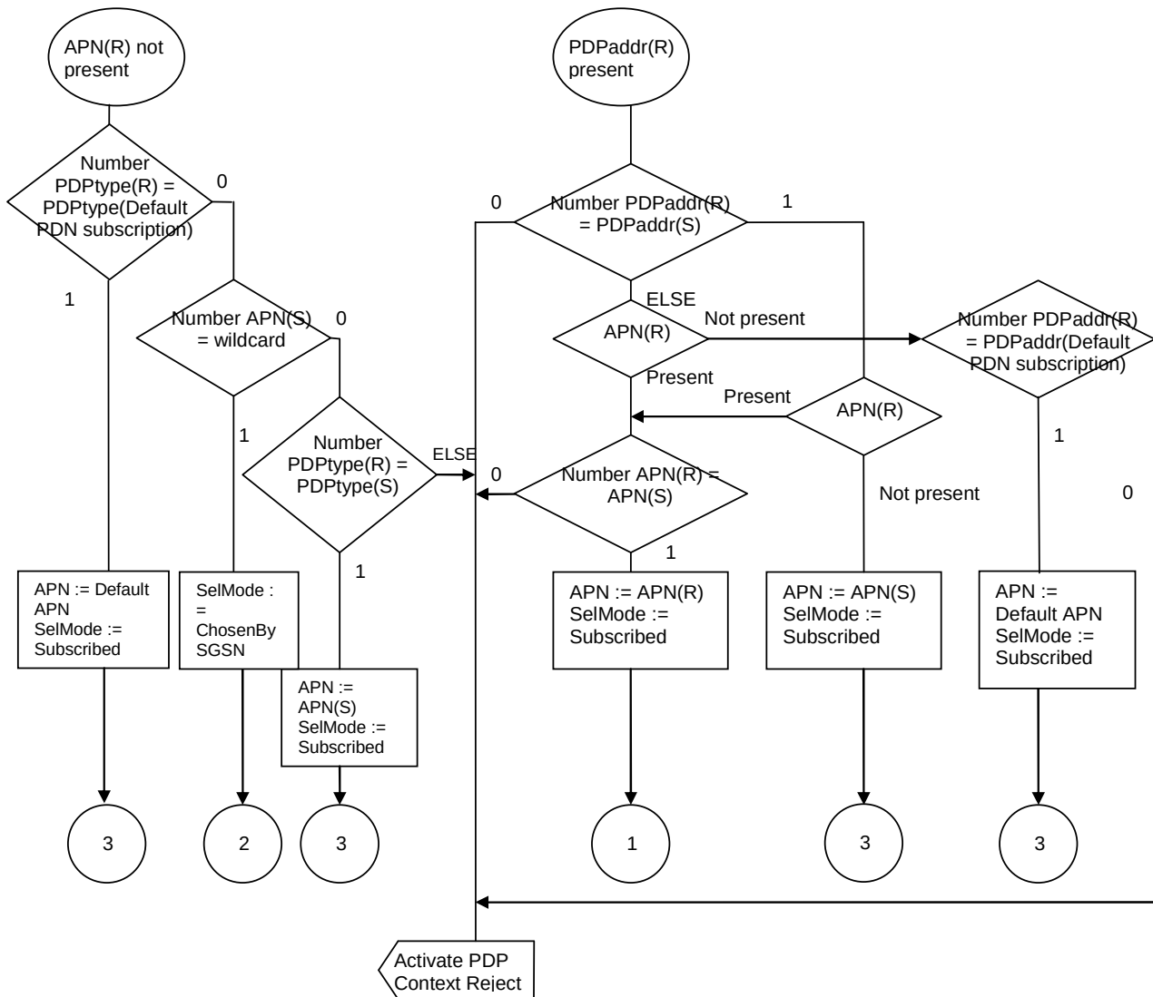
Figure A.3: SDL Diagram 3
