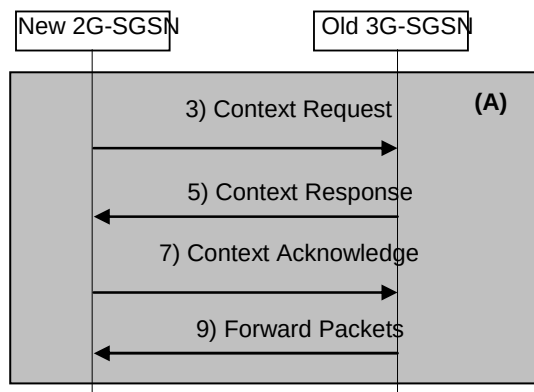
Figure 54-2: steps 3, 5, 7, 9 for lu mode to A/Gb mode Inter-SGSN Change using S4
