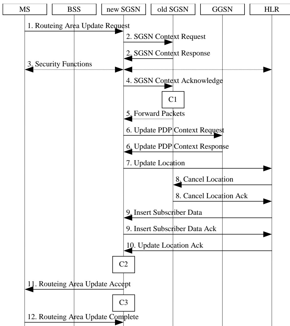
Figure 32: Inter SGSN Routing Area Update Procedure
