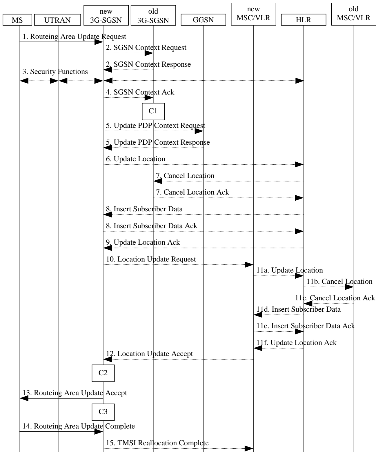
Figure 35: UMTS RA Update Procedure
