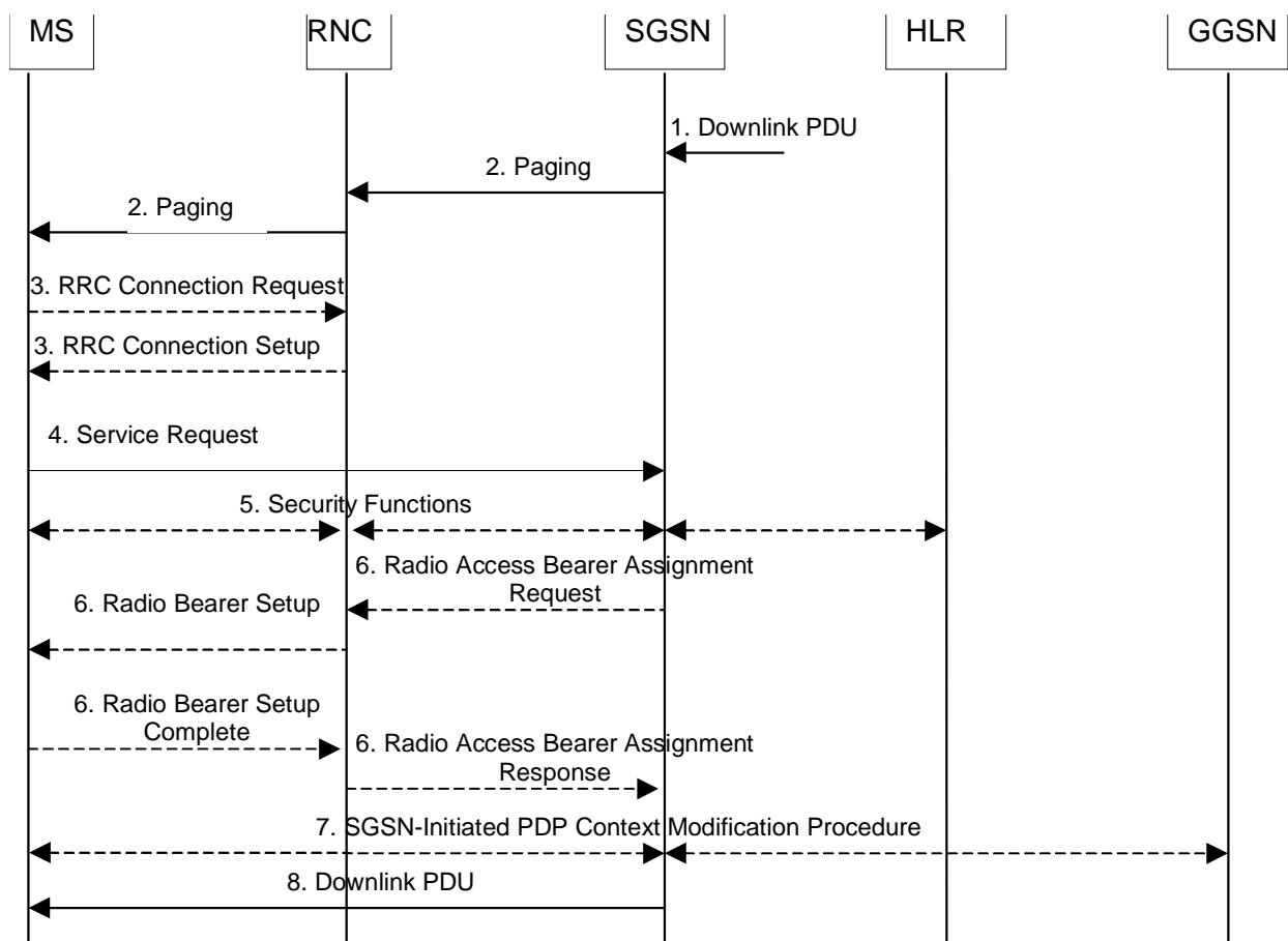
Figure 49: Service Request Initiated by Network Procedure
