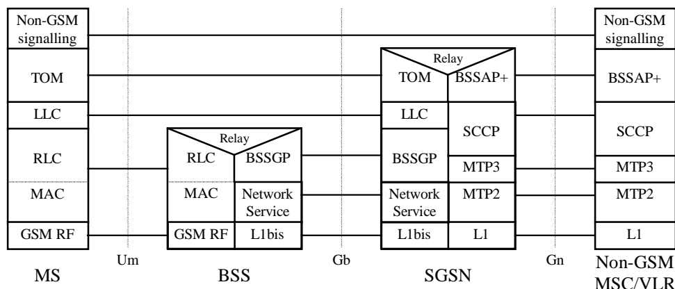
Figure 43: Control Plane MS - Non-GSM MSC/VLR
