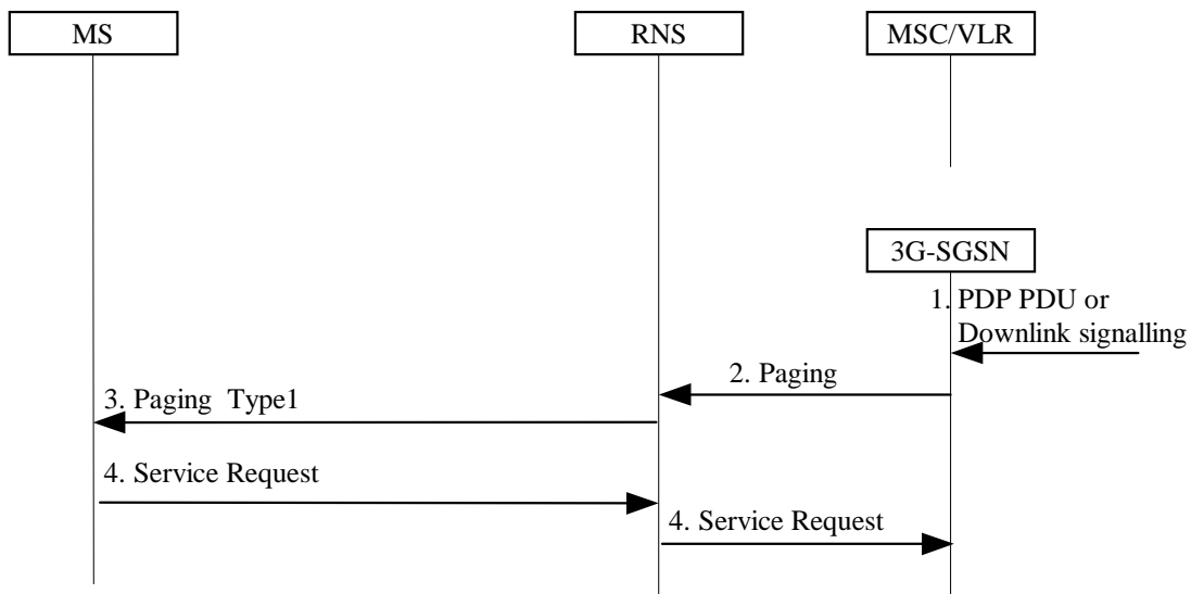
Figure 56: PS Paging Without RRC Connection for CS
