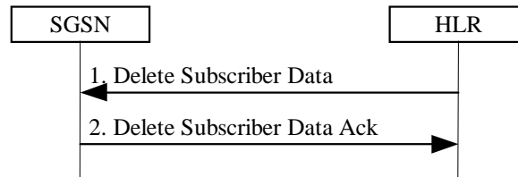
Figure 47: Delete Subscriber Data Procedure
