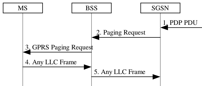
Figure 54: GPRS Paging Procedure
