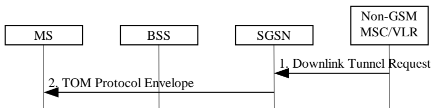
Figure 45: Downlink Tunnelling of non-GSM Signalling Messages Procedure
