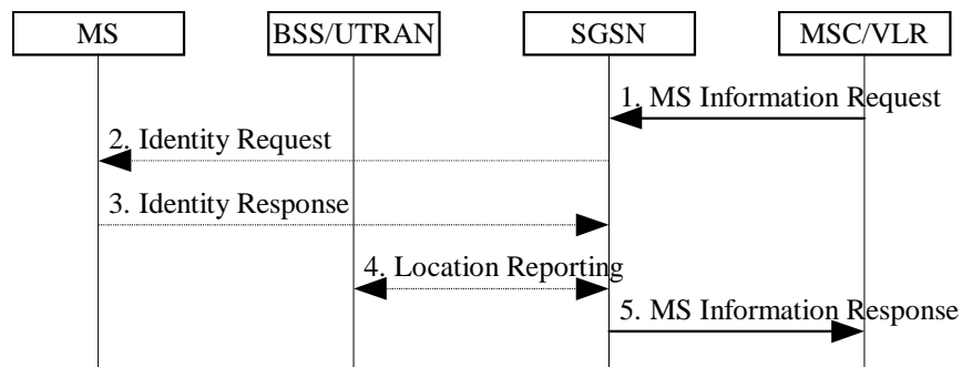
Figure 19: MS Information Procedure
