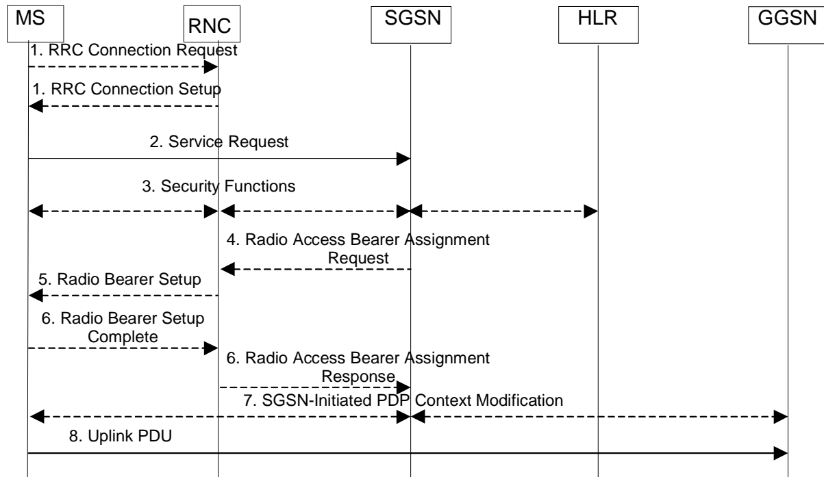
Figure 48: Service Request Initiated by MS Procedure
