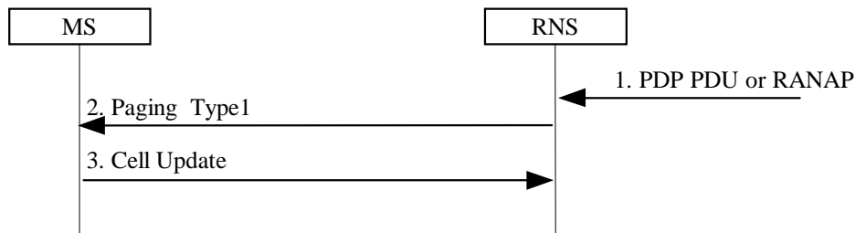
Figure 58: URA Paging Procedure
