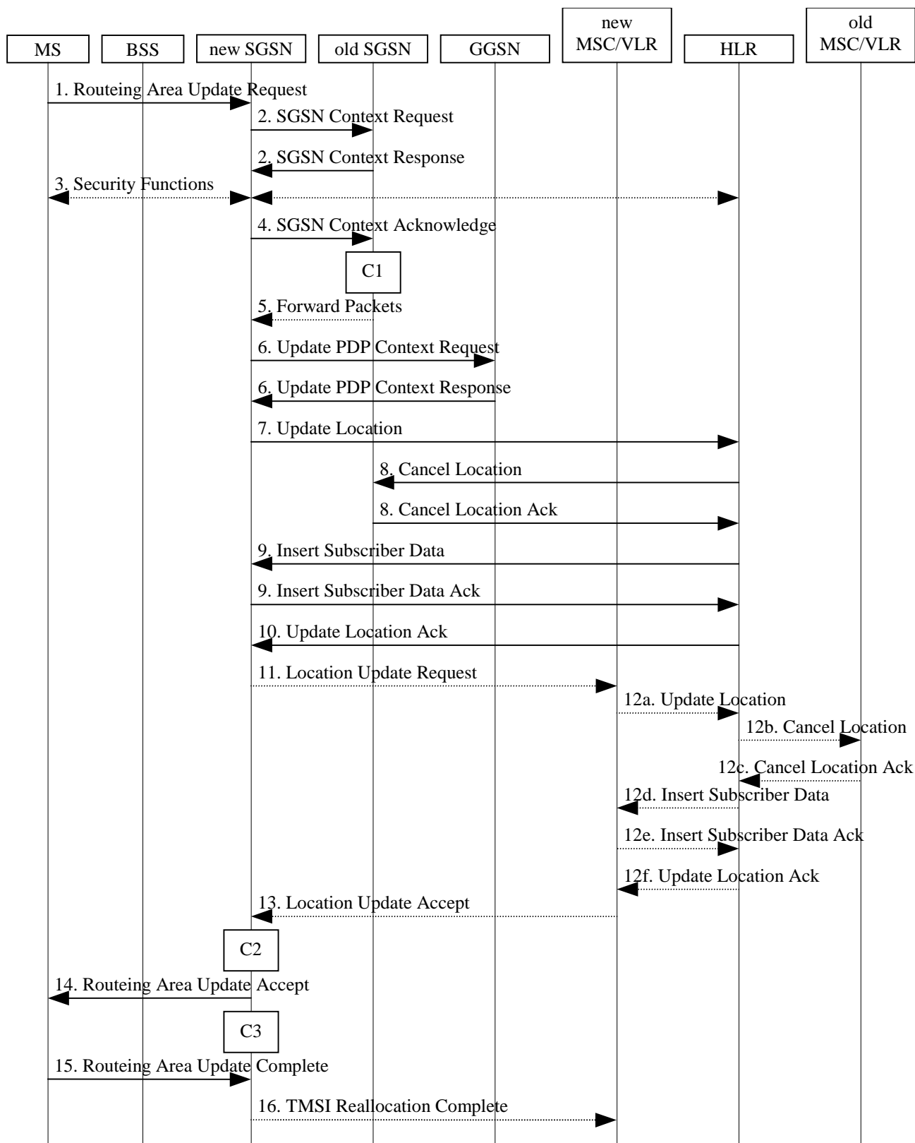
Figure 34: Combined RA / LA Update in the Case of Inter SGSN RA Update Procedure
