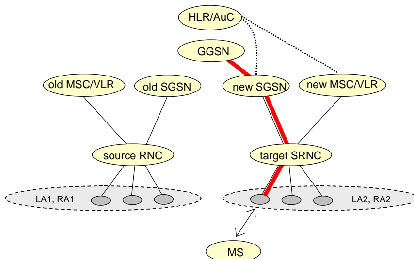
Figure 40: After Combined Hard Handover and SRNS Relocation and Routeing Area Update
