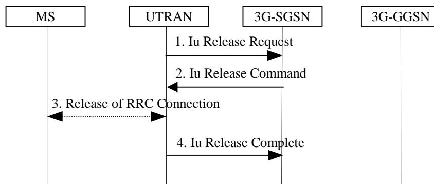
Figure 75: Iu Release Procedure
