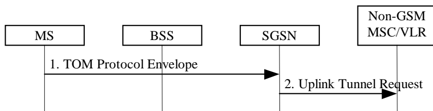
Figure 44: Uplink Tunnelling of non-GSM Signalling Messages Procedure
