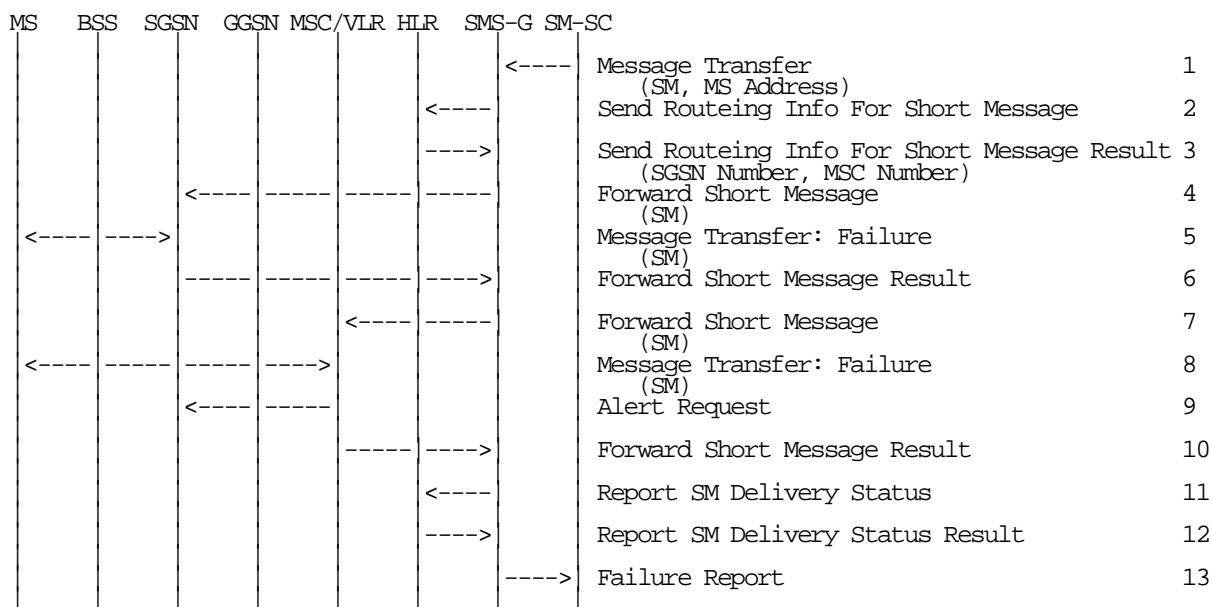
Figure 95: MT SMS Transfer, Unsuccessful
