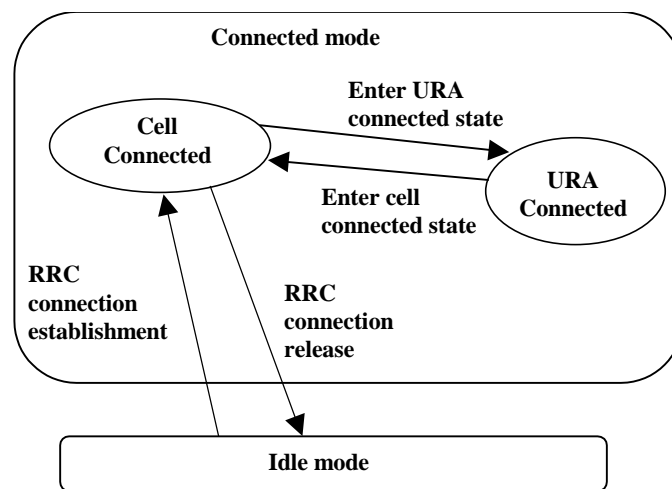
Figure 55: RRC Modes, Main RRC States and Main Mode and State Transition
