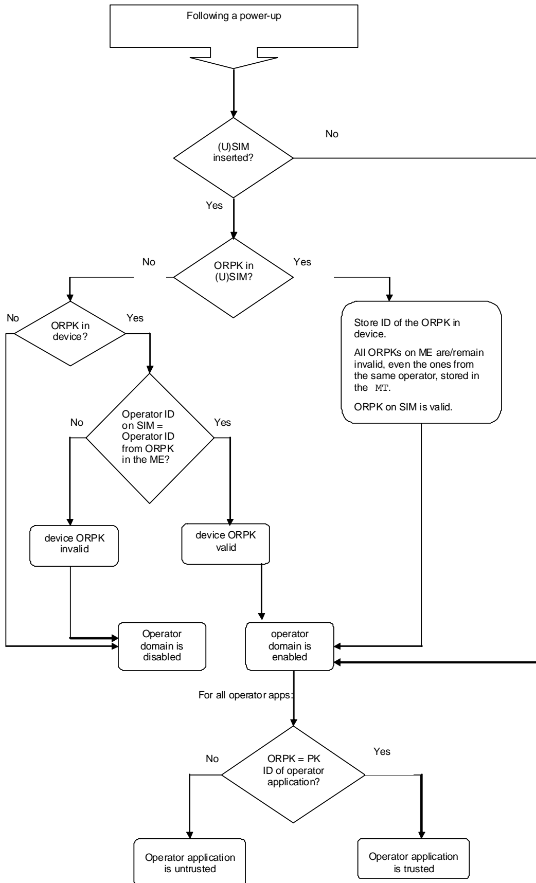
Figure 4: MExE device behaviour on power up
