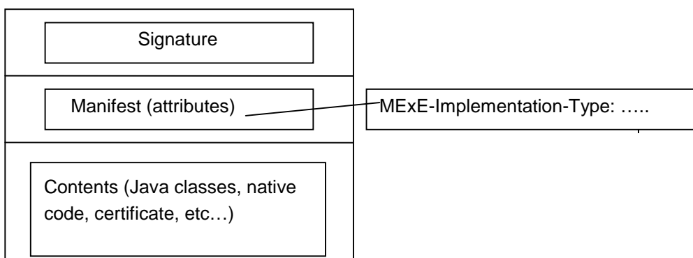
Figure 15: Signed packages
