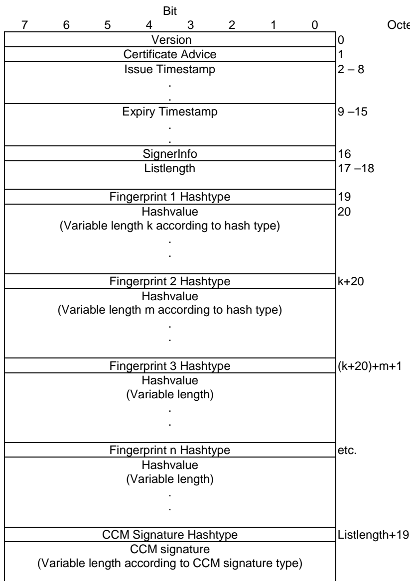
Figure 10: Format of a CCM
