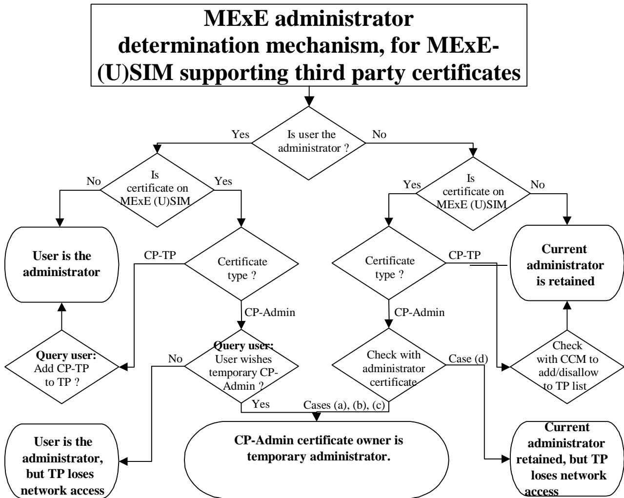
Figure 14: MExE administrator determination mechanism, for MExE-(U)SIM supporting third party certificates
