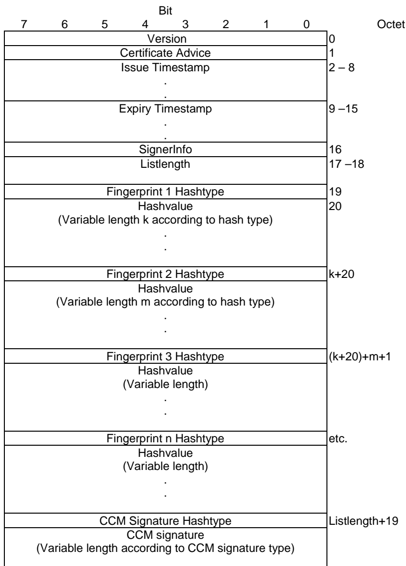
Figure 10: Format of a CCM
