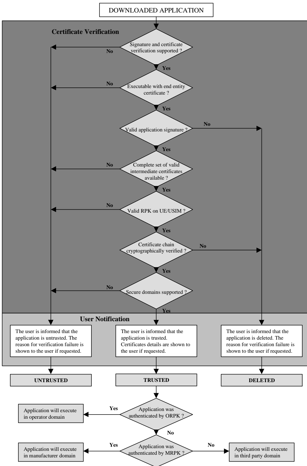
Figure 8: Certificate Chain Verification Diagram
