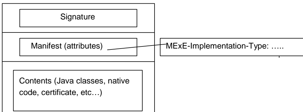
Figure 15: Signed packages
