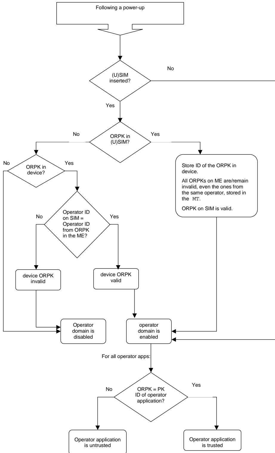
Figure 9: MExE device behaviour on power up
