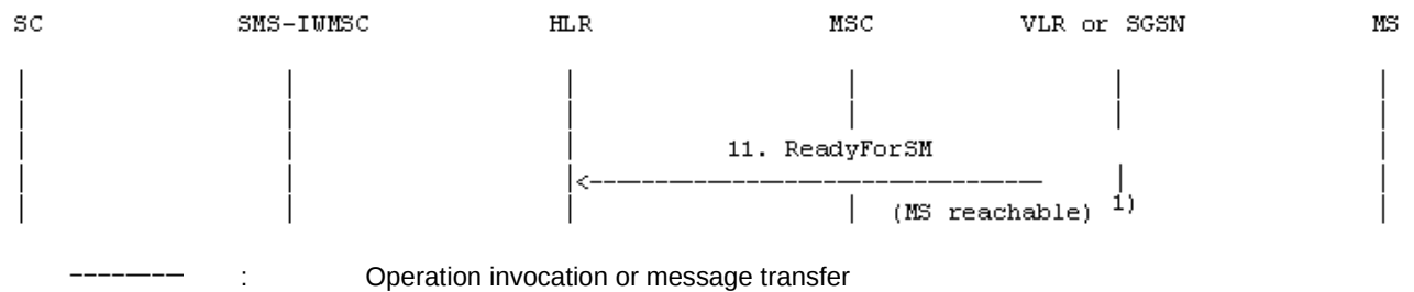
Figure 20a: The alert procedure when the MS becomes reachable, MNRF, MNRG or both are set and MCEF is not set
