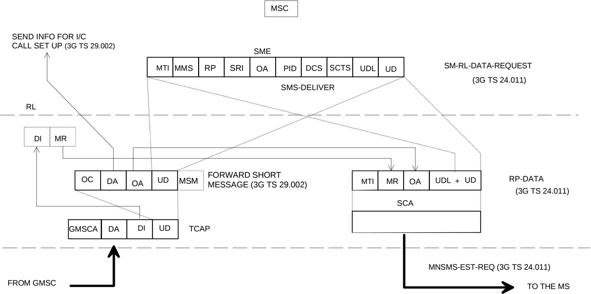
Figure C.3: Mobile terminated short message
