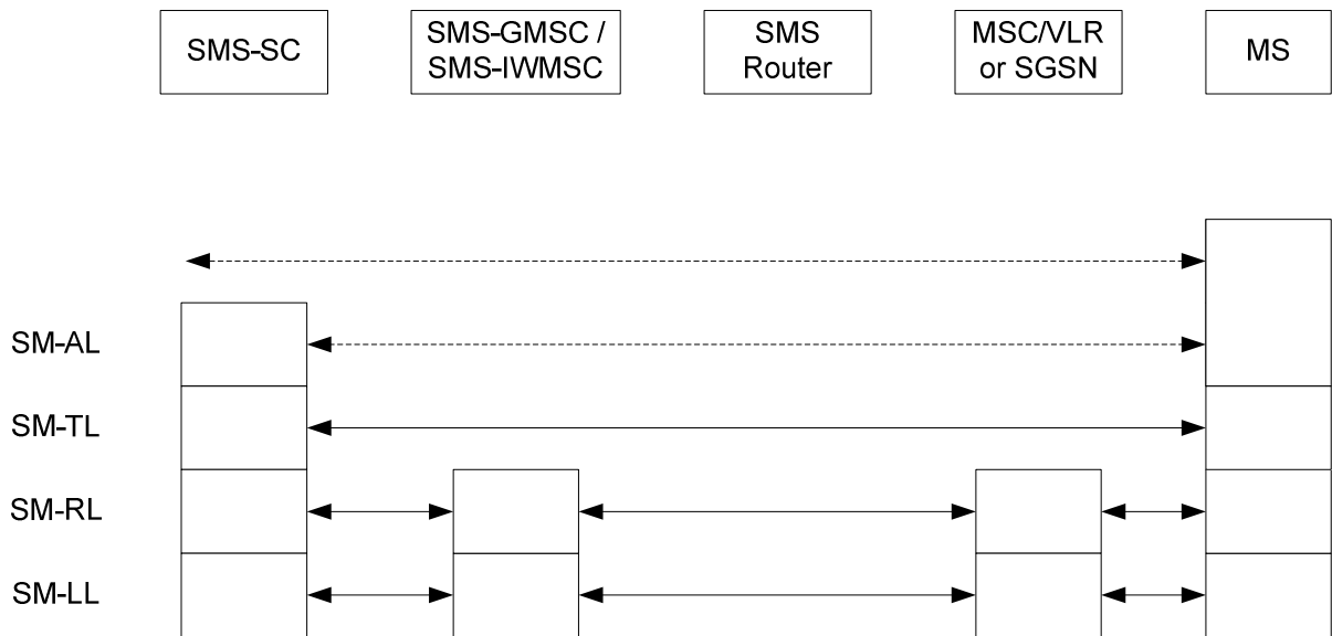
NOTE: The SMS Router is an optional functional entity, and is used only in the MT case. Figure 7: Protocol layer overview for the Short Message Service
