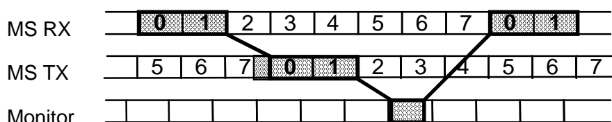
Figure 2: Double slot operation in the air interface
