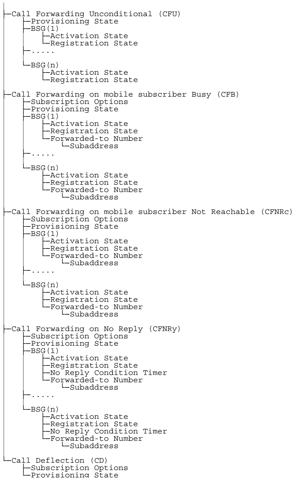
Figure 4: Forwarding Info
