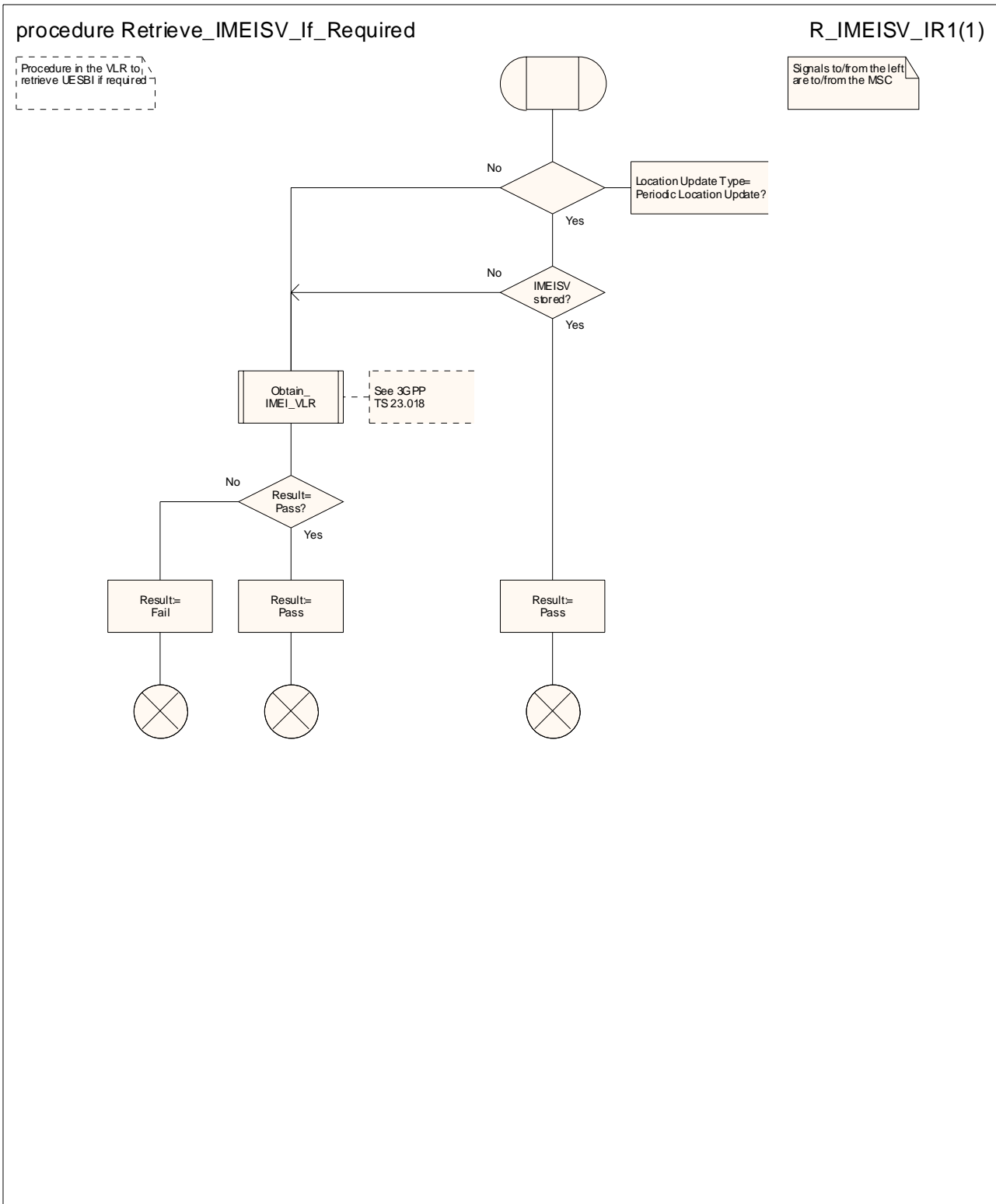
Figure 4.1.2.1A: Procedure Retrieve_IMEISV_If_Required
