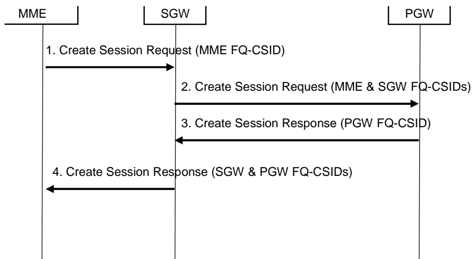
Figure 24-1: FQ-CSID establishment during the Attach or PDN establishment procedure
