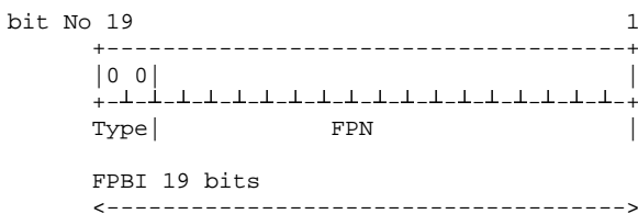
Figure 15: Structure of FPBI class A
