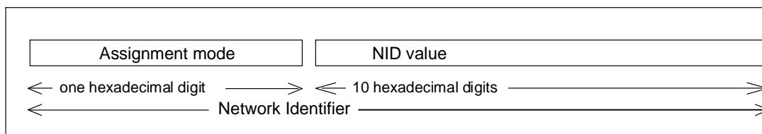
Figure 12.7.1-1: Network Identifier (NID)
