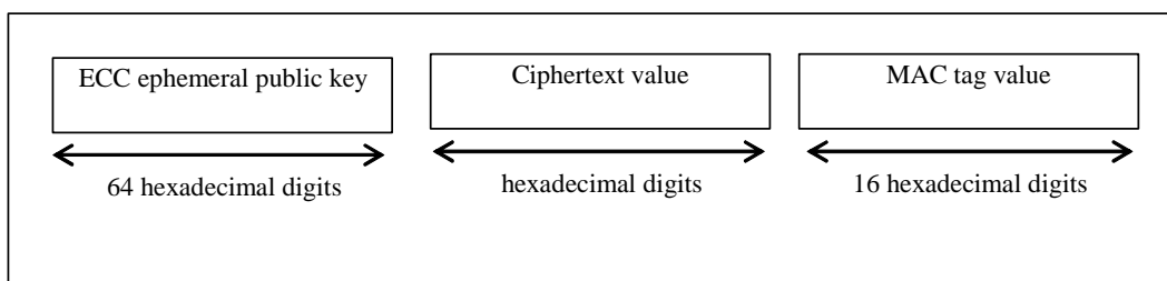
Figure 2.2B-3: Scheme Output for Elliptic Curve Integrated Encryption Scheme Profile A
