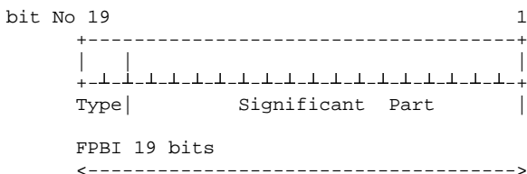
Figure 14: General structure of FPBI
