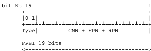
Figure 16: Structure of FPBI class B
