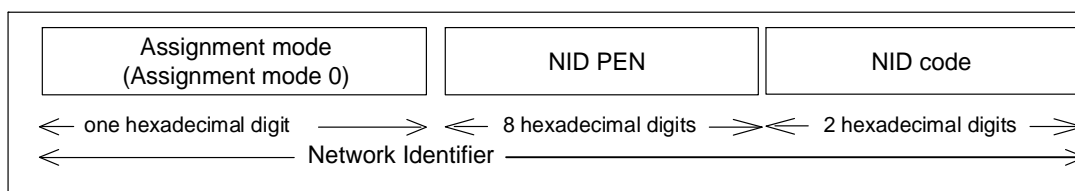
Figure 12.7.2-1: NID of assignment mode 0
