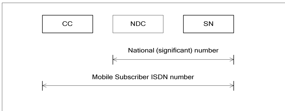
Figure 2: Number Structure of MSISDN
