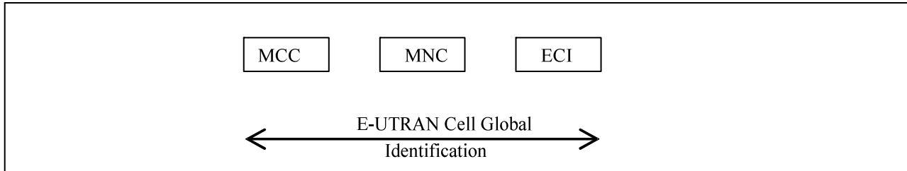
Figure 19.6.1: Structure of E-UTRAN Cell Global Identification
