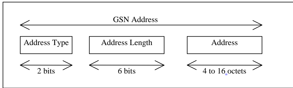
Figure 9A: Structure of GSN Address
