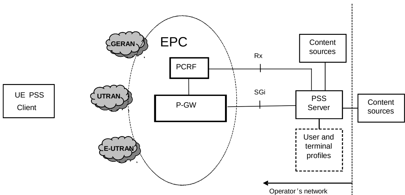
Figure 5.19-2: PSS Service Architecture for EPS
