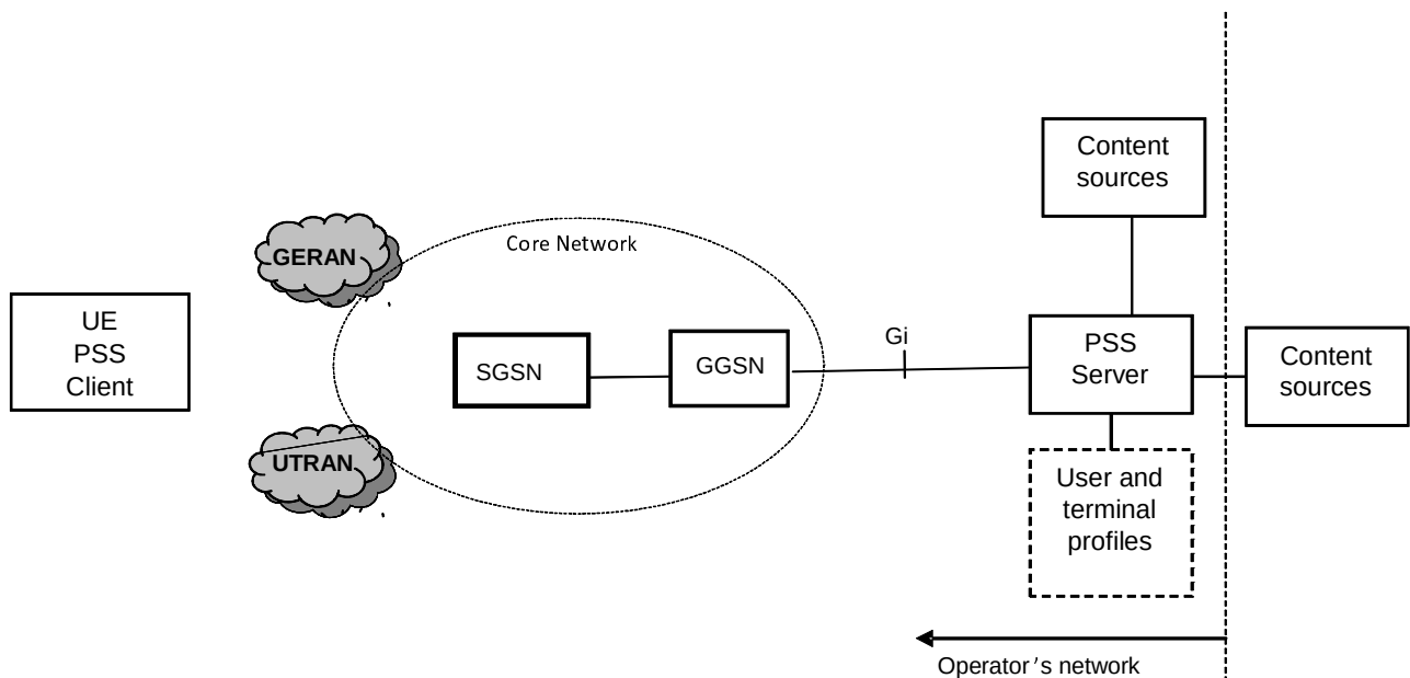
Figure 5.19-1: PSS Service Architecture for GPRS
