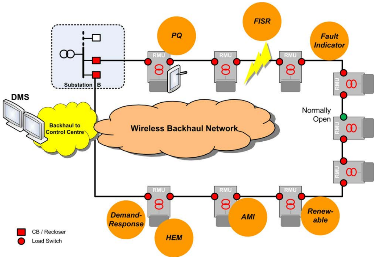
Figure D.4.1.0-1: Functional, topological sketch of a medium-voltage ring. AMI: advanced metering infrastructure; CB: circuit breaker; DMS: distribution management system; FISIR: fault isolation and system restoration; HEM: home energy manager; PQ: power quality; RMU: ring main unit.
