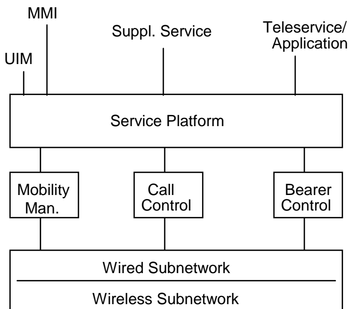
Figure 1: Service Architecture
