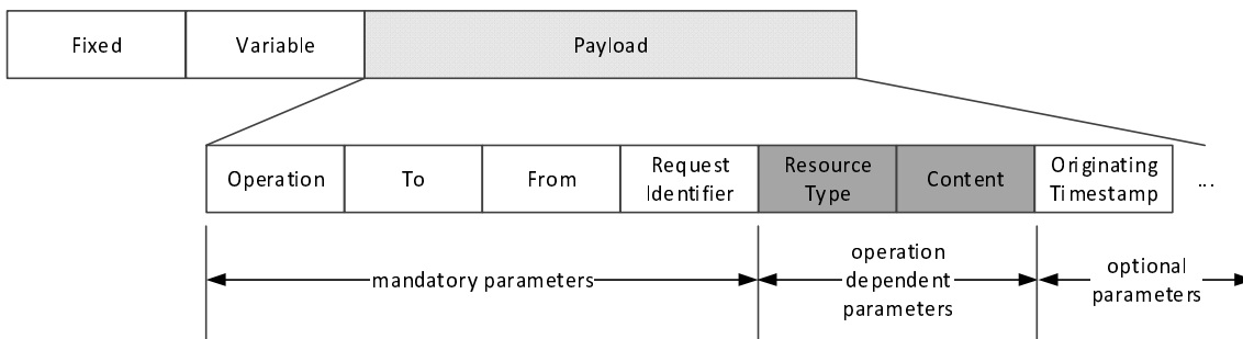
Figure 6.5.1-1: MQTT Request example
