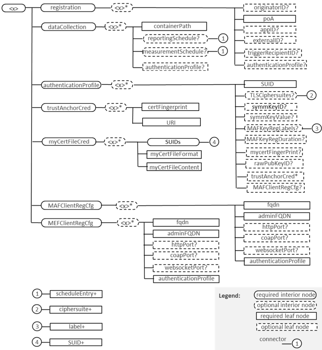
Figure 5.6.2-1: Structure of OMA-DM compatible M2M FieldDeviceConfig MO (MFDCMO)
