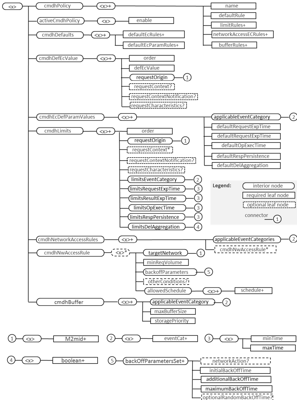
Figure 5.6.1-1: Structure of OMA-DM compatible M2M CMDH Policies MO (MCMMDHMO)
