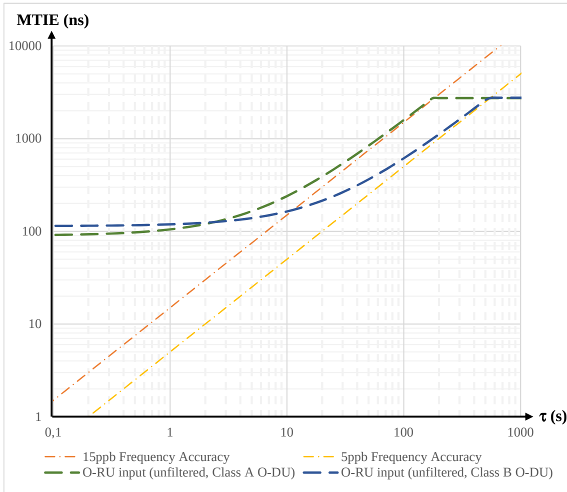
Figure H.2.4-4: MTIE limit at the input to an O-RU (LLS-C2)
