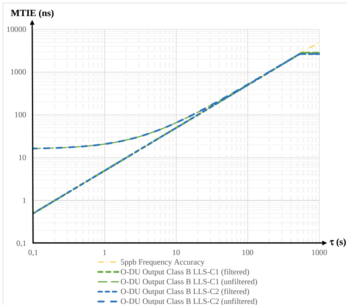
Figure H.2.4-3: MTIE Limit at the output of an O-DU Class B
