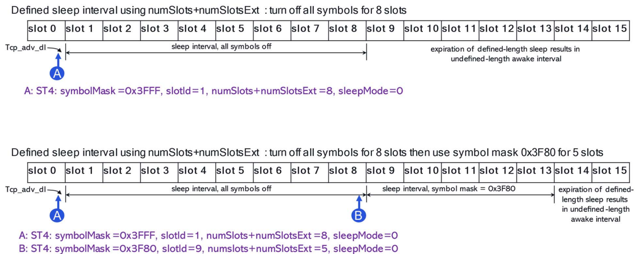
Figure 16.11-1: Timing diagram showing defined sleep intervals, sleepMode = 0
