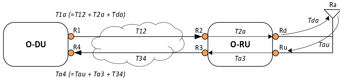
Figure 4.7-1: Definition of reference points including external antenna delay
