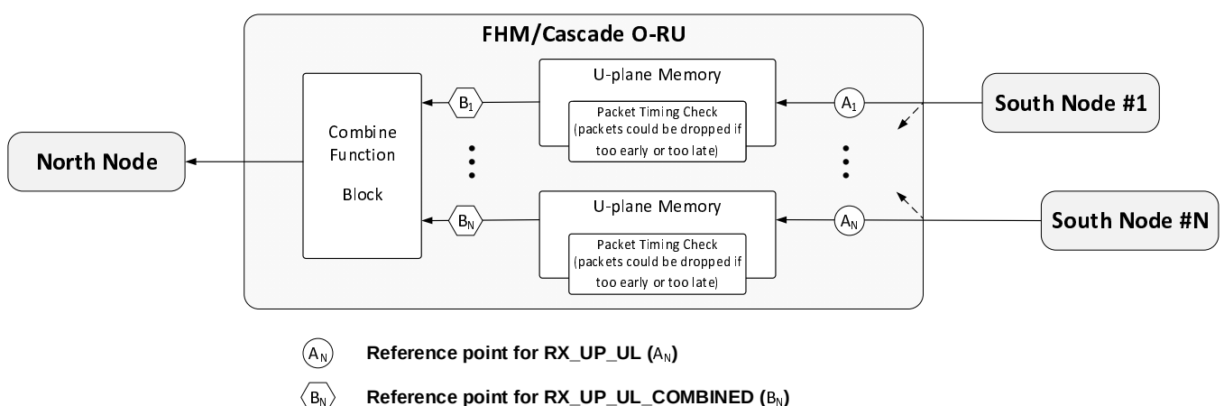
Figure 9.1-1: Reference Point Model of Performance Counter for UL combining Function
