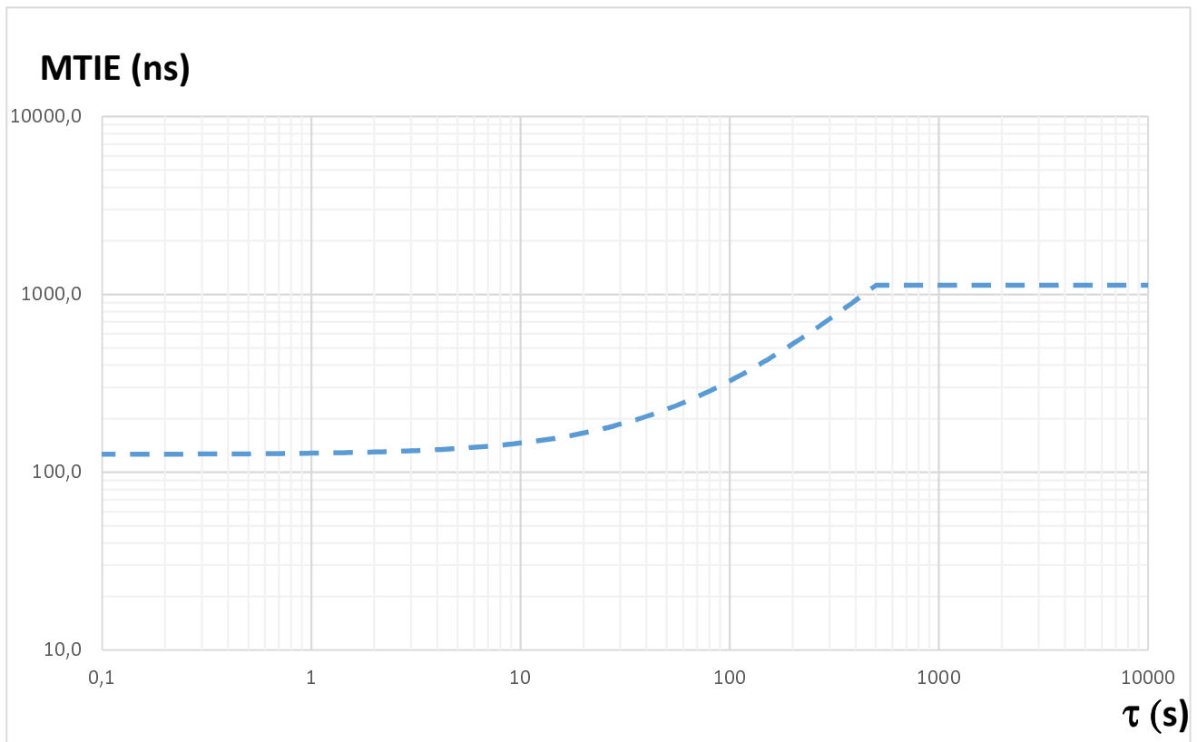
Figure H.2.5-1: MTIE limit at the input to an O-RU in LLS-C3
