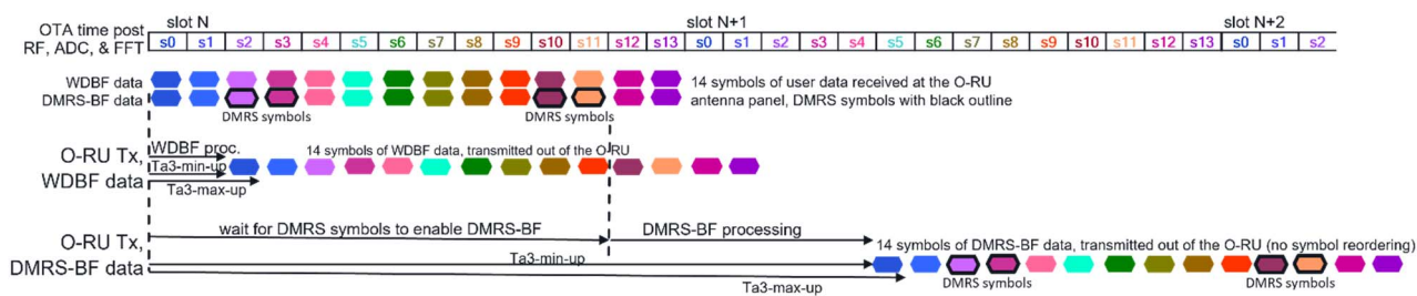
Figure 12.6.1.4-1: Comparison of WDBF delay profile versus DMRS-BF delay profile
