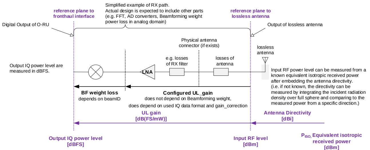
Figure 8.1.3.2.1-3: Details of UL gain
