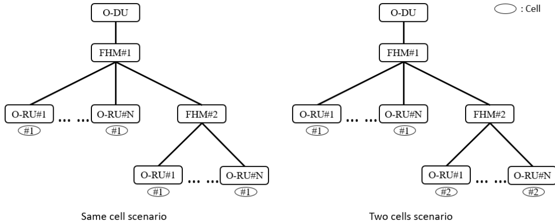
Figure 13.7.1-1: Cascade-FHM mode
