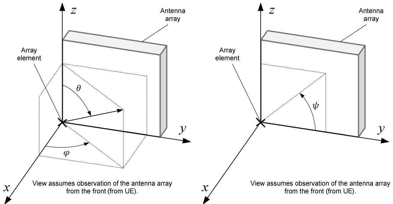
Figure 12.5.2-1: Array Coordinate System
