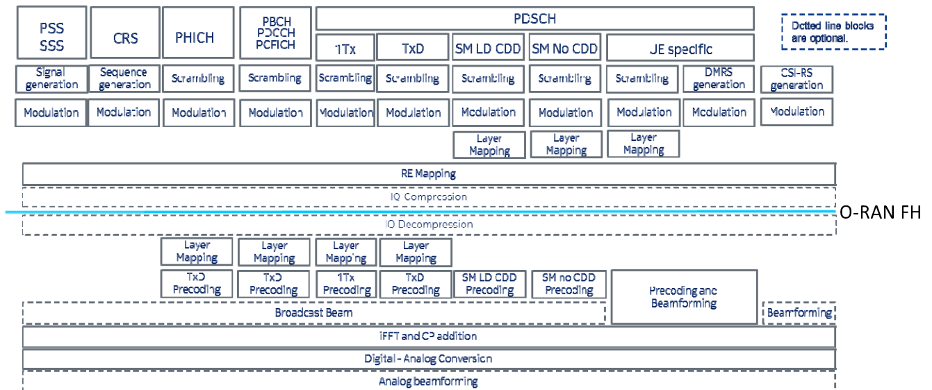
Figure 4.2.2.1-2: Lower layer DL split description, LTE, Category B O-RUs
