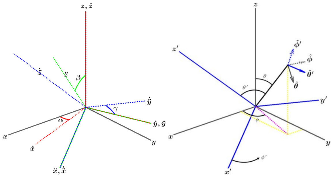
Figure F-2: Orienting the LCS (blue) with respect to the GCS (grey) by a sequence of 3 rotations (left); Definition of spherical coordinates and unit vectors in both the GCS and LCS (right)
