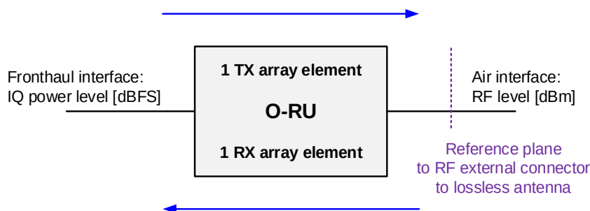
Figure 8.1.3.2.1-1: DL and UL gain over fronthaul interface
