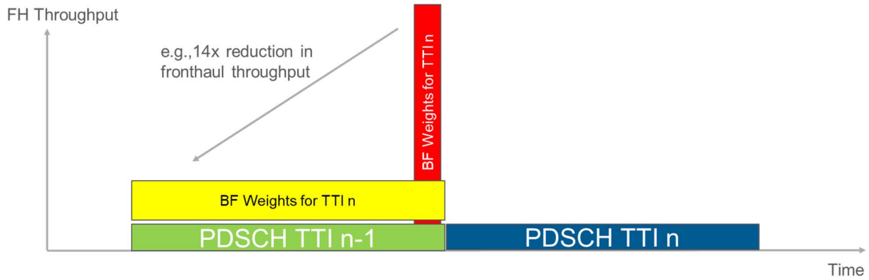
Figure 4.4.2.2-1: Example of the benefit of using a longer C-Plane tx/rx window compared to the U-Plane windows
