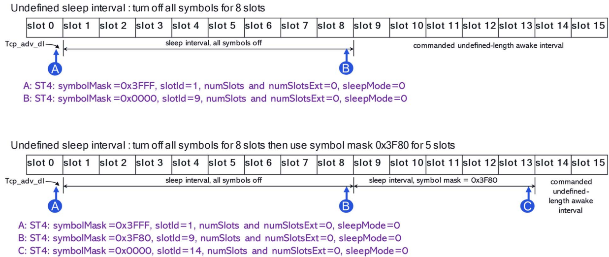
Figure 16.11-2: Timing diagram showing undefined sleep intervals, sleepMode = 0
