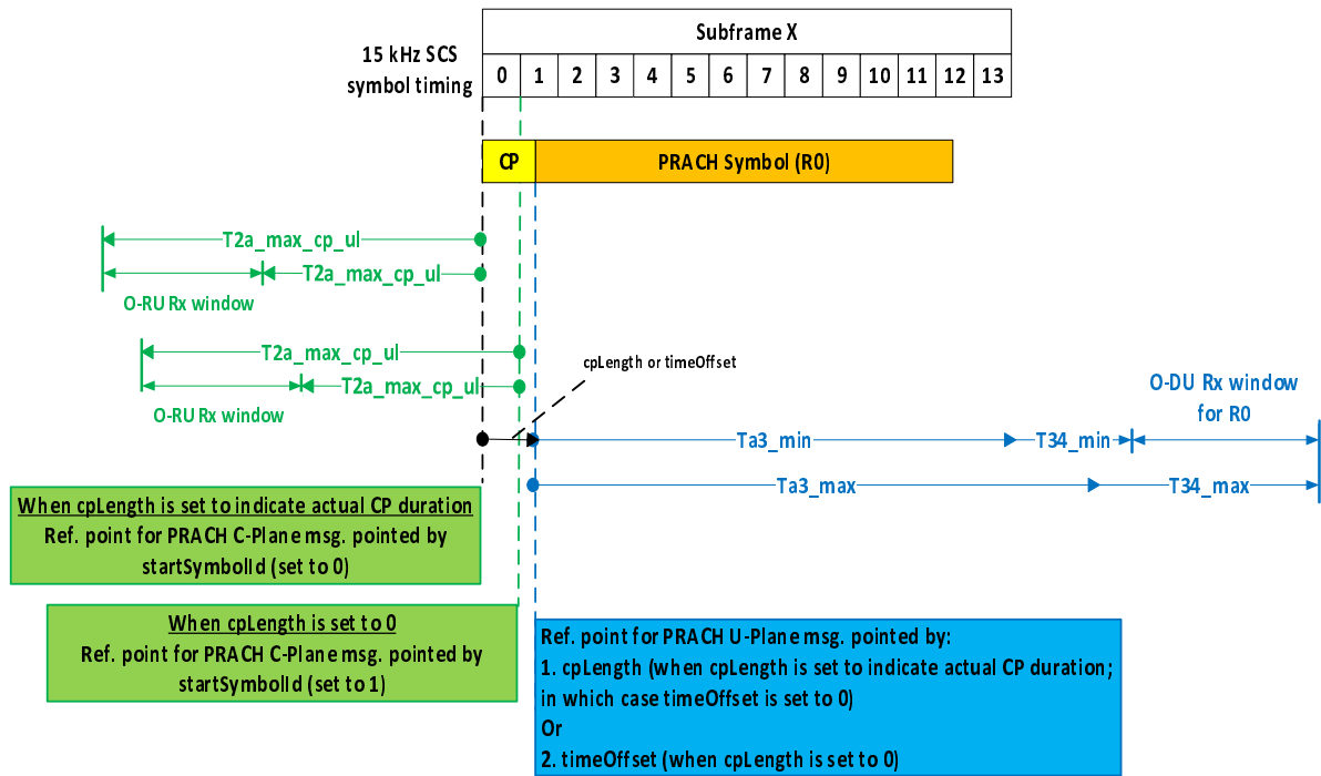
Figure 4.4.3-3: Timing relations for PRACH (Example 1: PRACH Format 0)
