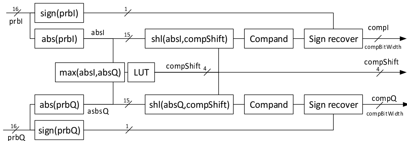
Figure A.3.1-1: \mu -Law compression algorithm
