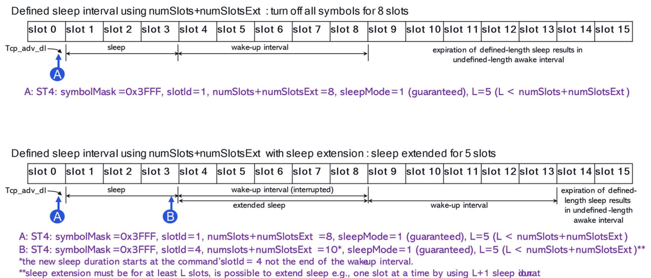
Figure 16.11-3: Timing diagram showing defined sleep intervals, guaranteed wake-up durations
