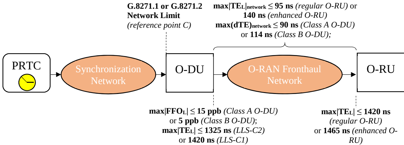
Figure H.2.4-1: Simplified view of LLS-C1 and LLS-C2 configurations, with network limits
