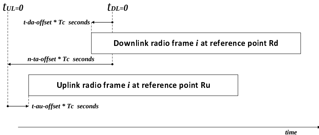
Figure 4.8.1-2 : Uplink-Downlink Timing Relation for O-RU handling external antenna delay
