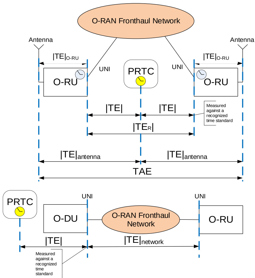
Figure 11.2.5.5-1: Definition of |TE| and TAE and UNI
