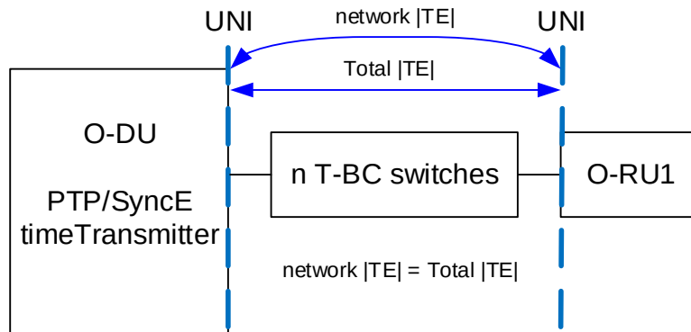
Figure H.2.3-1: Clock chain model for analysis for two paths
