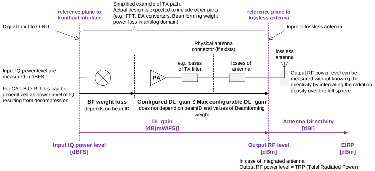
Figure 8.1.3.2.1-2: Details of DL gain
