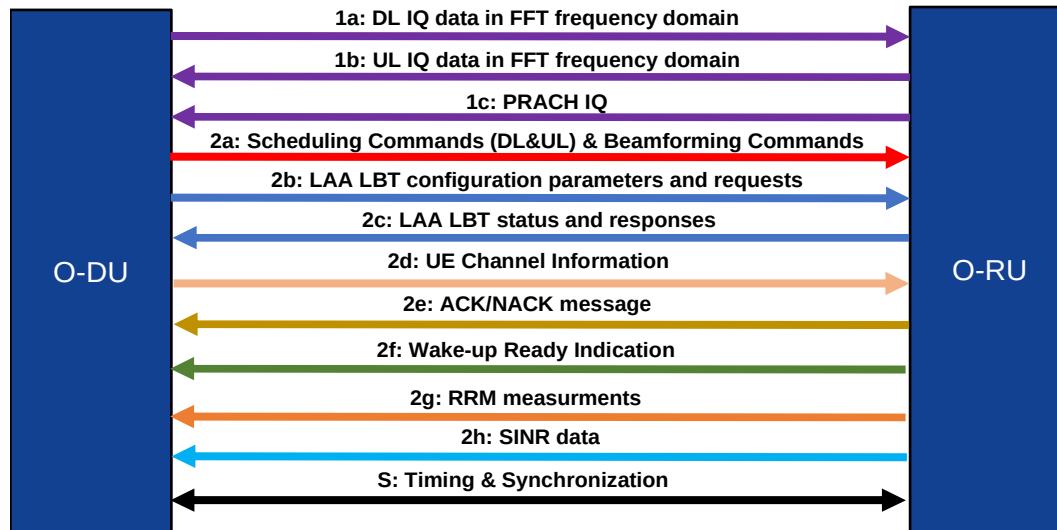
Figure 4.3-1: Lower layer fronthaul data flows
