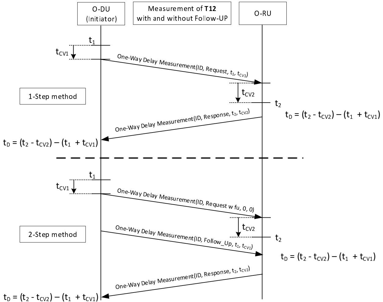
Figure 4.4.4-1: eCPRI One-Way Delay T12 Measurement procedure
