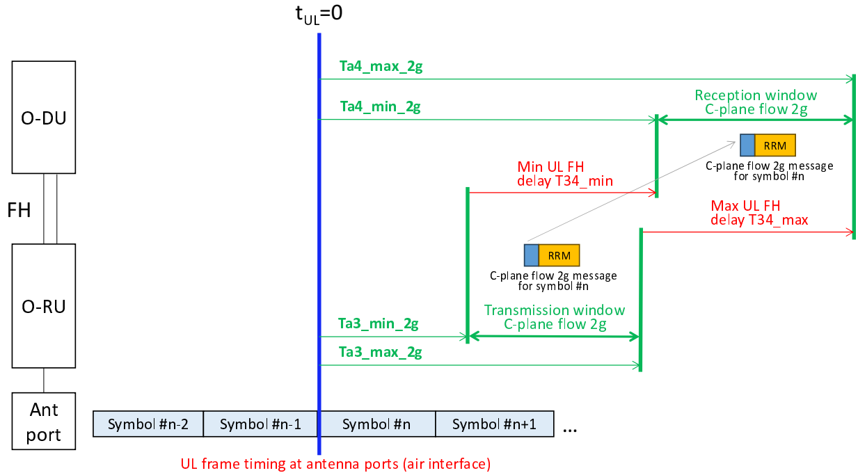
Figure 4.4.3-7: Timing relations for C-Plane data flow 2g (RRM Measurements)
