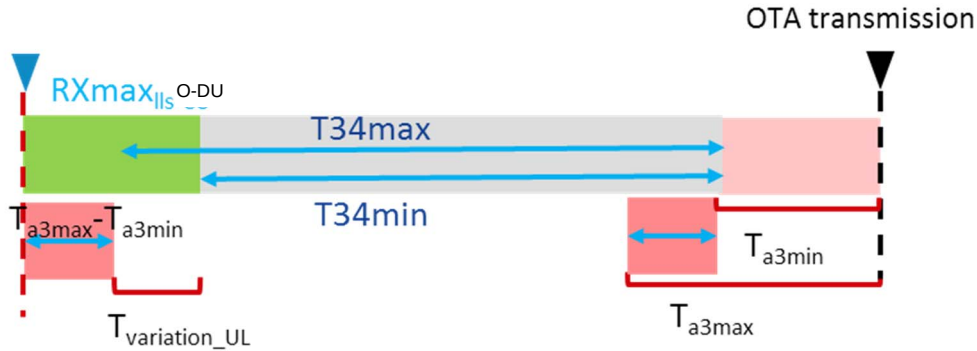
Figure 4.4.5-3: Uplink transport variation
