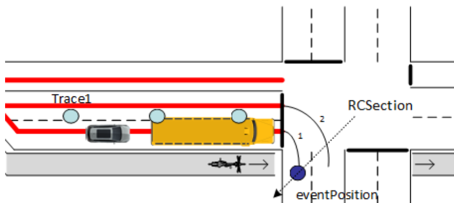
Figure B.7: Scenario where a road configuration description in terms of mapemConfiguration using MAPEM connections is useful
