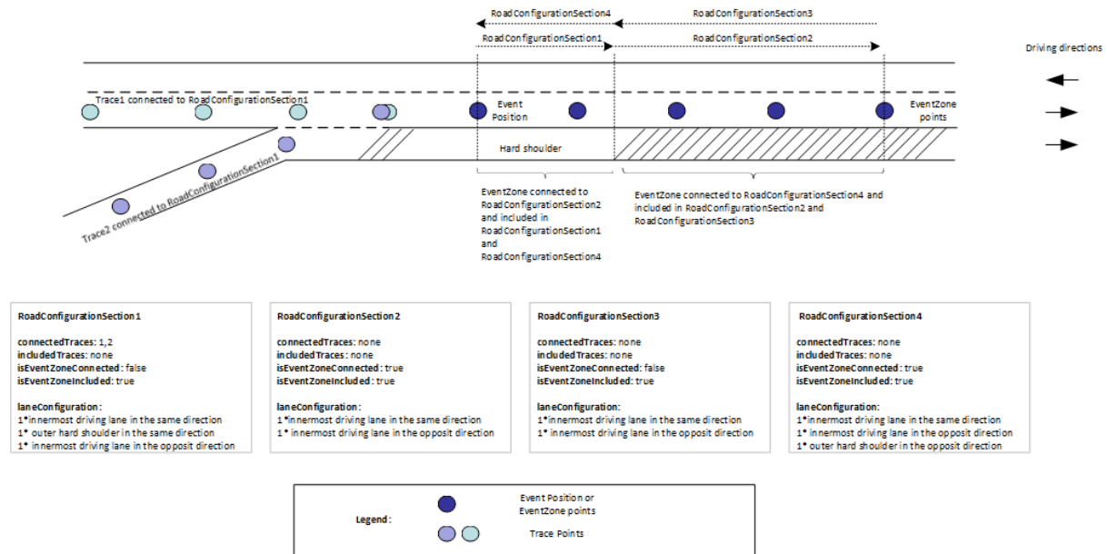
Figure B.3: Visual explanation of the RCC elements
