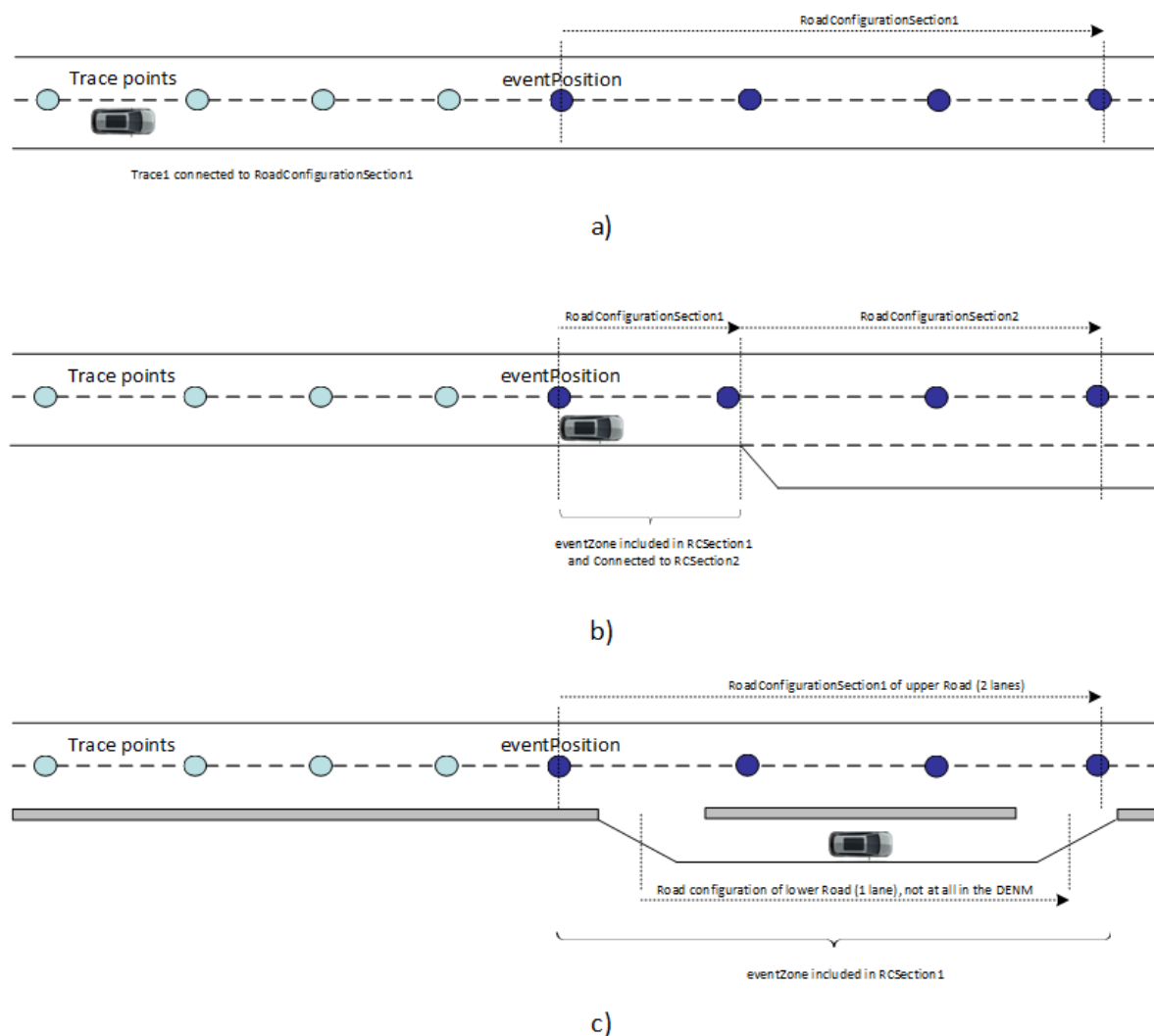
Figure B.4: Examples of traces and EventZone , connected and included in RoadConfigurationSections
