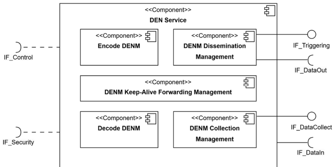
Figure 3: DEN service component diagram
