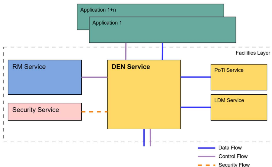
Figure 2: DEN service and logical interfaces
