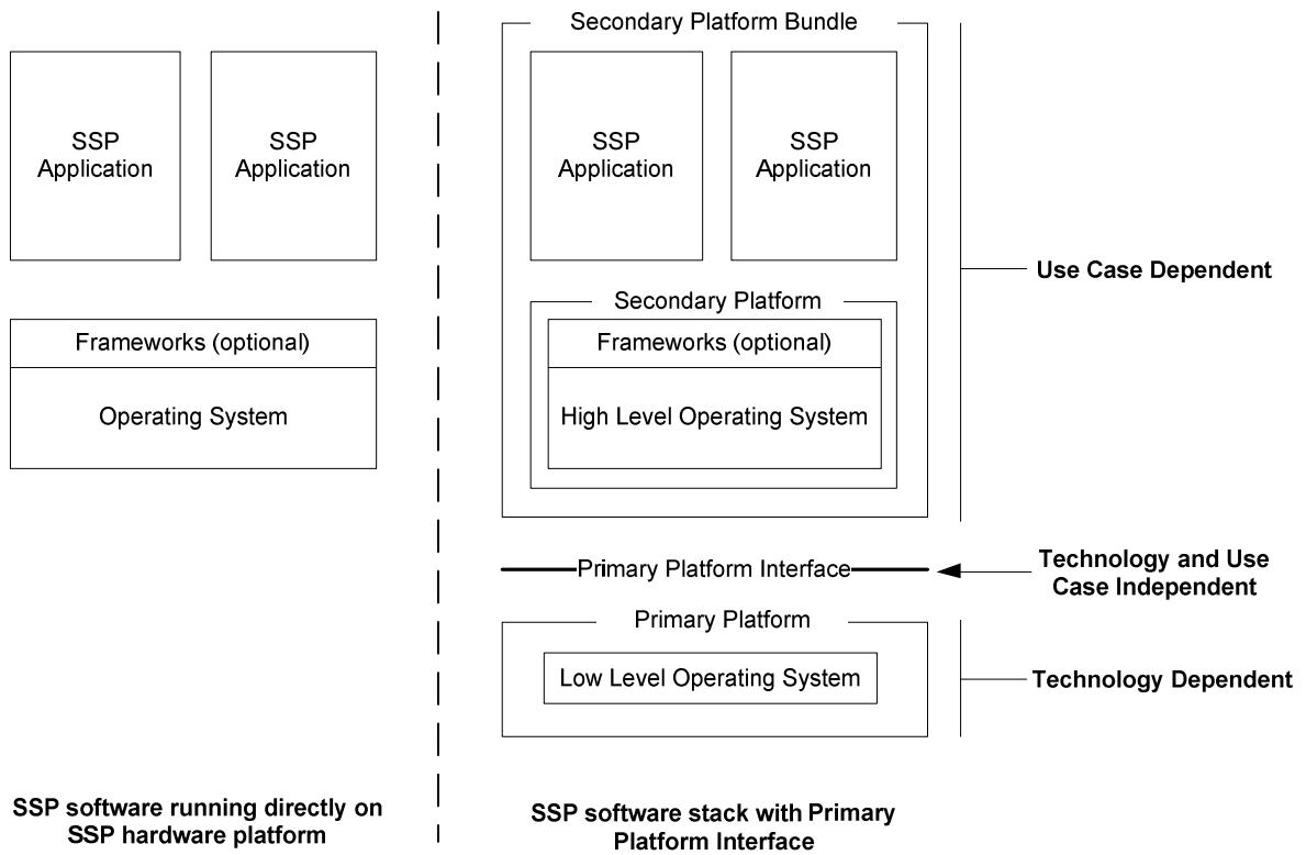
Figure 5.1: SSP software architectures
