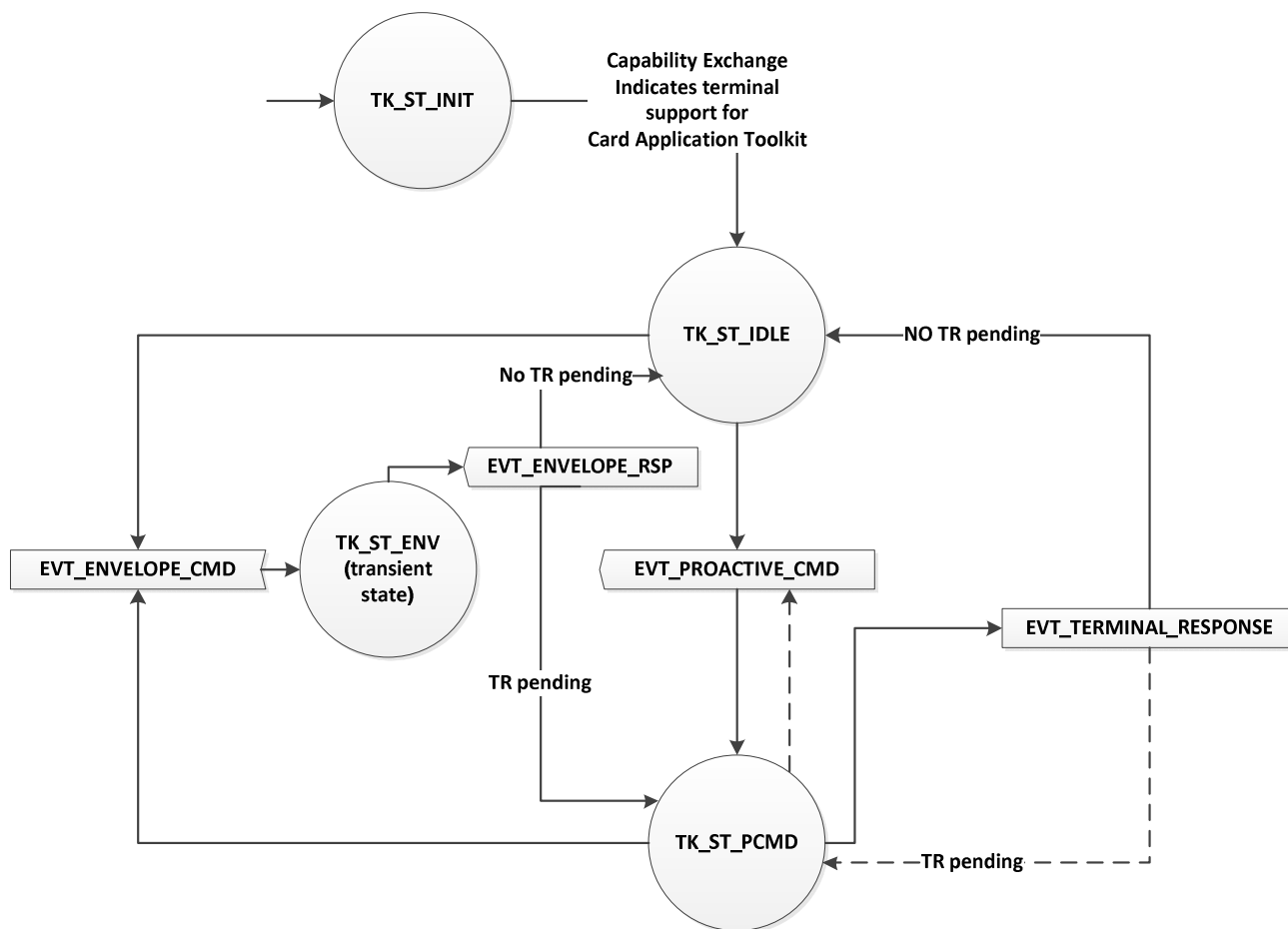
Figure 10.10: State transitions
