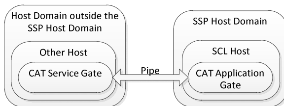
Figure 10.8: Platform supporting the CAT service
