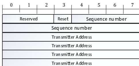
Figure 6.3.3.4-1: RD Broadcasting Header
