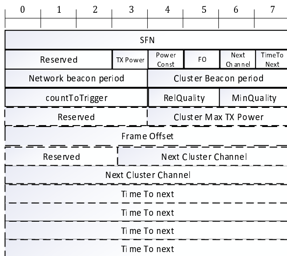
Figure 6.4.2.3-1: Cluster Beacon Message IE
