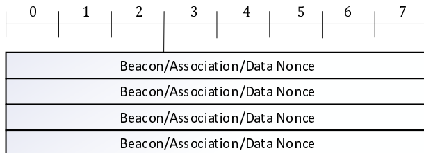
Figure 6.4.3.19-1: Access Token IE
