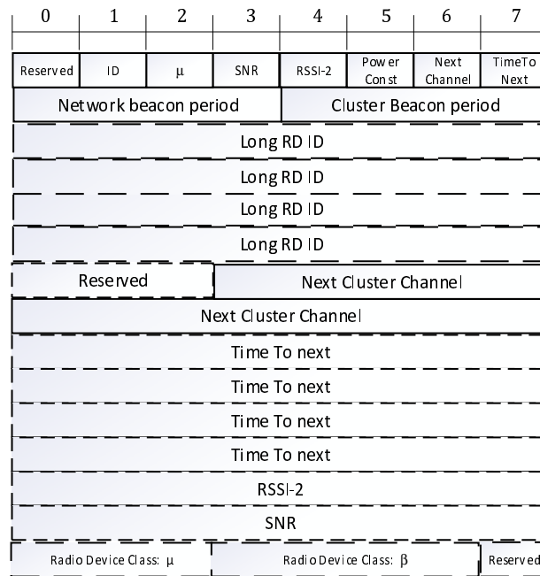
Figure 6.4.3.6-1: Neighbouring IE
