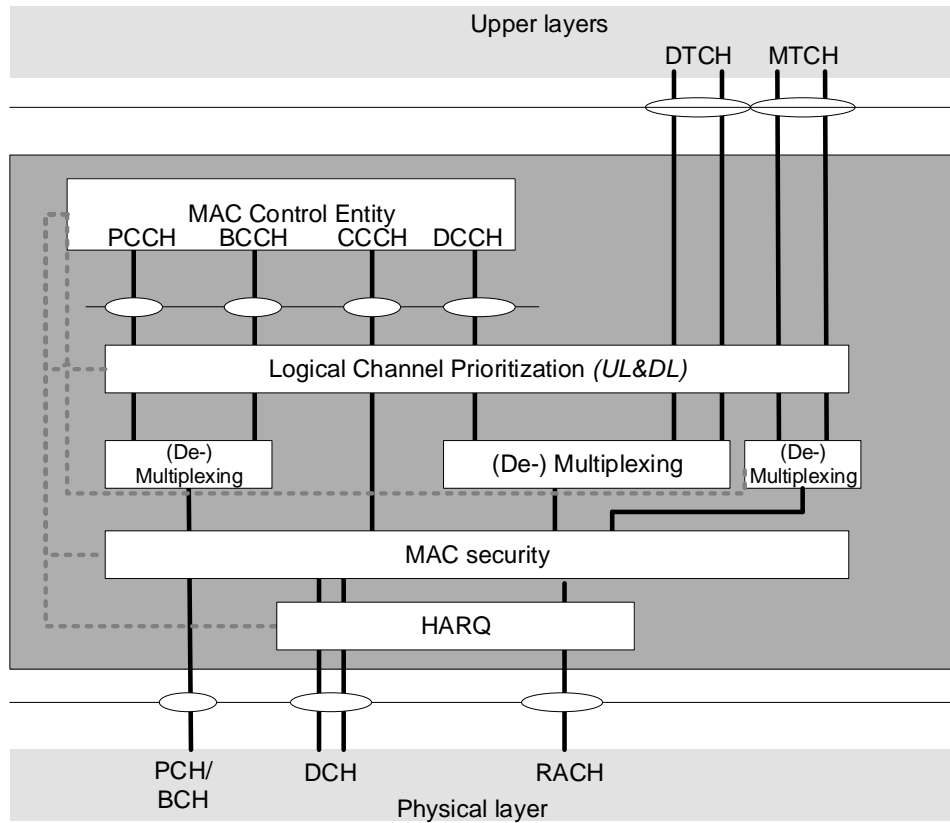
Figure 4.2.2-1: MAC structure overview
