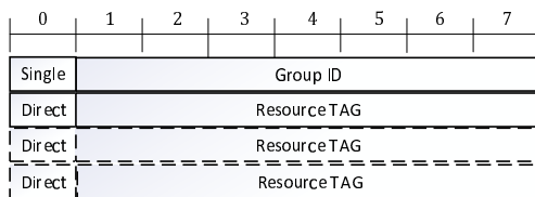
Figure 6.4.3.9-1: Group Assignment IE
