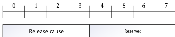
Figure 6.4.2.6-1: Association Release Message IE
