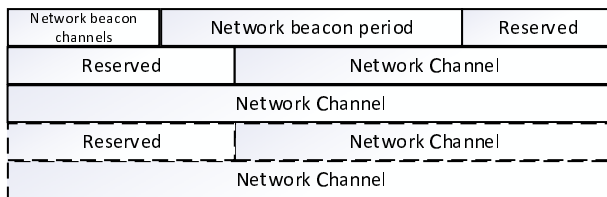
Figure 6.4.2.10-1: Joining Beacon message IE
