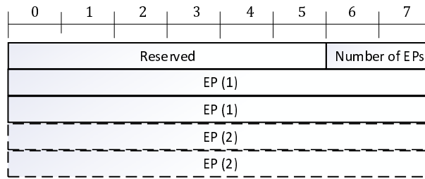
Figure 6.4.3.17-1: Joining Information IE
