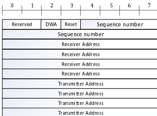
Figure 6.3.3.3-1: Unicast Header
