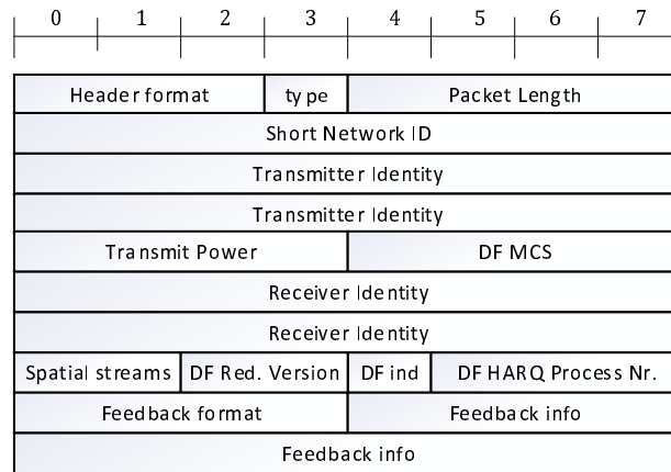
Figure 6.2.1-2: Physical Layer Control Field: Type 2
