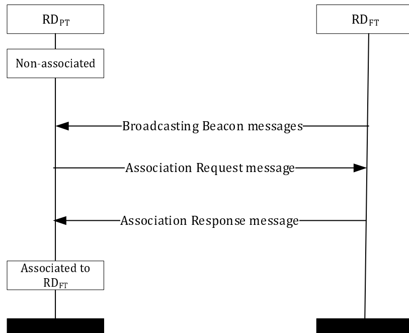
Figure 5.8.1-1: Association signalling
