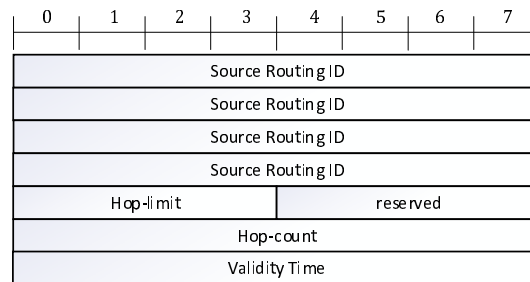
Figure 6.4.3.16-1: Source Routing IE
