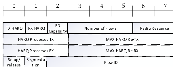
Figure 6.4.2.8-1: Reconfiguration Request Message IE
