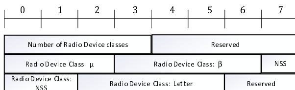
Figure 6.4.3.5-1: RD Capability IE
