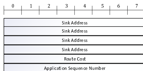
Figure 6.4.3.2-1: Route Info IE
