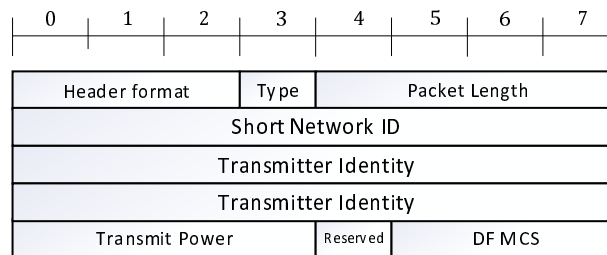
Figure 6.2.1-1: Physical Layer Control Field: Type 1
