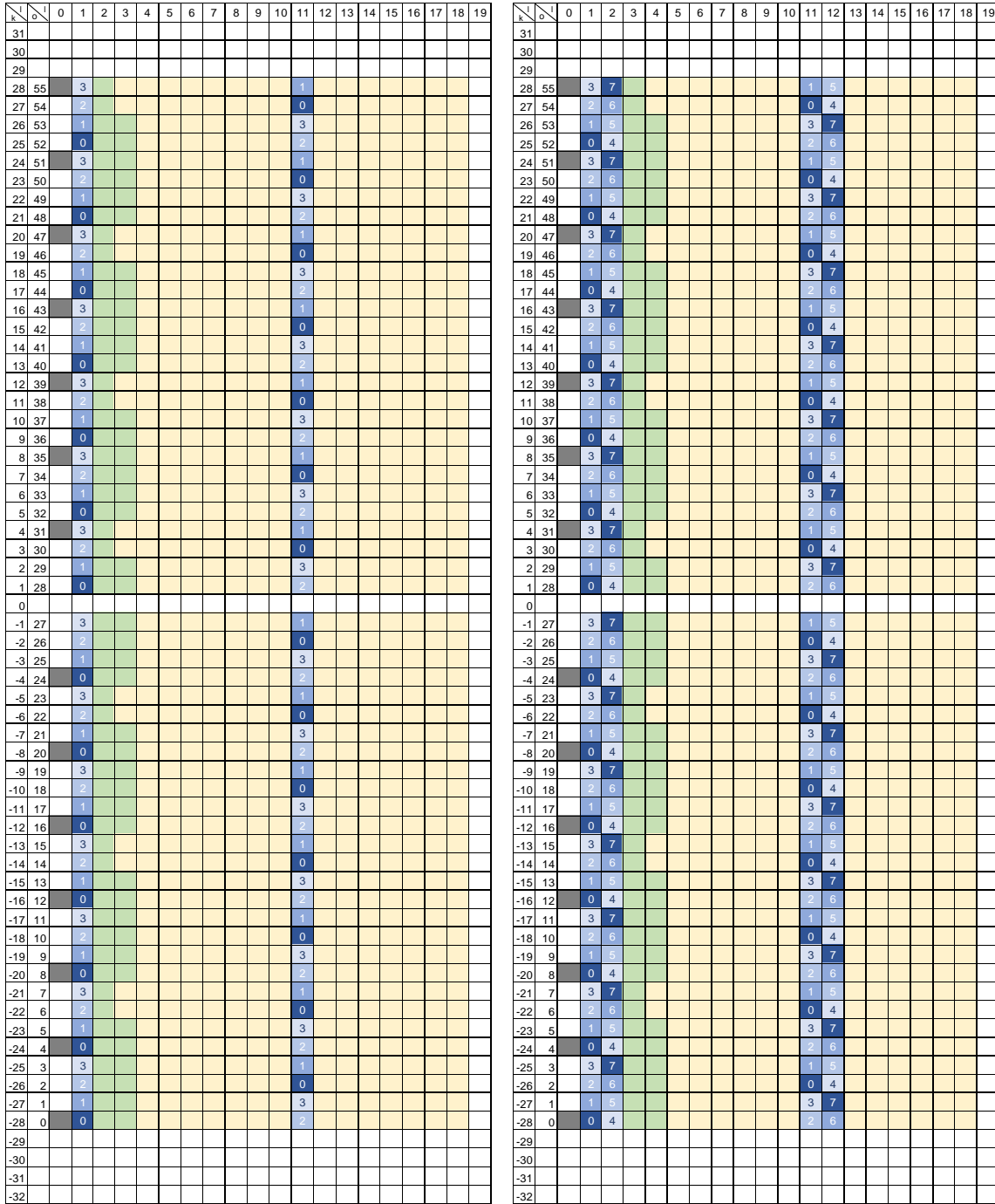
d) Transmission from four effective antennas of four subslots duration e) Transmission from eight effective antennas of four subslots duration 3 2 1 0 Synchronization Training Field Allocation Demodulation Reference Signal Allocation Physical Control Channel Allocation Physical Data Channel Allocation Unallocated Guard or Empty Resource
