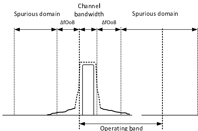
Figure 6.5.1-1: Transmitter RF spectrum
