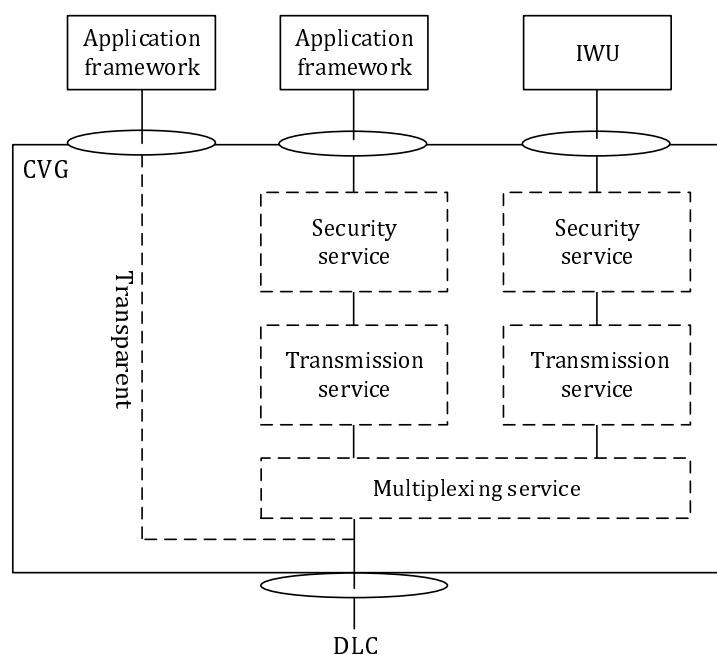
Figure 6.6.1-1: CVG architecture
