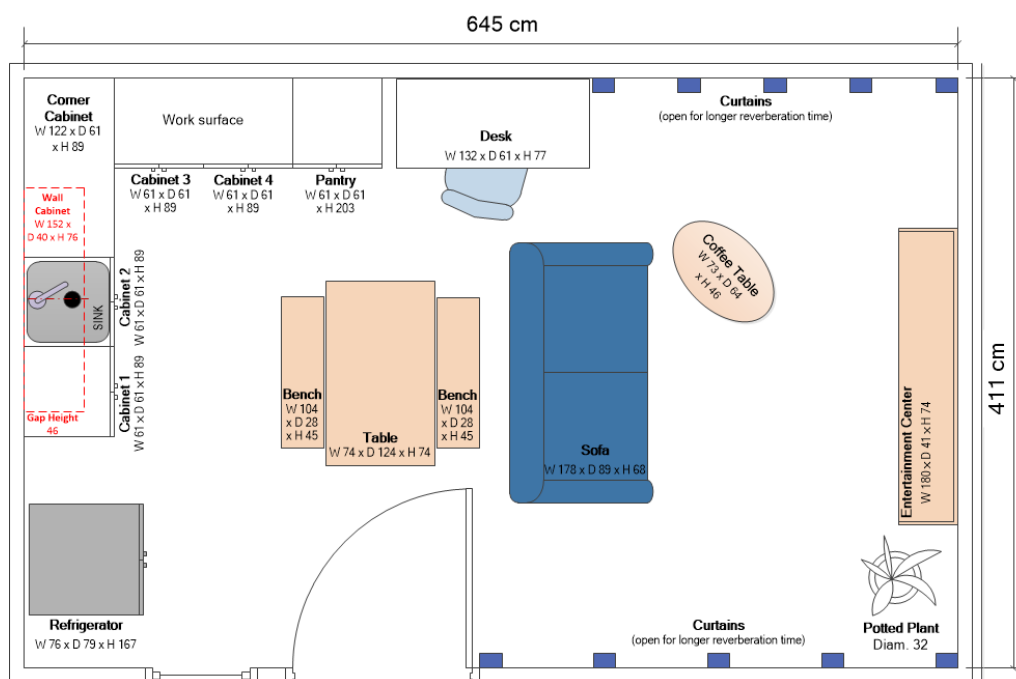
Figure B.2: Acoustic condition 2 home-like test environment layout (dimensions are in cm)
