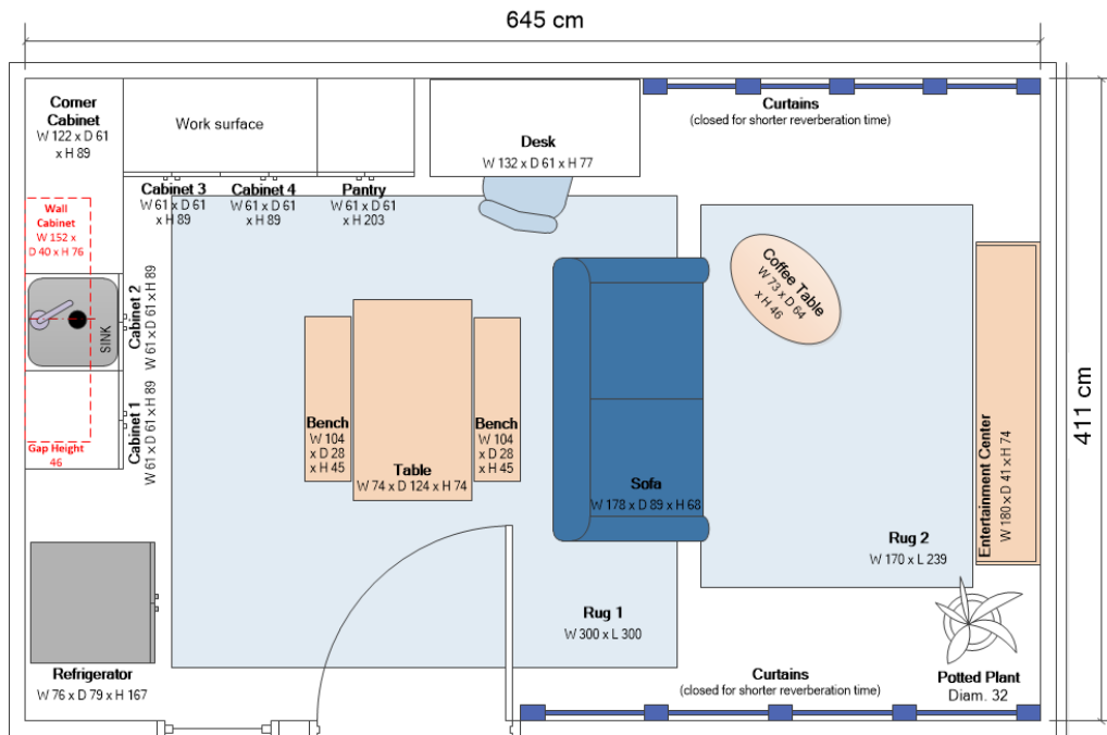
Figure B.1: Acoustic condition 1 home-like test environment layout (dimensions are in cm)
