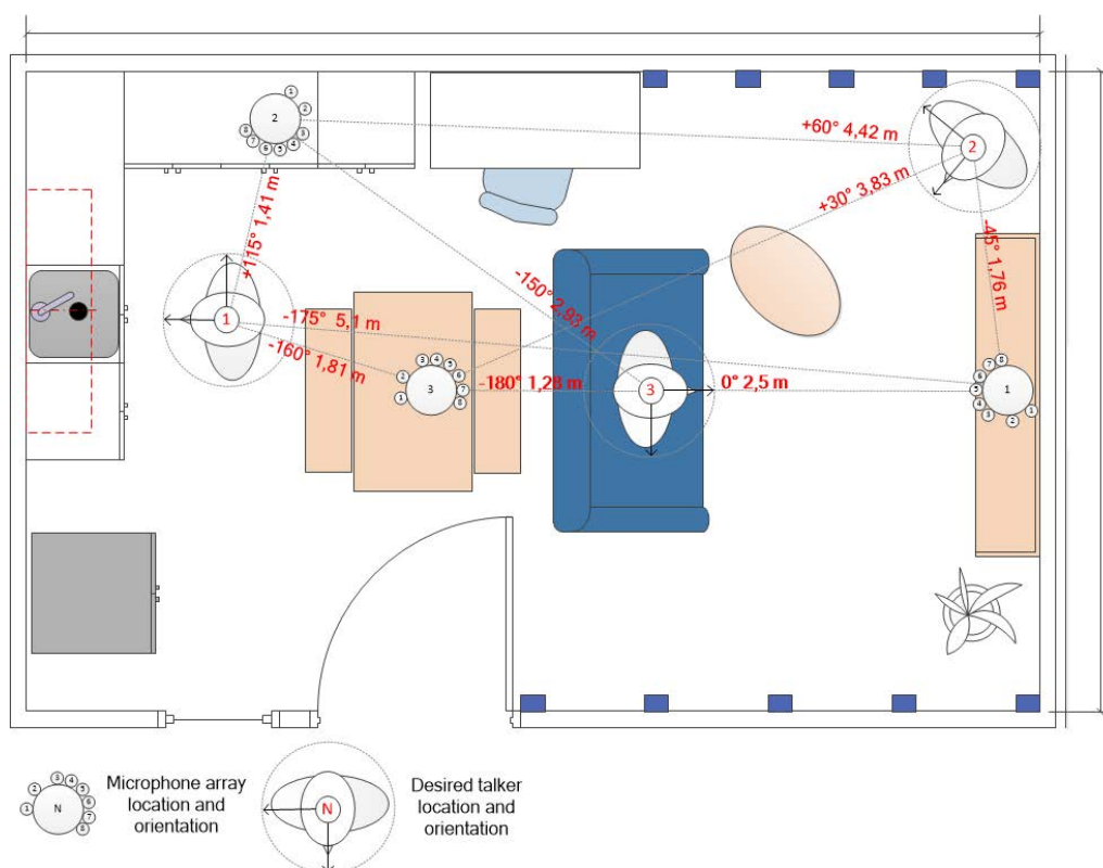
Figure B.3: Desired talker and microphone array (DUT) positions and orientations
