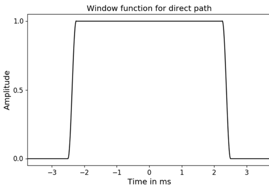
Figure 3: Window function for extracting the direct path from the impulse responses (time scale relative to maximum position of impulse response)
