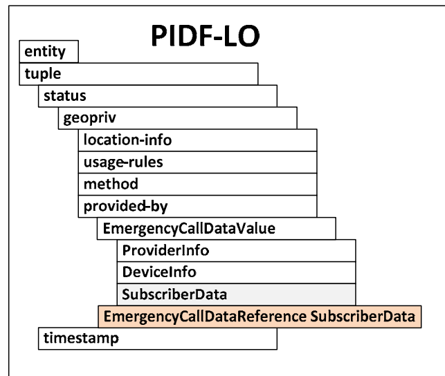
Figure 19: PEMEA PIDF-LO Structure
