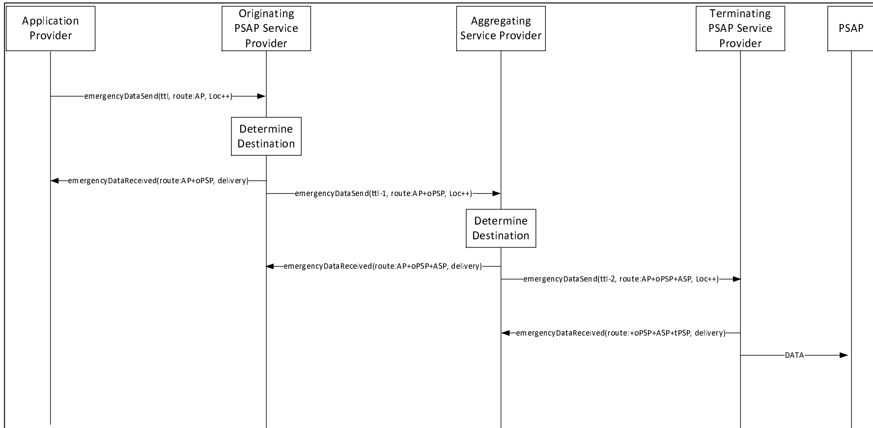
Figure 9: Ps routing flow
