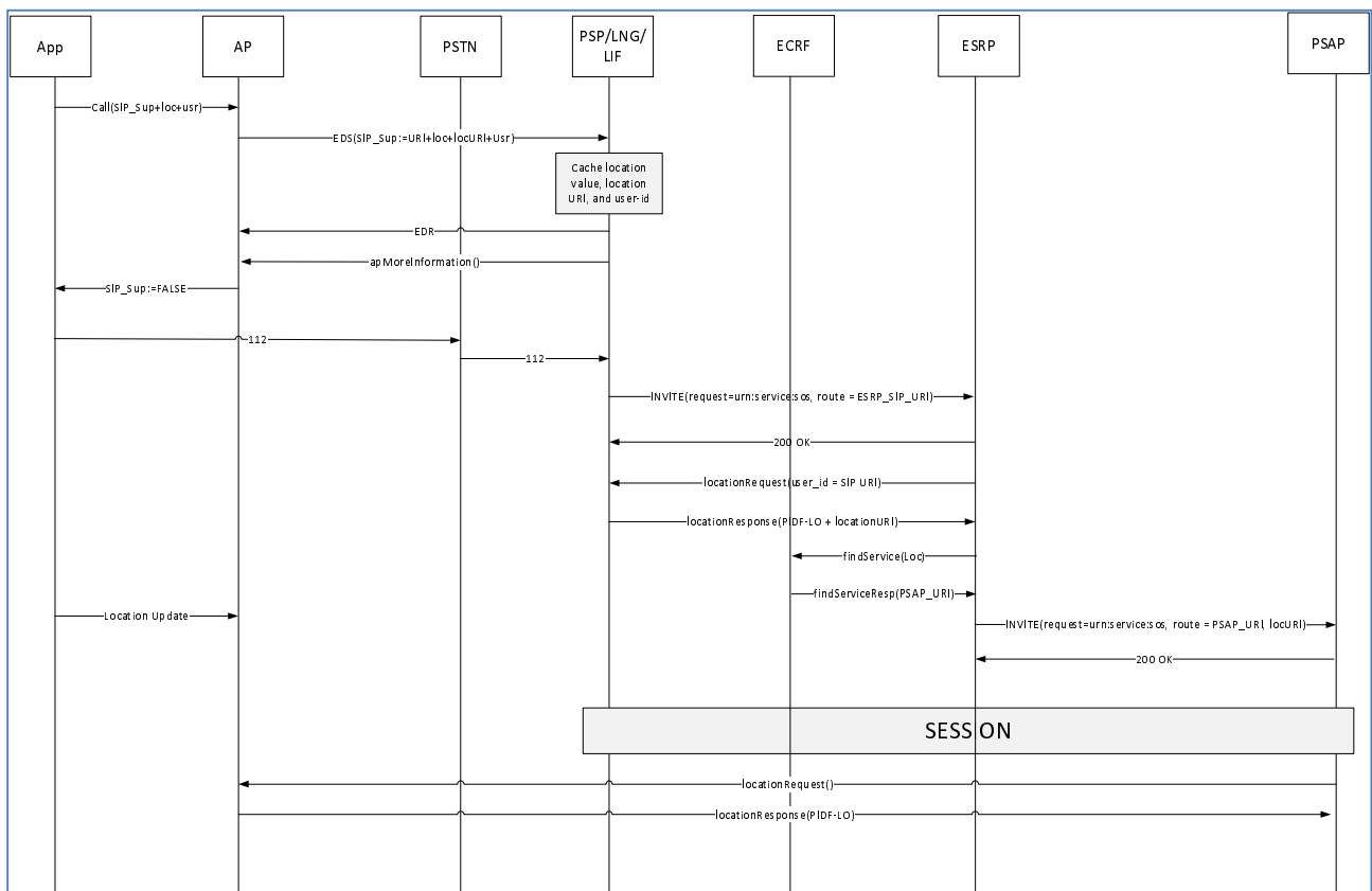
Figure 11: PEMEA alignment with ETSI TS 103 479 [i.1] for legacy calls
