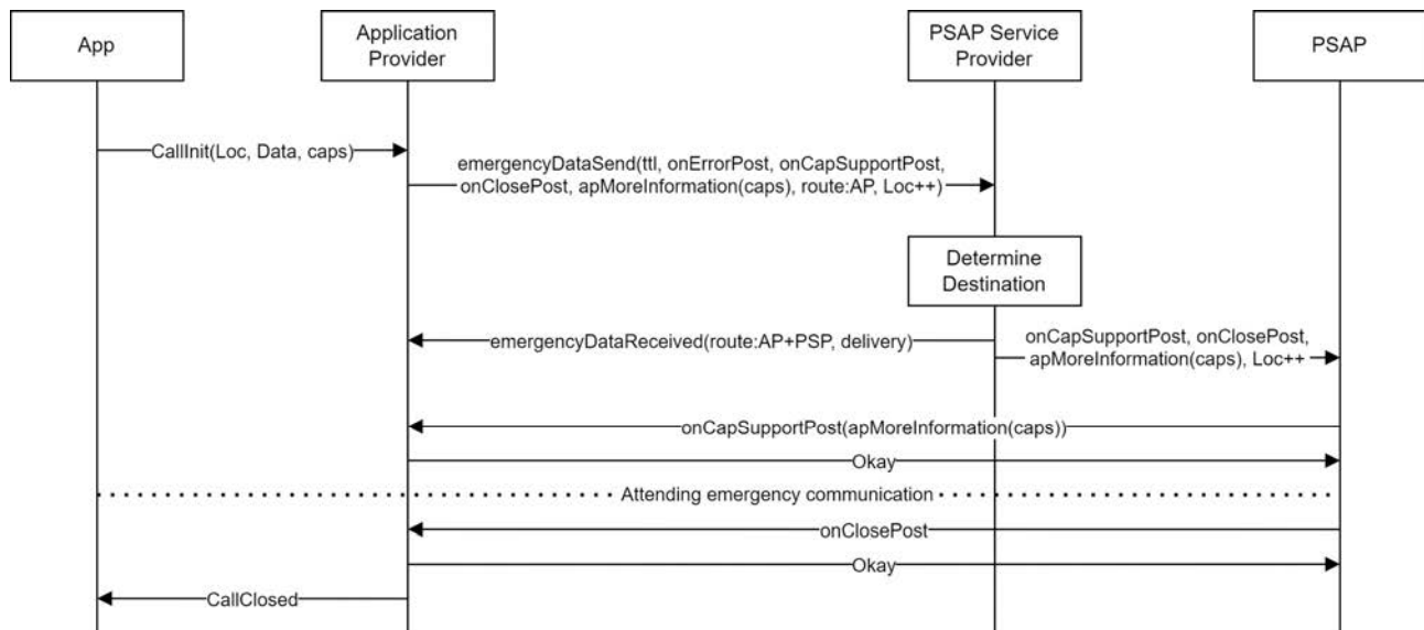
Figure 15: onClosePost message sequence
