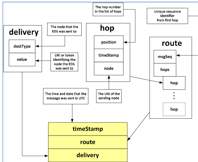
Figure 17: emergencyDataReceived message structure
