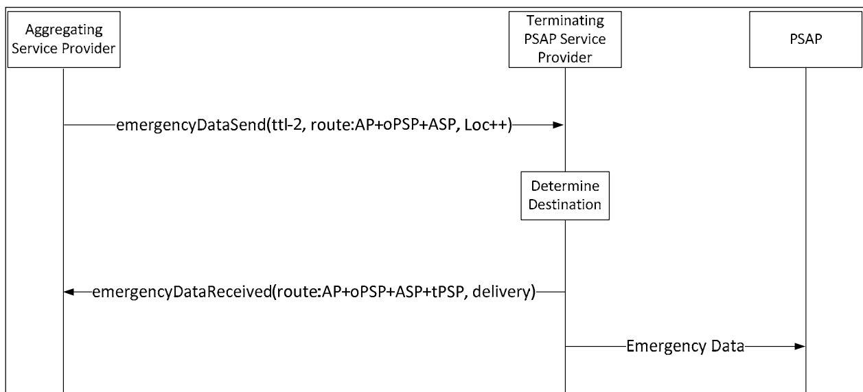
Figure 7: Pr basic message flow
