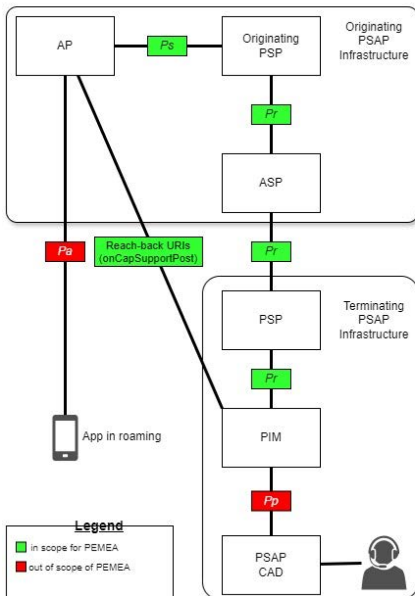
Figure 2: PEMEA roaming scenario
