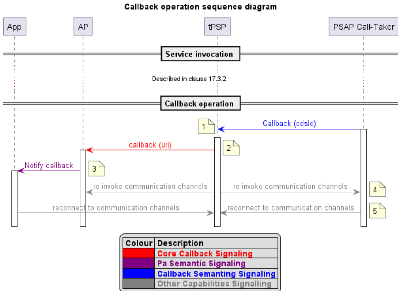
Figure 21: PEMEA Callback operation sequence diagram
