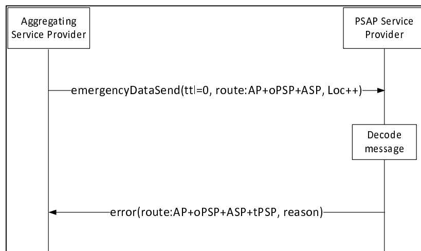
Figure 8: Pr error flow
