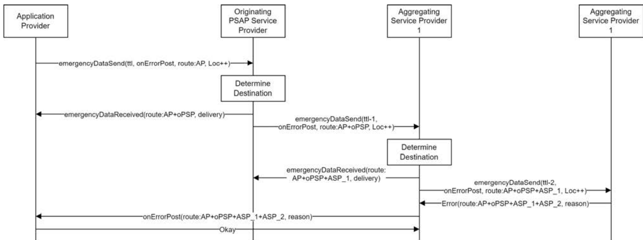
Figure 13: onErrorPost message flow
