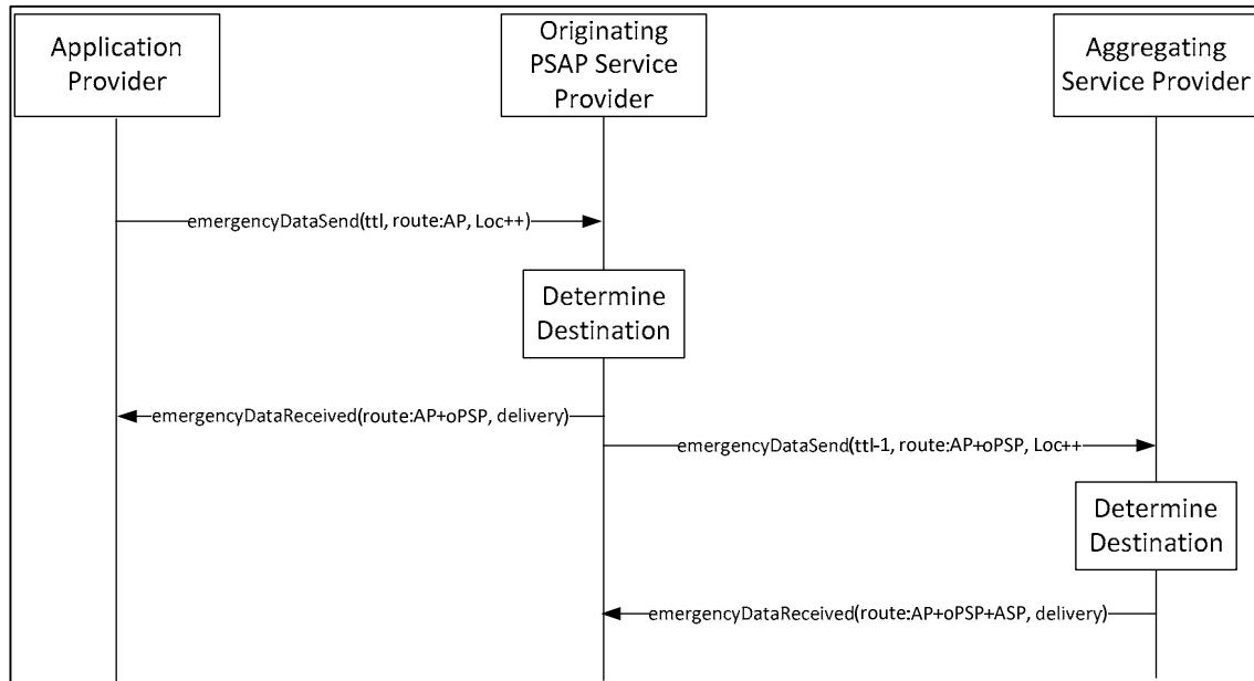
Figure 6: Ps routing flow
