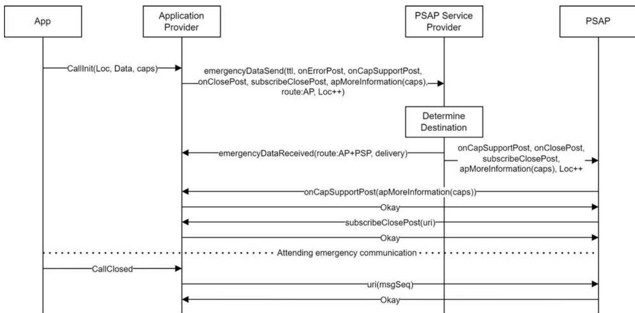
Figure 16: subscribeClosePost message sequence
