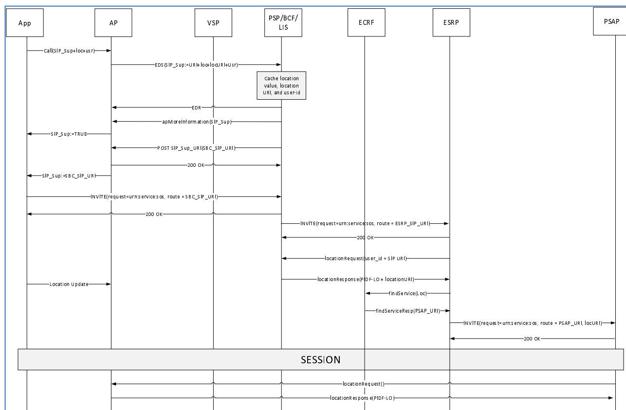
Figure 10: PEMA alignment with ETSI TS 103 479 [i.1] for SIP-originated calls
