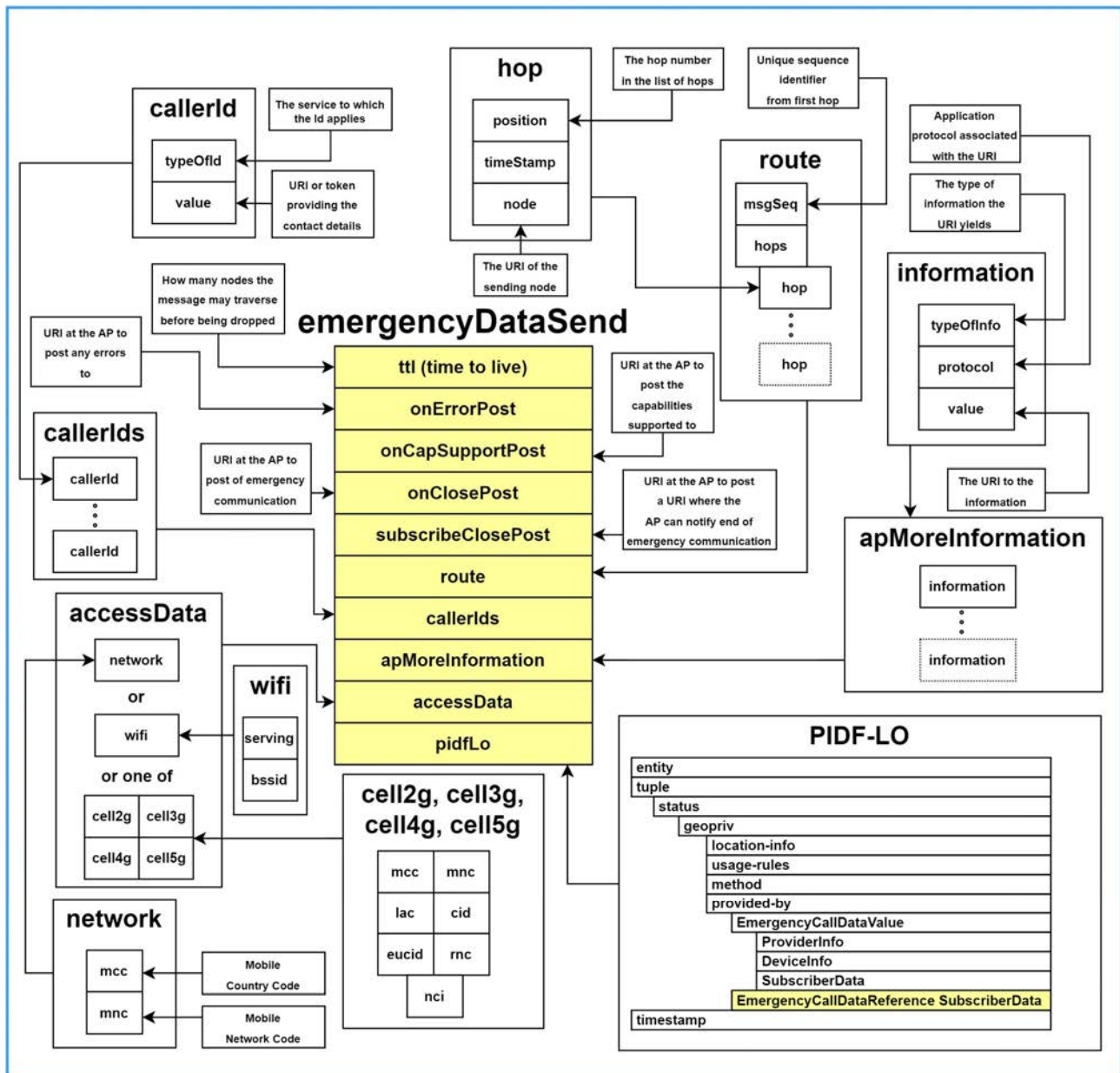
Figure 12: emergencyDataSend message structure
