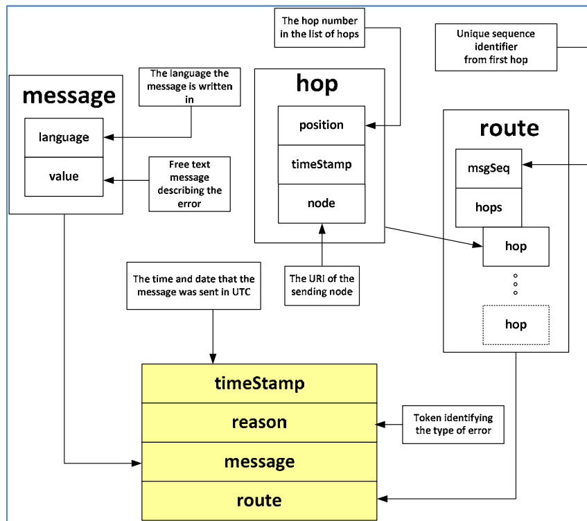
Figure 18: Error message structure
