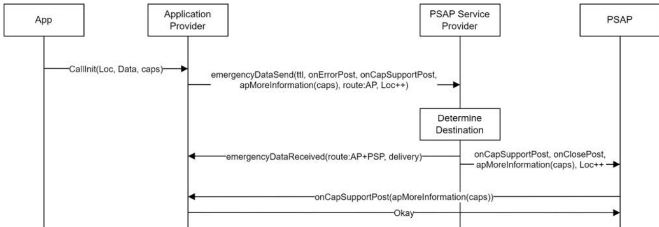
Figure 14: onCapSupportPost message sequence
