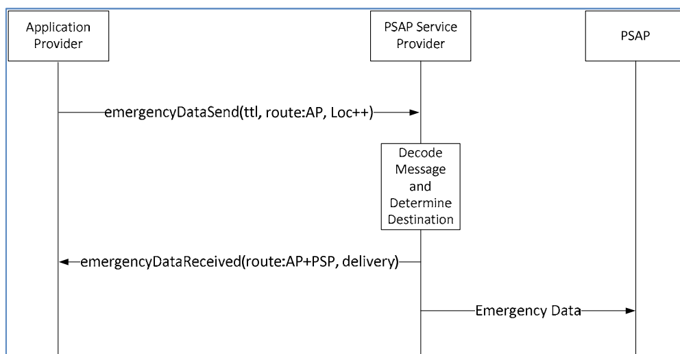
Figure 4: Ps basic message flow
