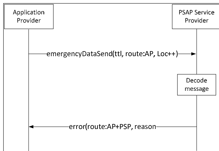
Figure 5: Ps error flow
