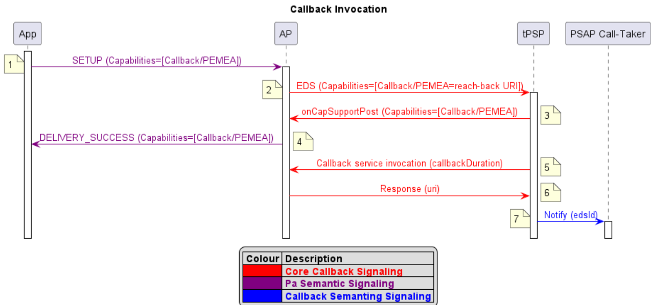
Figure 20: PEMA Callback service invocation sequence diagram
