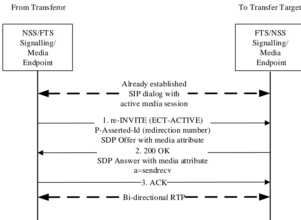
Figure 6.12: Transferor notifies transfer target about ECT-active event (target alerting)
