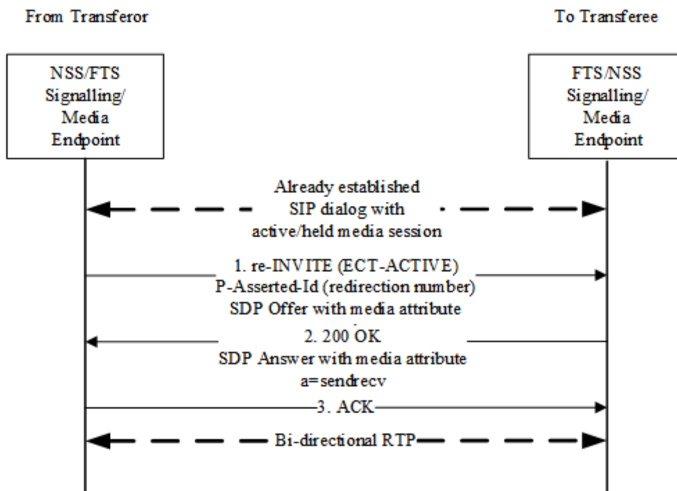
Figure 6.10: Transferor retrieves call to transferee (in case of ECT-alerting event)
