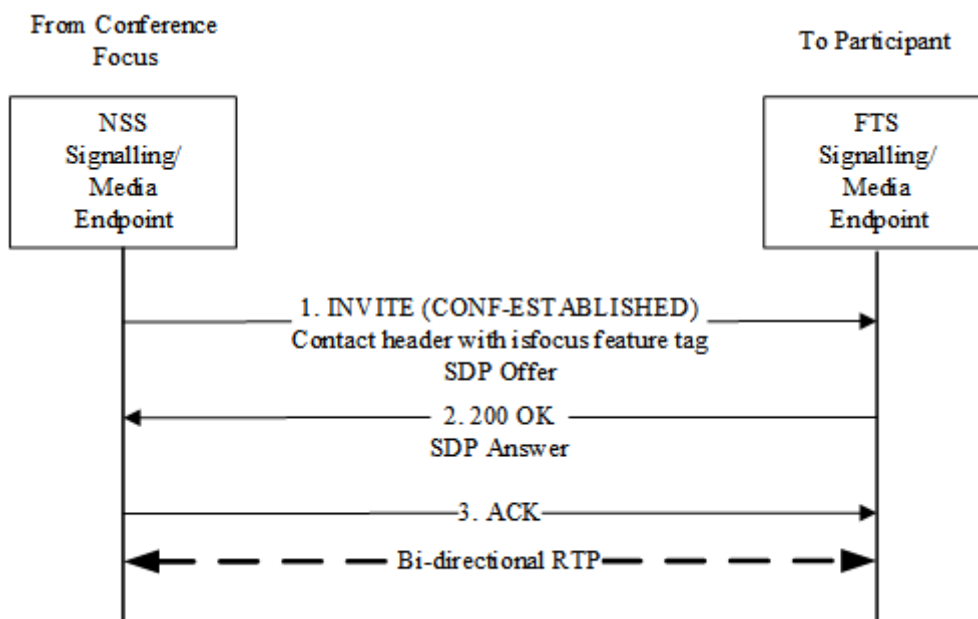
Figure 6.18: Point-to-point call is turned into conference call
