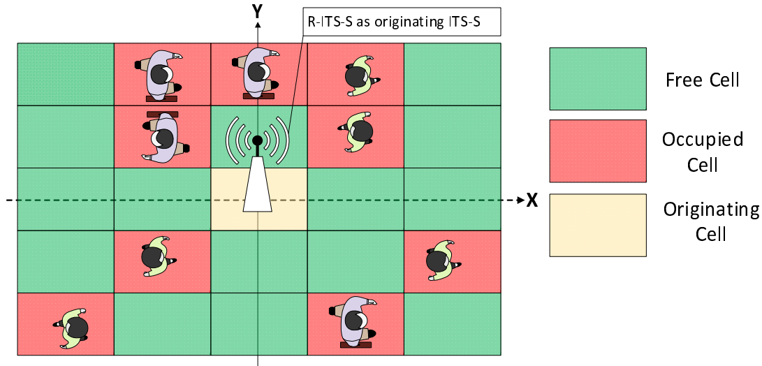
Figure I.1: Grid Occupancy Map concept shown for non-VRU ITS-S as the originating/ITS-S
