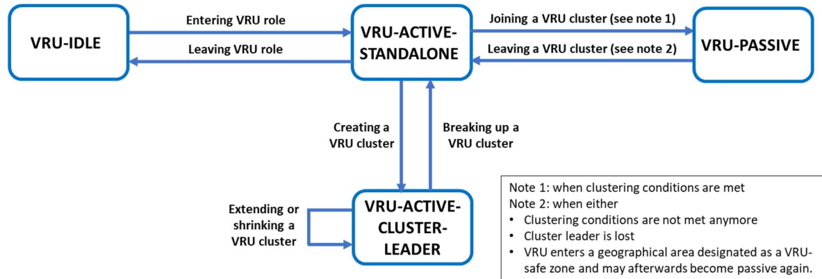
Figure 3: VBS state diagram related to VRU cluster operation
