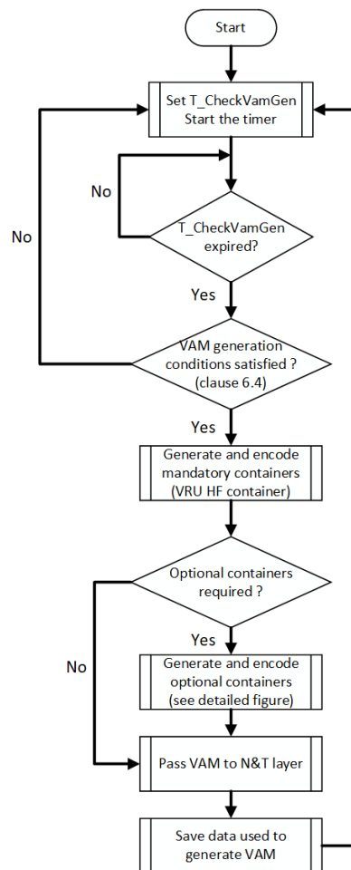
Figure C.1: VBS general protocol operation
