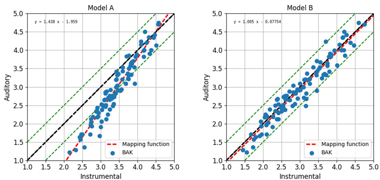
Figure 9.2: Prediction results for databases DES-25/-26 for N-MOS
