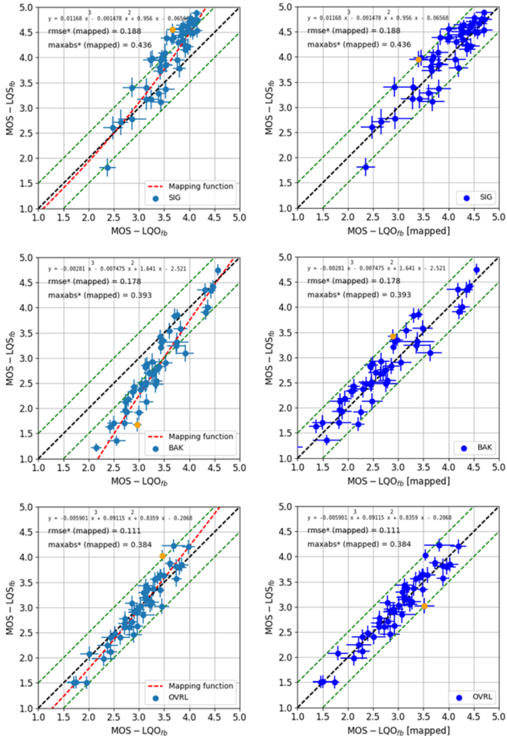
Figure 8.3: Scatter plots from model A for validation database 3
