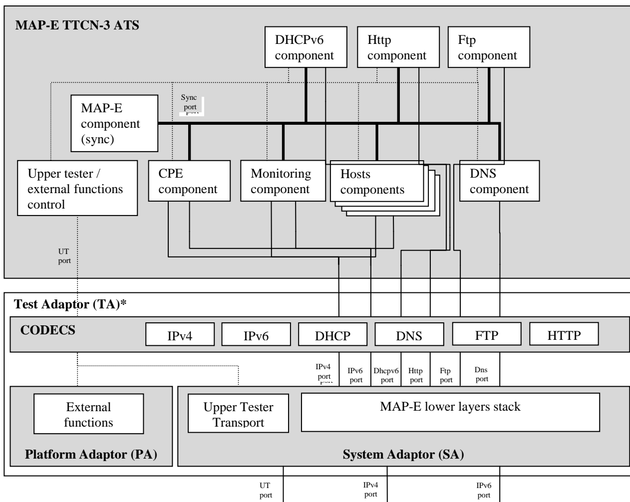
Figure 6: MAP-E TTCN-3 test architecture
