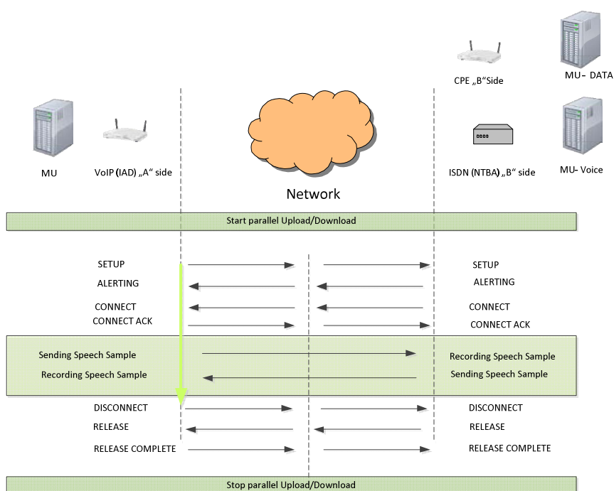
Figure 17: Measurement of voice quality with parallel data load
