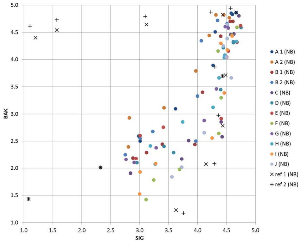
Figure 37: BAK vs SIG results, Tests 3 and 4
