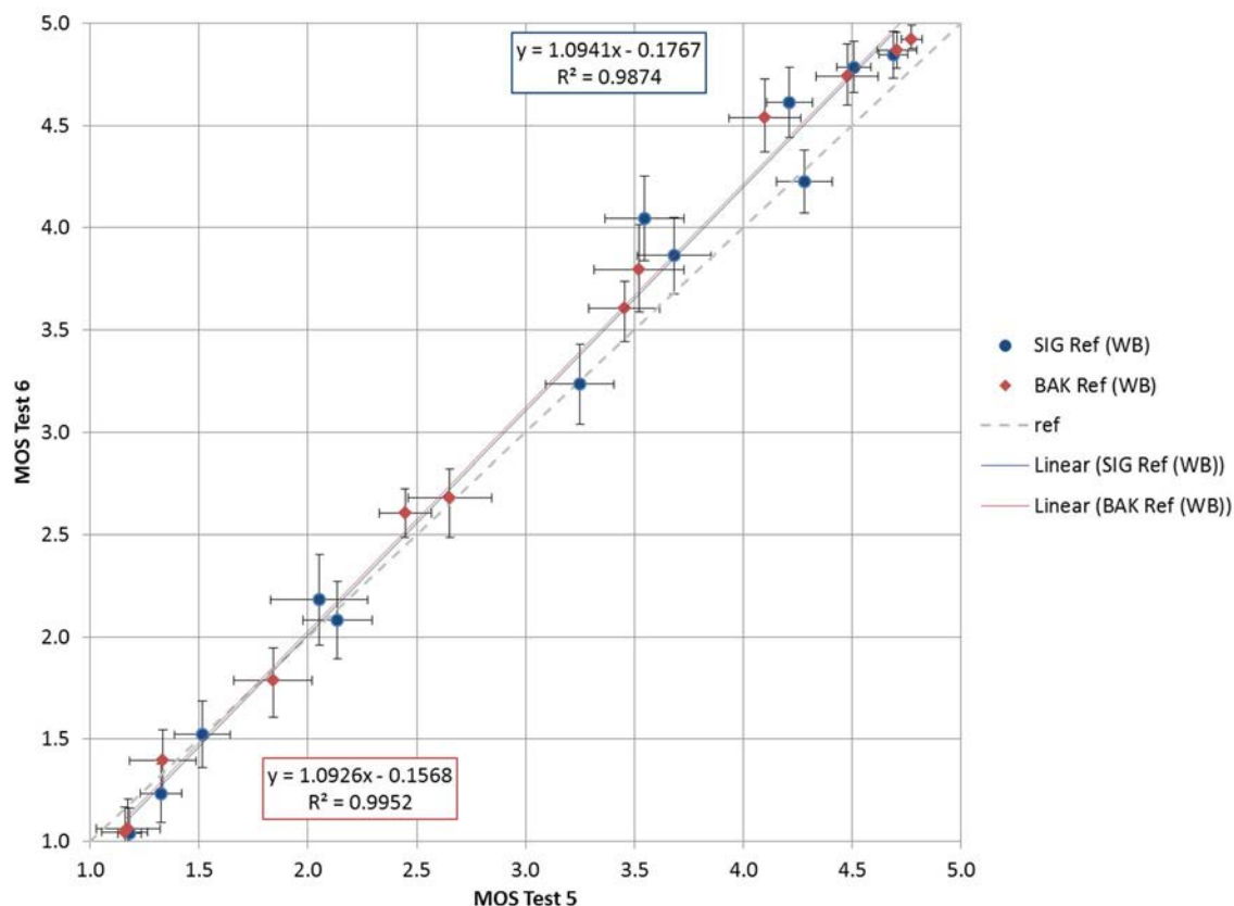
Figure 47: Scatterplot of SIG and BAK scores for reference conditions, Tests 5 and 6
