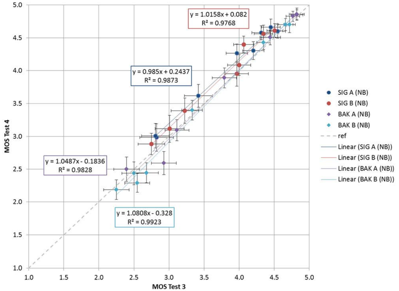
Figure 39: Scatterplot of SIG and BAK scores for devices A and B, Tests 3 and 4
