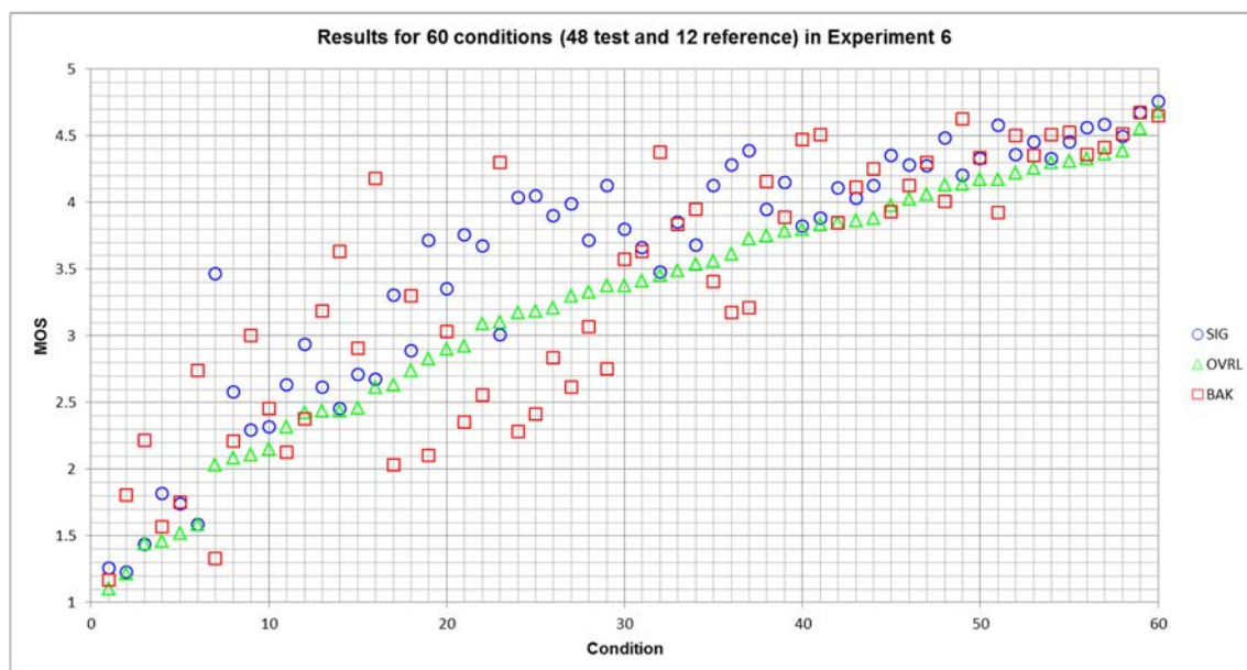
Figure 17: Results of Experiment 6
