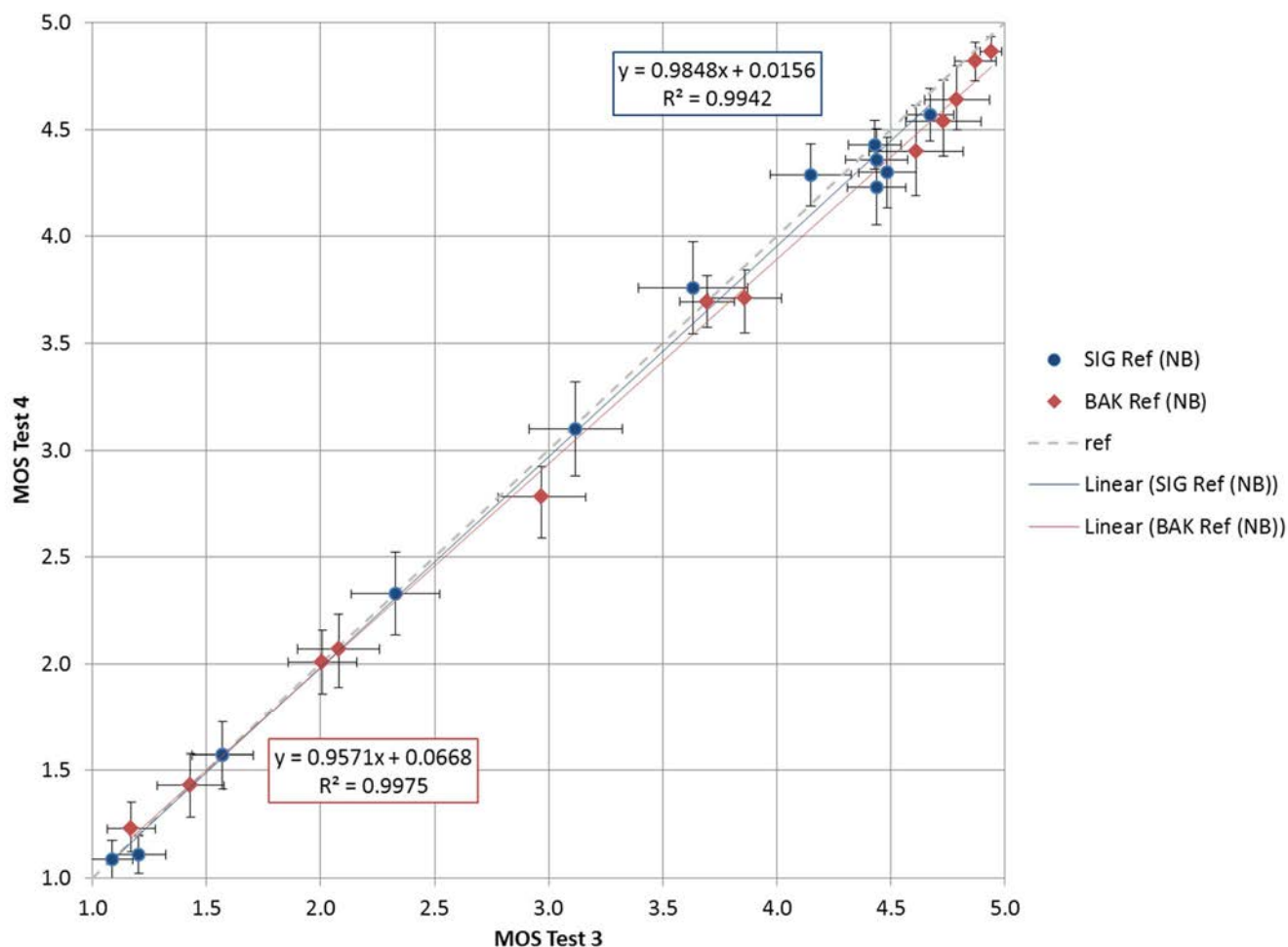
Figure 38: Scatterplot of SIG and BAK scores for reference conditions, Tests 3 and 4
