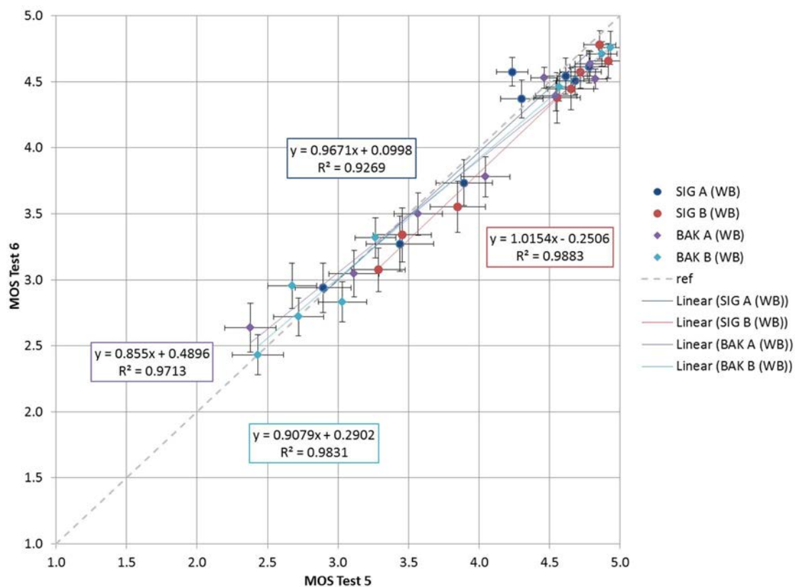
Figure 48: Scatterplot of SIG and BAK scores for devices A and B, Tests 5 and 6
